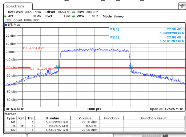
802.11ax20_5500MHz_RU_FULL_Ant 2
