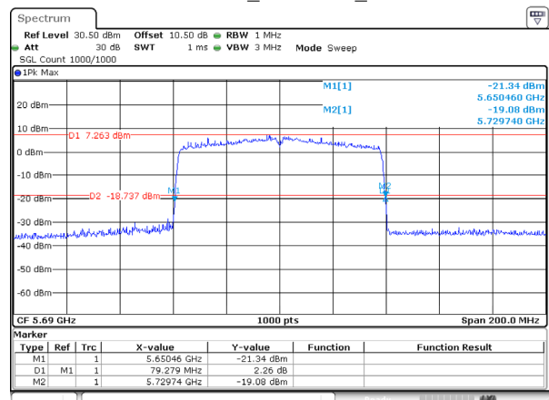
802.11ac80_5690MHz_Ant 2
