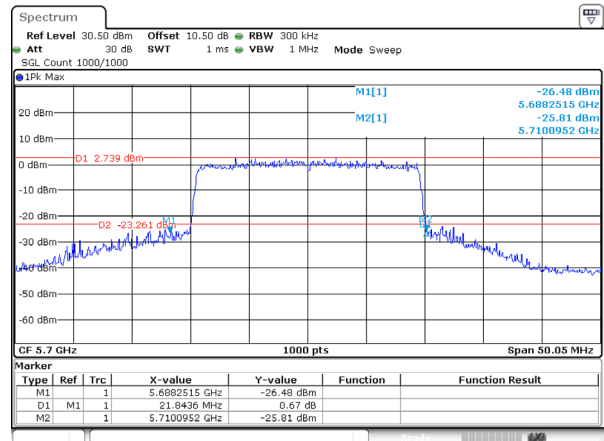
802.11ax20_5700MHz_RU_FULL_Ant 1
