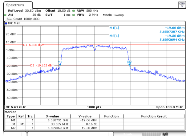
802.11ac40_5670MHz_Ant 2
