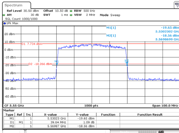
802.11be40_5550MHz_RU_FULL_Ant 1
