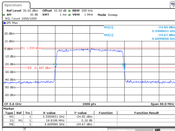
802.11ax20_5600MHz_RU_FULL_Ant 1
