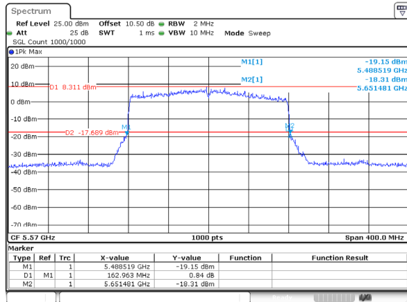
802.11ax160_5570MHz_RU_FULL_Ant 0
