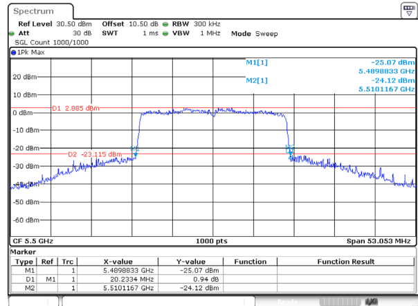
802.11ax20_5500MHz_RU_FULL_Ant 1
