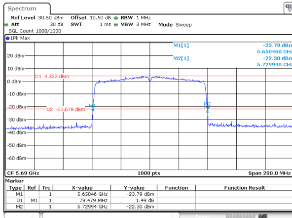
802.11ac80_5690MHz_Ant 1
