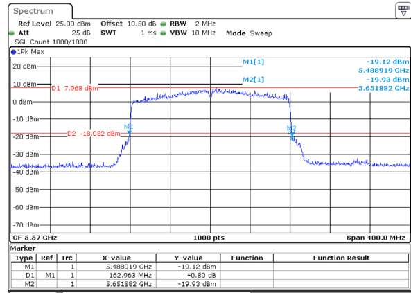
802.11ax160_5570MHz_RU_FULL_Ant 1
