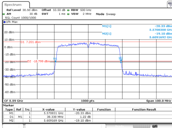
802.11ac40_5590MHz_Ant 2
