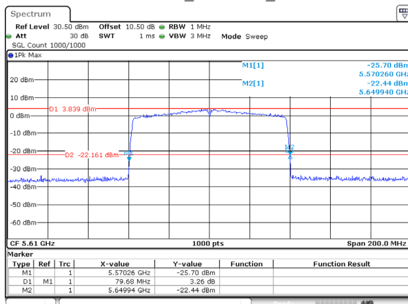
802.11ac80_5610MHz_Ant 0
