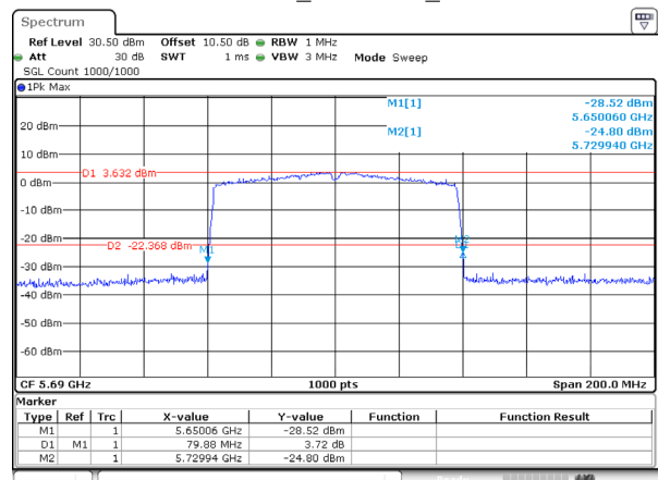
802.11ac80_5690MHz_Ant 0
