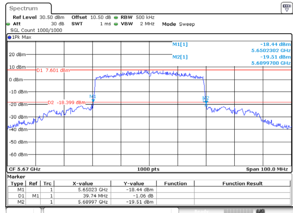
802.11be40_5670MHz_RU_FULL_Ant 1
