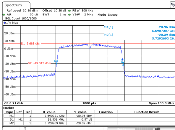
802.11ac40_5710MHz_Ant 2
