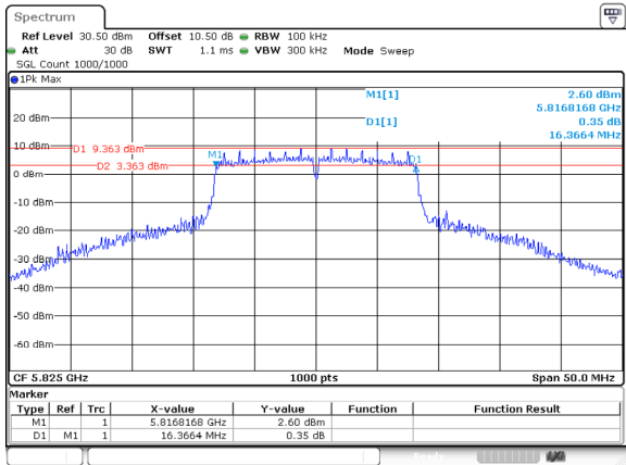
802.11a_5825MHz_Ant 0
