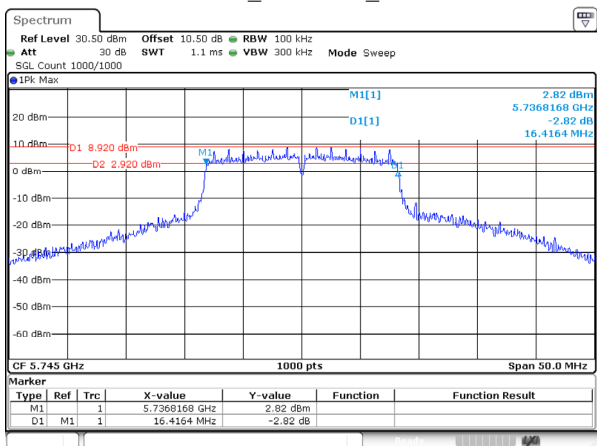
802.11a_5745MHz_Ant 2
