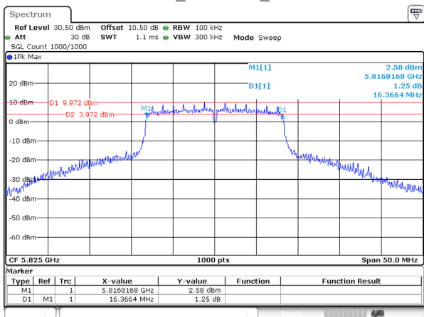
802.11a_5825MHz_Ant 1
