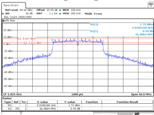
802.11a_5825MHz_Ant 2
