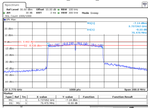
802.11ac80_5775MHz_Ant 2
