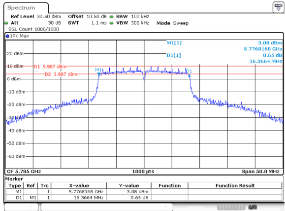
802.11a_5785MHz_Ant 0
