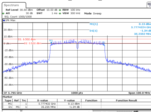
802.11ac40_5795MHz_Ant 0
