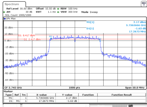
802.11ac20_5745MHz_Ant 1
