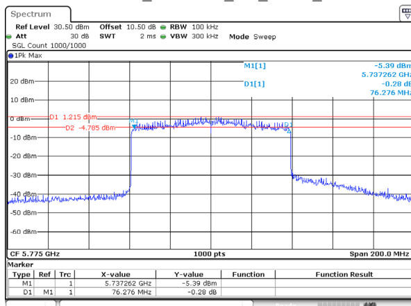
802.11ax80_5775MHz_RU_FULL_Ant 1
