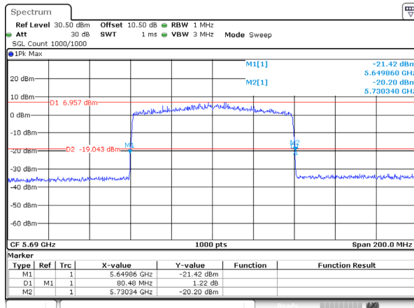
802.11be80_5690MHz_RU_FULL_Ant 1
