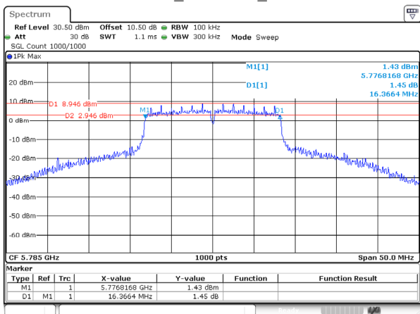
802.11a_5785MHz_Ant 2
