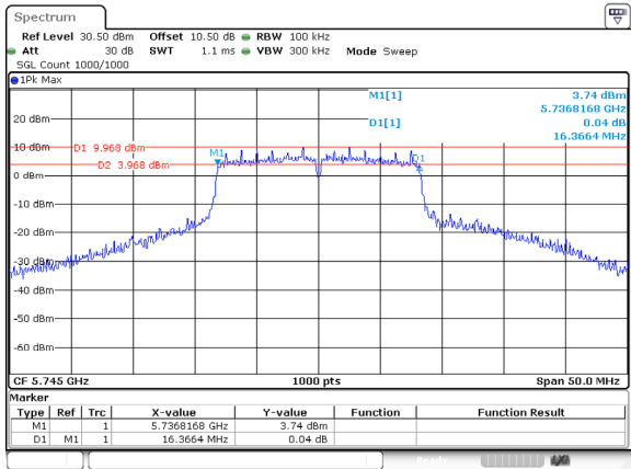
802.11a_5745MHz_Ant 0
