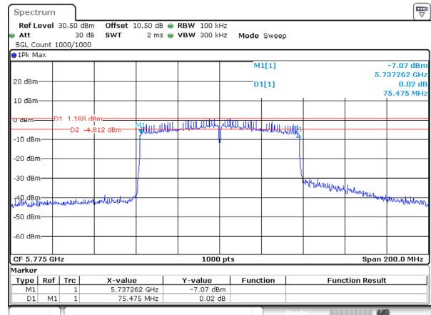
802.11ac80_5775MHz_Ant 0
