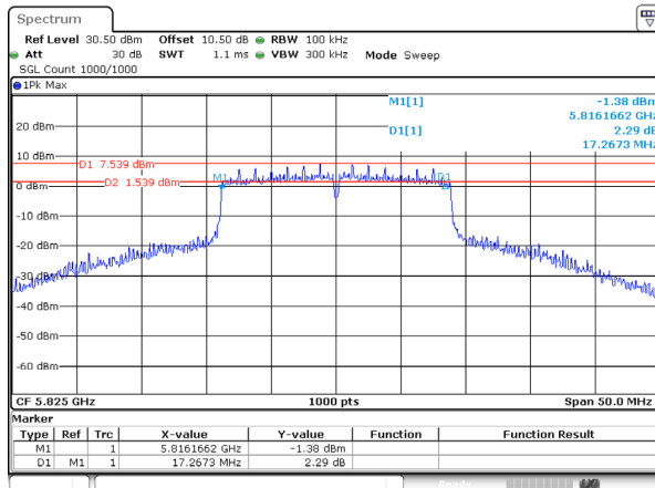
802.11ac20_5825MHz_Ant 2
