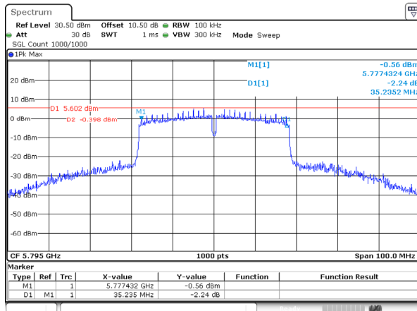
802.11ac40_5795MHz_Ant 2
