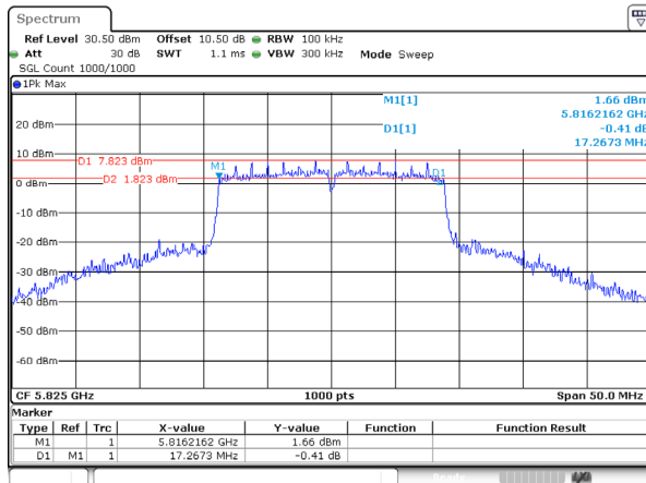
802.11ac20_5825MHz_Ant 0
