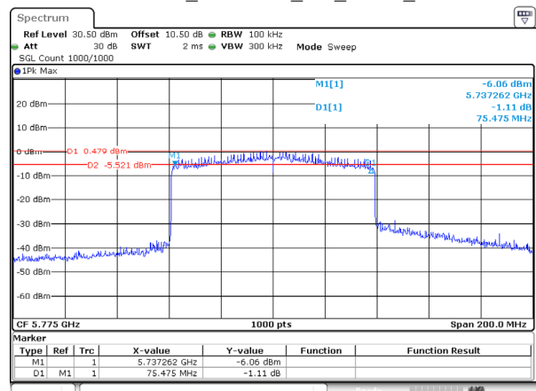
802.11ax80_5775MHz_RU_FULL_Ant 2
