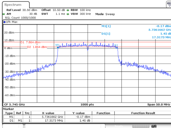
802.11ac20_5745MHz_Ant 2
