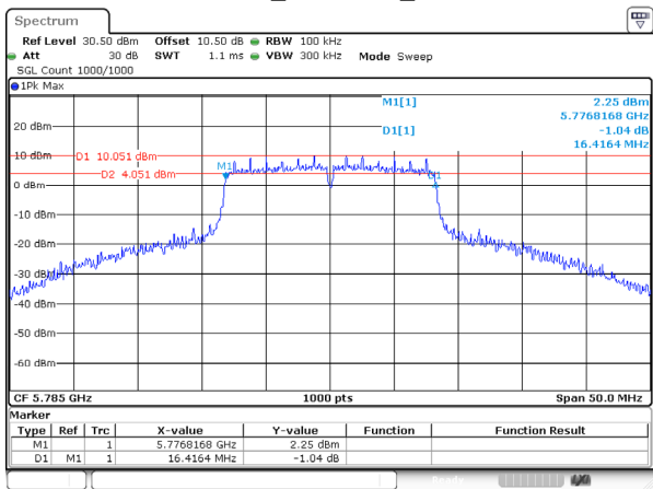
802.11a_5785MHz_Ant 1
