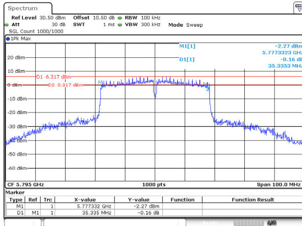
802.11ac40_5795MHz_Ant 1
