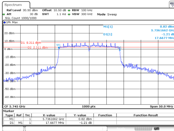
802.11ac20_5745MHz_Ant 0
