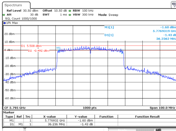
802.11ax40_5795MHz_RU_FULL_Ant 2
