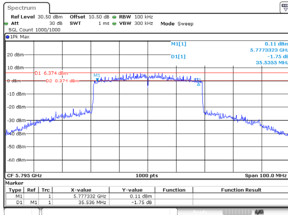
802.11ax40_5795MHz_RU_FULL_Ant 1
