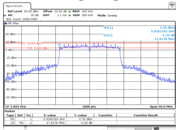
802.11ac20_5825MHz_Ant 1
