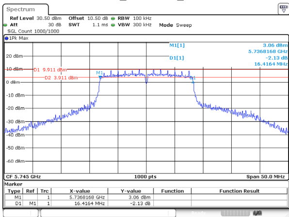
802.11a_5745MHz_Ant 1
