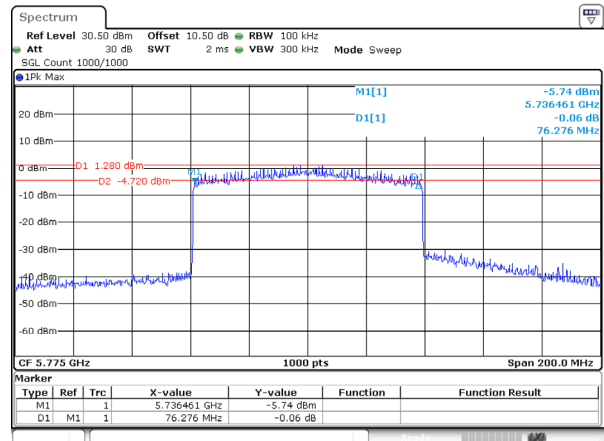
802.11ax80_5775MHz_RU_FULL_Ant 0
