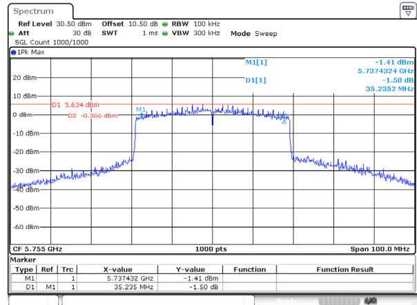
802.11ax40_5755MHz_RU_FULL_Ant 2
