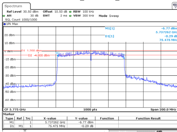
802.11ac80_5775MHz_Ant 1
