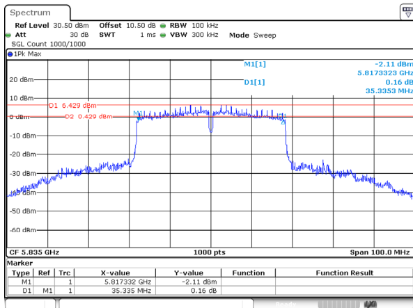
802.11ac40_5835MHz_Ant 1
