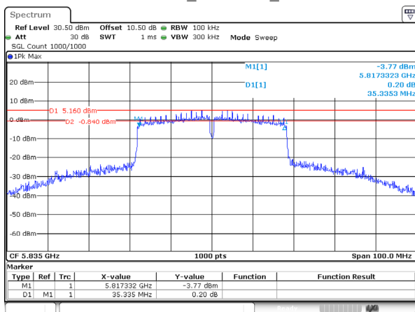
802.11ac40_5835MHz_Ant 2
