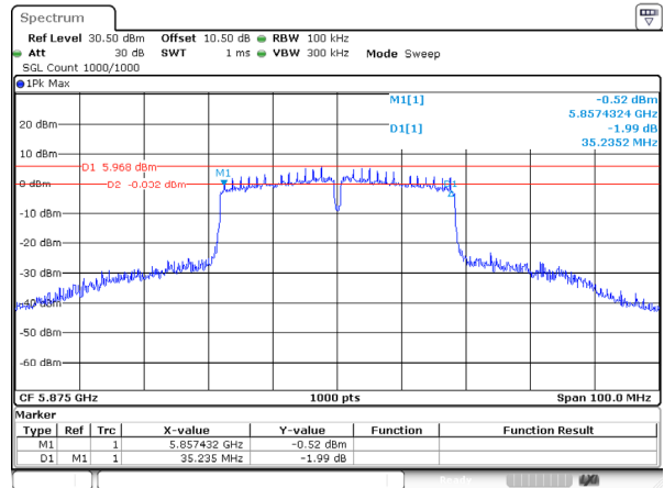
802.11ac40_5875MHz_Ant 0
