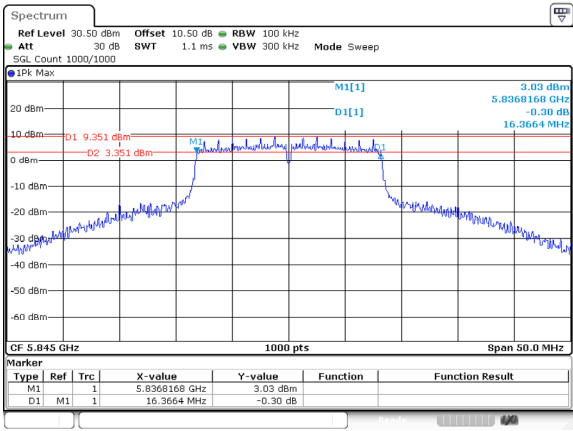
802.11a_5845MHz_Ant 0
