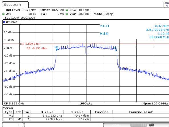
802.11ac40_5835MHz_Ant 0
