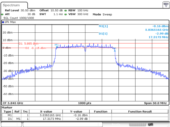
802.11ac20_5845MHz_Ant 2
