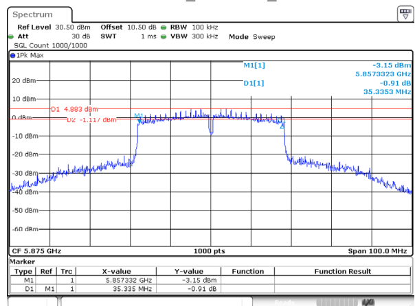
802.11ac40_5875MHz_Ant 2
