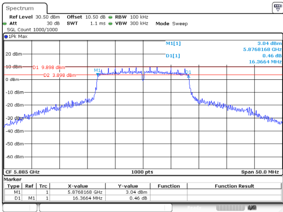
802.11a_5885MHz_Ant 1
