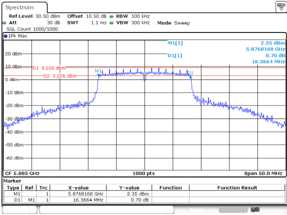
802.11a_5885MHz_Ant 0
