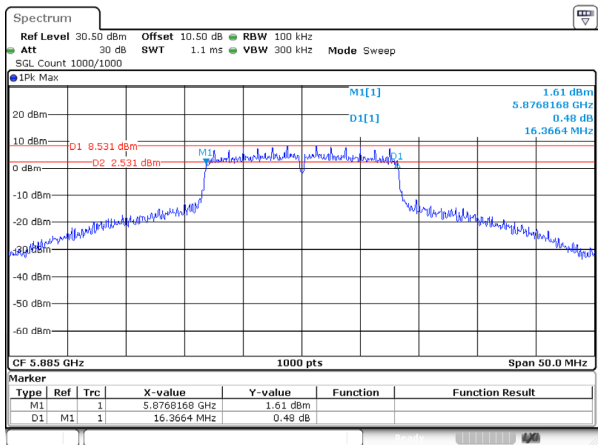
802.11a_5885MHz_Ant 2
