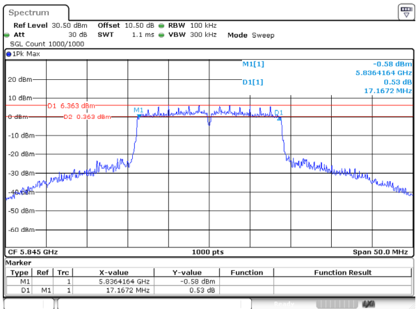
802.11ac20_5845MHz_Ant 0
