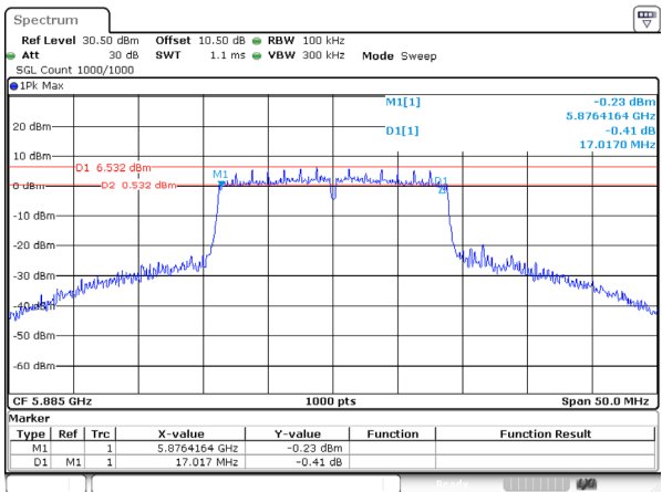
802.11ac20_5885MHz_Ant 0
