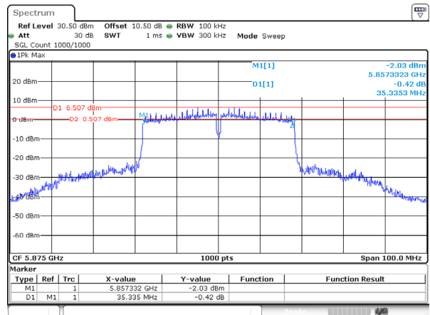
802.11ac40_5875MHz_Ant 1
