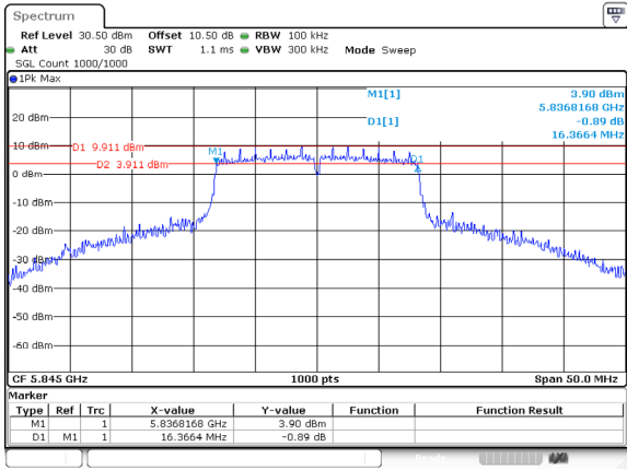
802.11a_5845MHz_Ant 1
