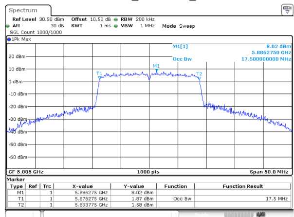
802.11ac20_5885MHz_Ant 0
