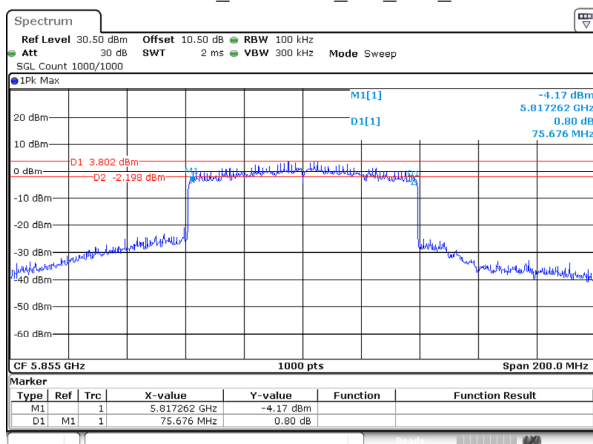
802.11ax80_5855MHz_RU_Full_Ant 1
