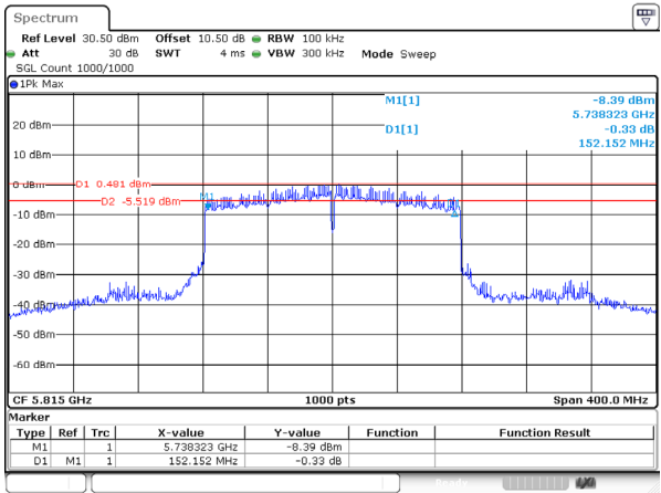
802.11ax160_5815MHz_RU_FULL_Ant 1
