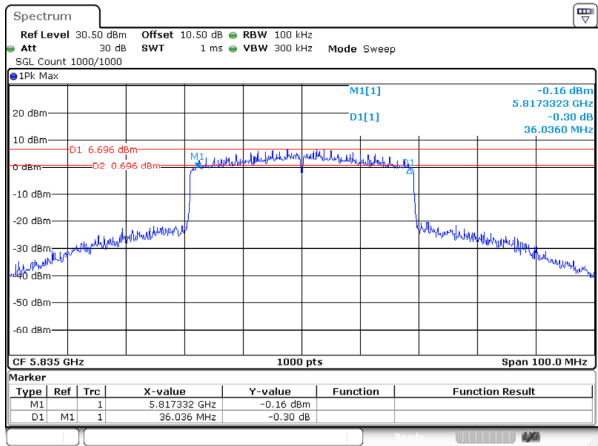
802.11be40_5835MHz_RU_Full_Ant 0
