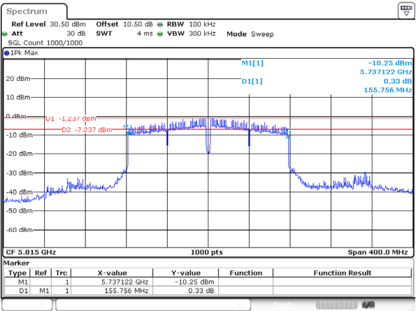
802.11ac160_5815MHz_RU_FULL_Ant 2
