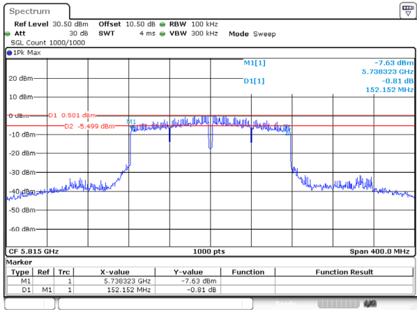
802.11ac160_5815MHz_RU_FULL_Ant 1
