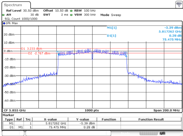
802.11ac80_5855MHz_Ant 0
