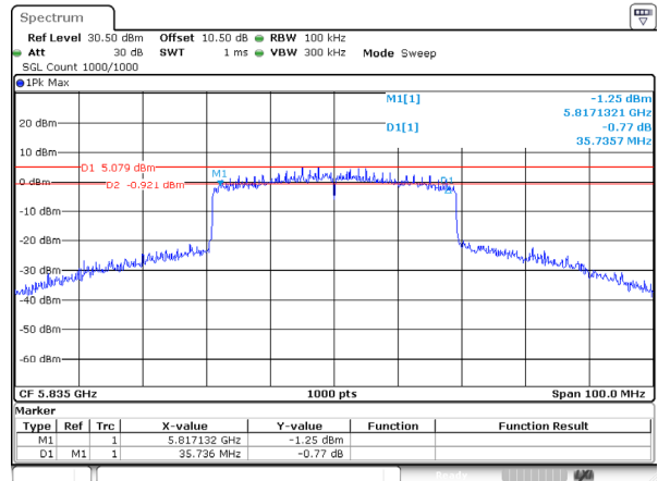
802.11ax40_5835MHz_RU_Full_Ant 2
