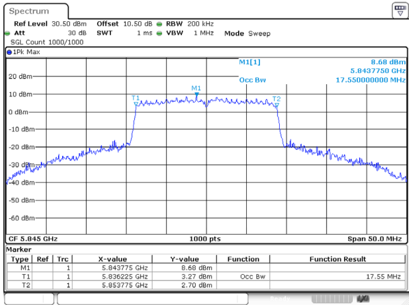
802.11ac20_5845MHz_Ant 1
