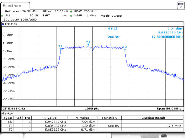
802.11ac20_5845MHz_Ant 2
