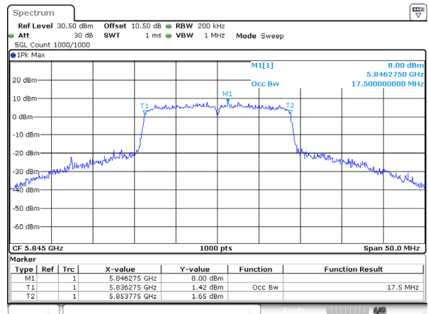
802.11ac20_5845MHz_Ant 0
