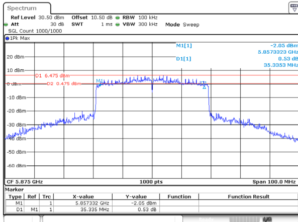
802.11ax40_5875MHz_RU_Full_Ant 1
