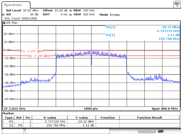
802.11ax160_5815MHz_RU_FULL_Ant 2
