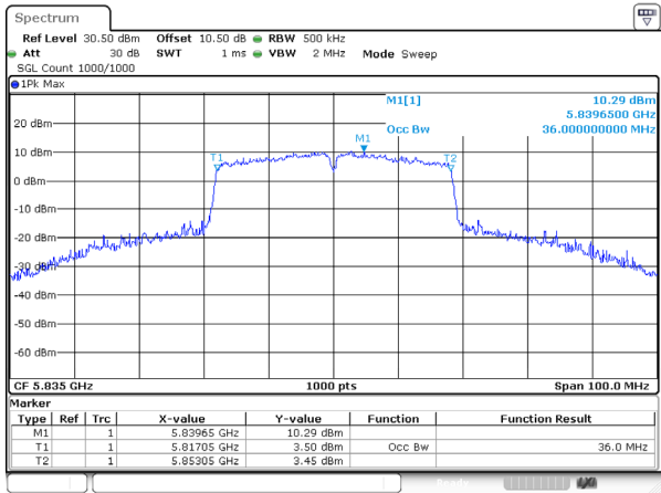
802.11ac40_5835MHz_Ant 0
