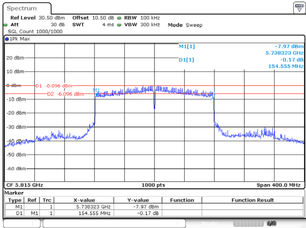
802.11ax160_5815MHz_RU_FULL_Ant 0
