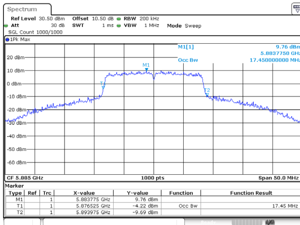
802.11a_5885MHz_Ant 2
