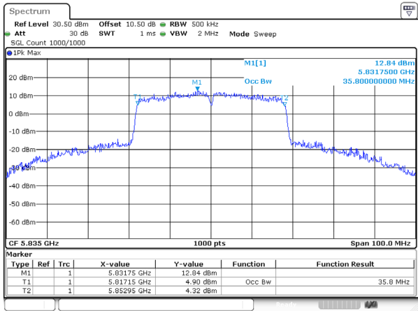
802.11ac40_5835MHz_Ant 1
