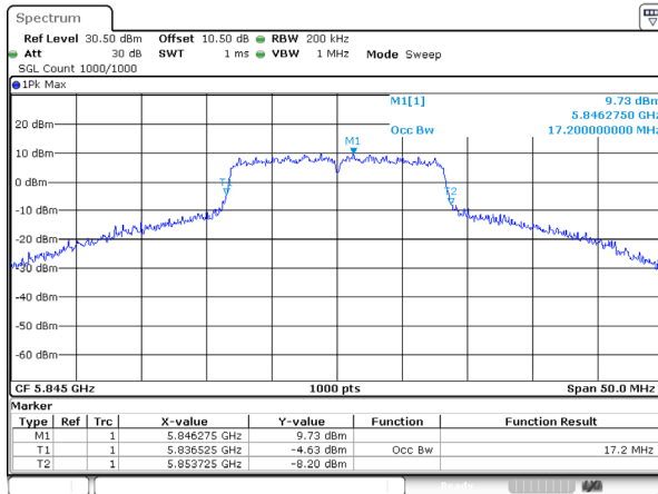
802.11a_5845MHz_Ant 2
