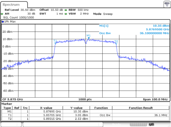
802.11ac40_5875MHz_Ant 2
