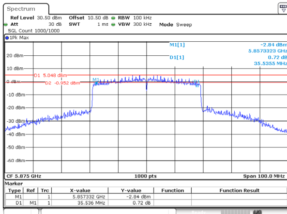
802.11ax40_5875MHz_RU_Full_Ant 2
