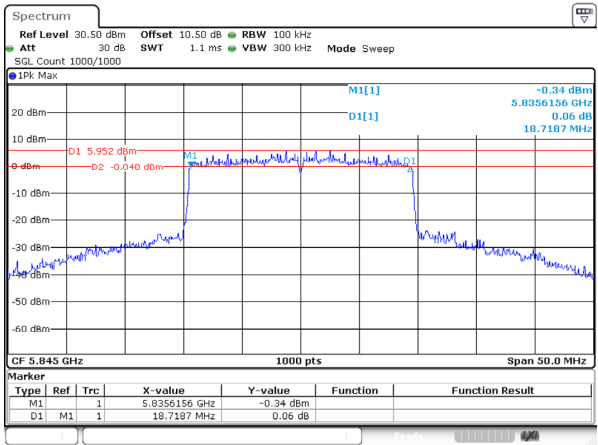
802.11be20_5845MHz_RU_Full_Ant 0
