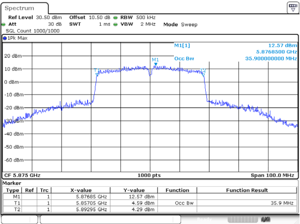
802.11ac40_5875MHz_Ant 1
