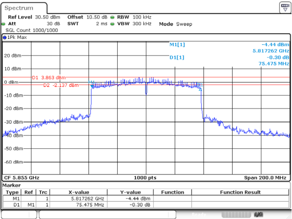
802.11ac80_5855MHz_Ant 1
