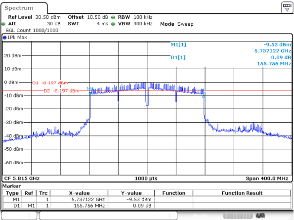
802.11ac160_5815MHz_RU_FULL_Ant 0
