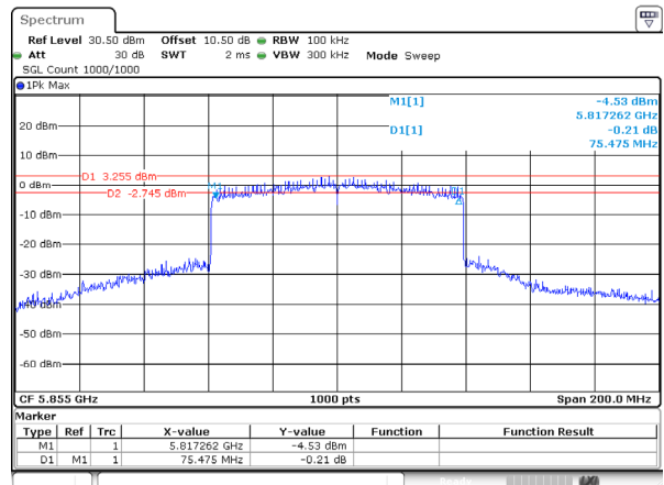
802.11ax80_5855MHz_RU_Full_Ant 0
