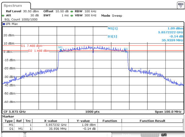
802.11be40_5875MHz_RU_Full_Ant 1
