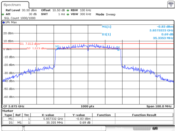
802.11be40_5875MHz_RU_Full_Ant 0
