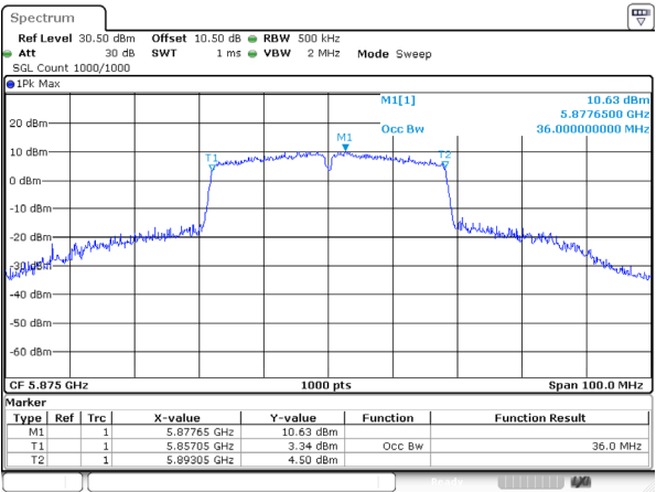
802.11ac40_5875MHz_Ant 0
