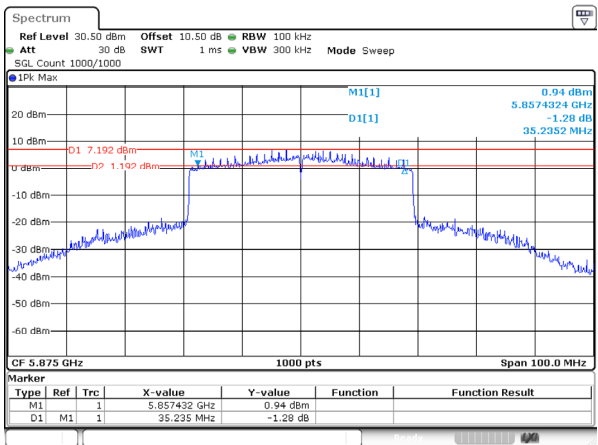
802.11be40_5875MHz_RU_Full_Ant 2
