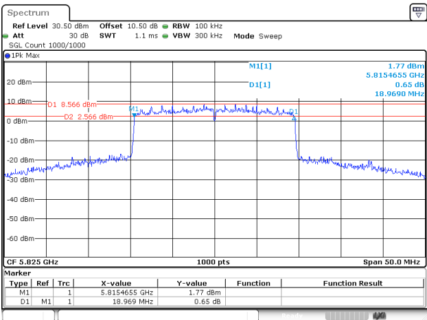
802.11be20_5825MHz_RU_Full_Chain 1
