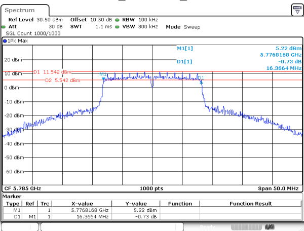
802.11a_5785MHz_Chain 0
