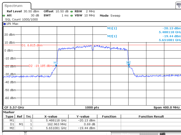
802.11ac160_5570MHz_RU_FULL_Chain 1
