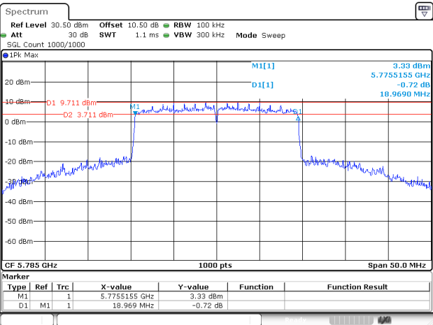
802.11be20_5785MHz_RU_Full_Chain 1
