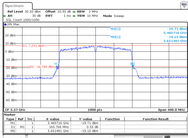
802.11ac160_5570MHz_RU_FULL_Chain 2
