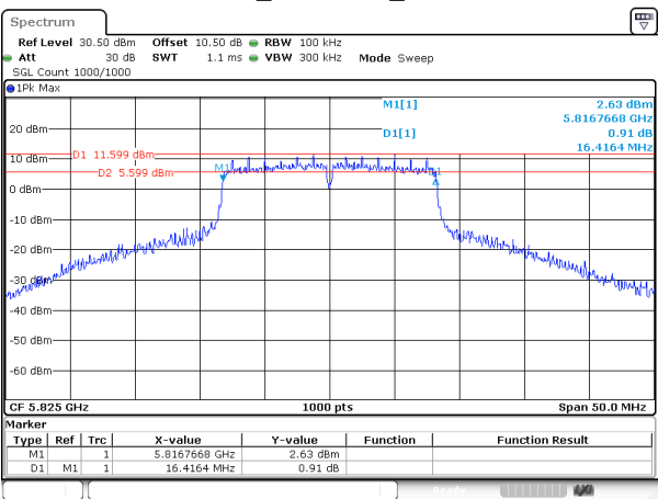
802.11a_5825MHz_Chain 1
