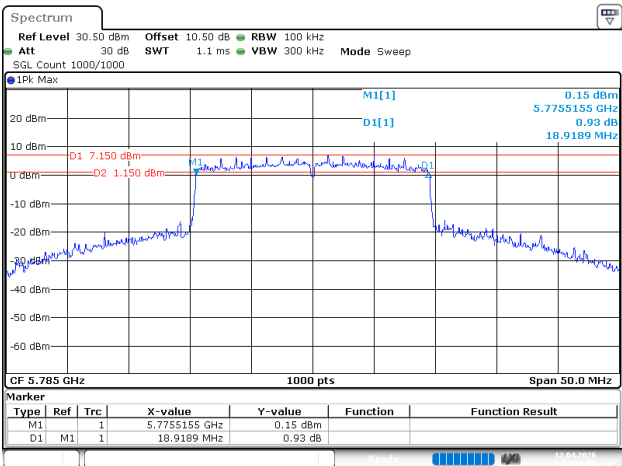
802.11be20_5785MHz_RU_Full_Chain 2
