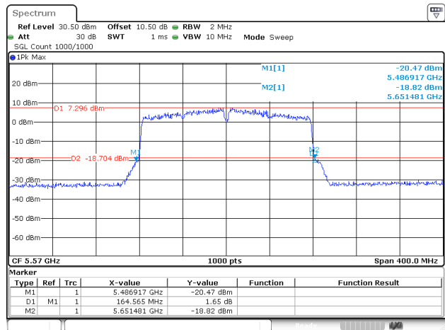
802.11ac160_5570MHz_RU_FULL_Chain 0
