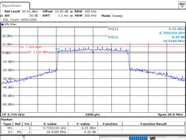
802.11be20_5745MHz_RU_Full_Chain 2
