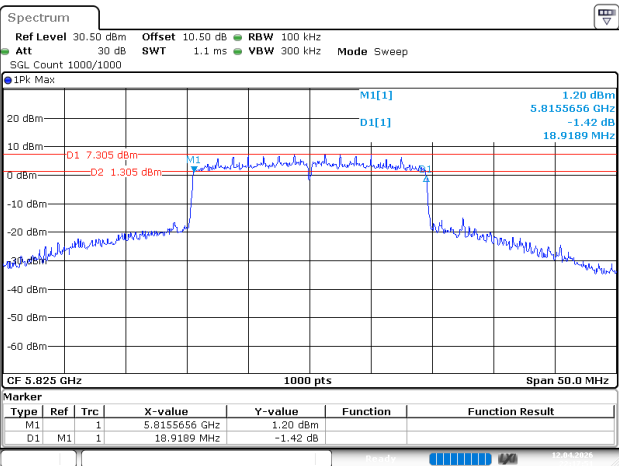
802.11be20_5825MHz_RU_Full_Chain 2
