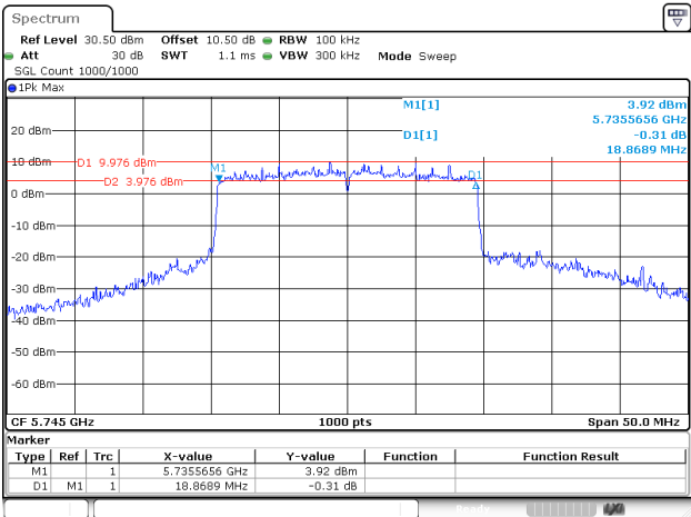
802.11be20_5745MHz_RU_Full_Chain 1
