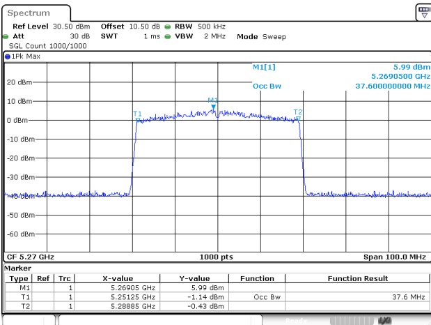
802.11be40_5270MHz_RU_Full_Chain 1
