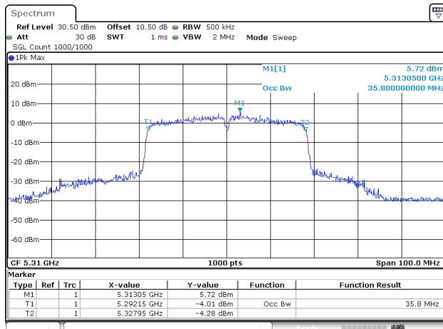
802.11ac40_5310MHz_Chain 1
