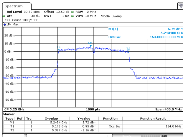
802.11ac160_5250MHz_RU_FULL_Chain 2
