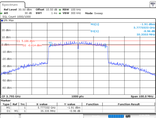
802.11be40_5795MHz_RU_Full_Chain 0
