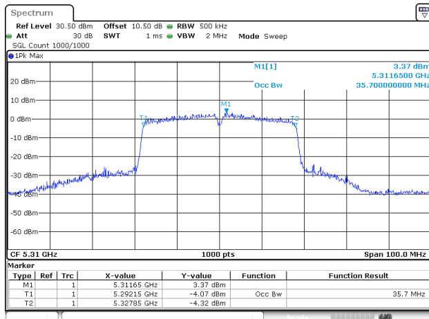
802.11ac40_5310MHz_Chain 2
