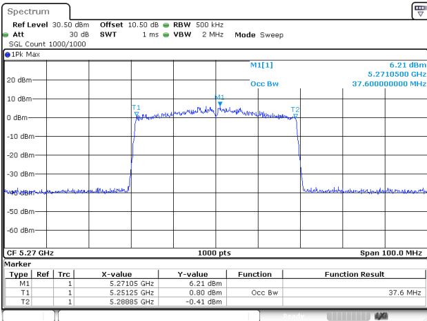
802.11be40_5270MHz_RU_Full_Chain 0
