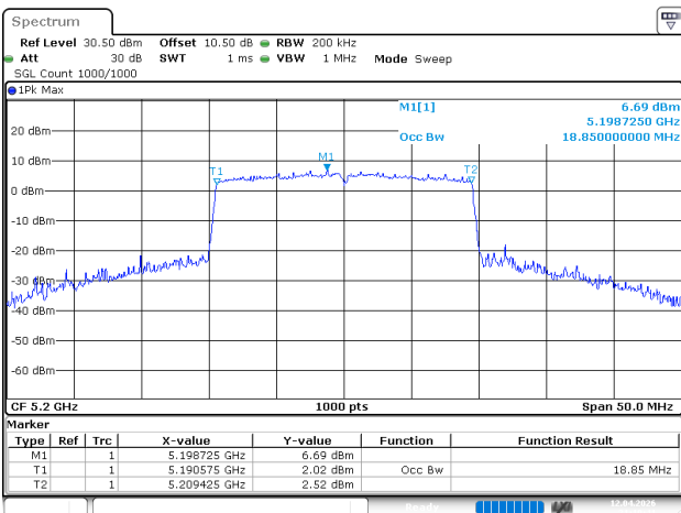
802.11be20_5200MHz_RU_Full_Chain 0
