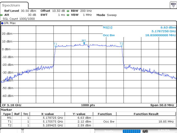
802.11be20_5180MHz_RU_Full_Chain 0
