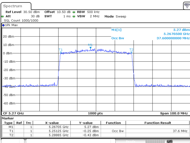
802.11be40_5270MHz_RU_Full_Chain 2
