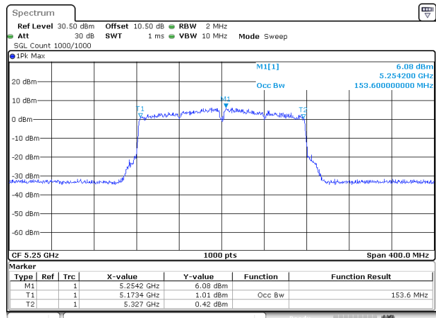
802.11ac160_5250MHz_RU_FULL_Chain 1
