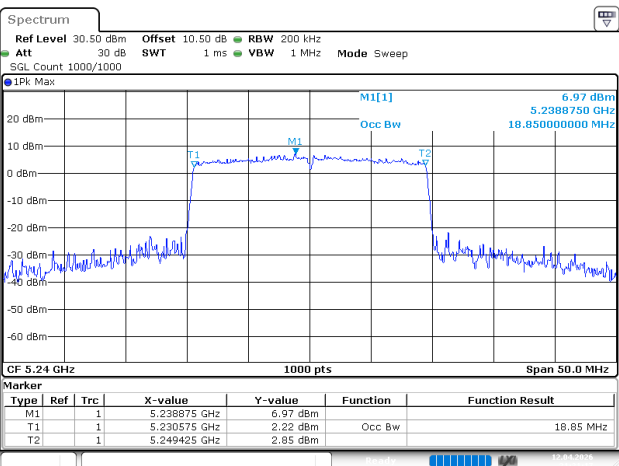
802.11be20_5240MHz_RU_Full_Chain 0
