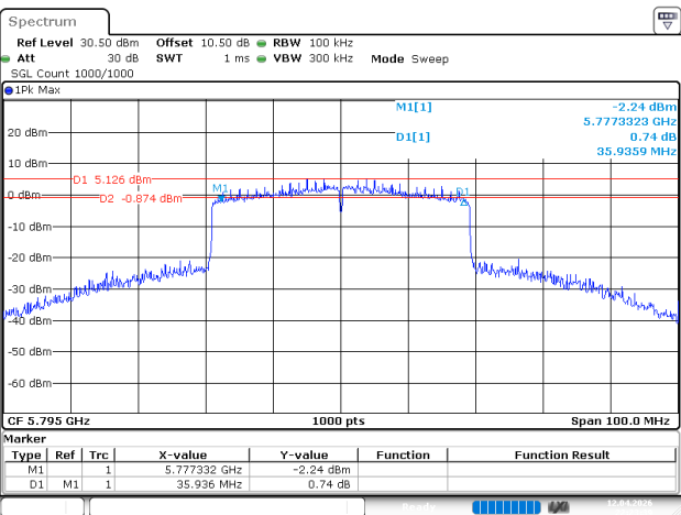
802.11be40_5795MHz_RU_Full_Chain 2
