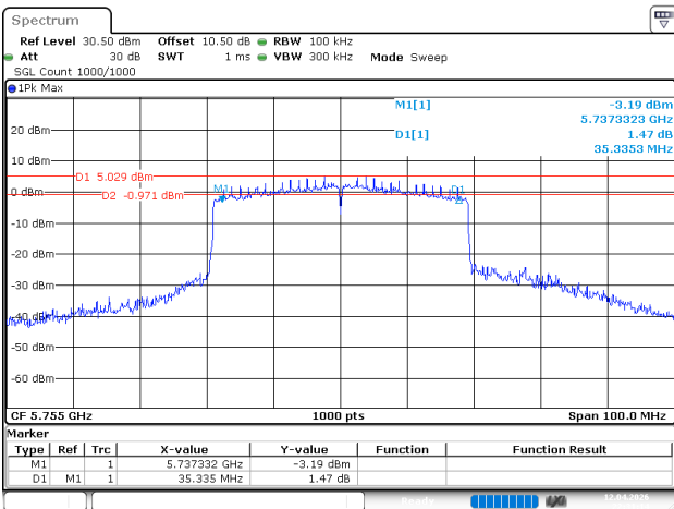
802.11be40_5755MHz_RU_Full_Chain 0
