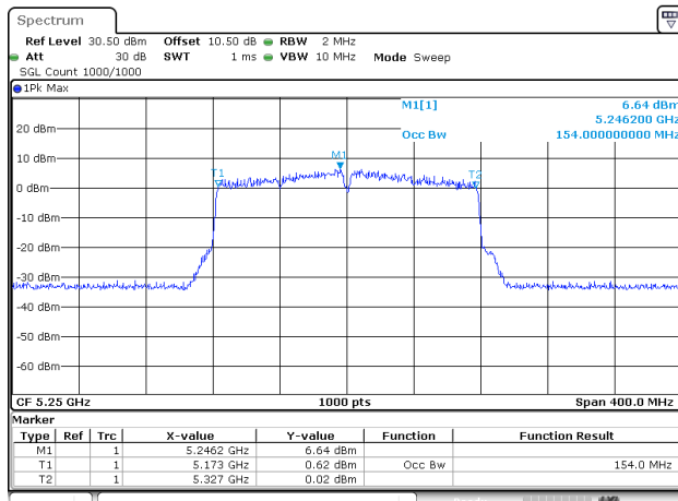
802.11ac160_5250MHz_RU_FULL_Chain 0
