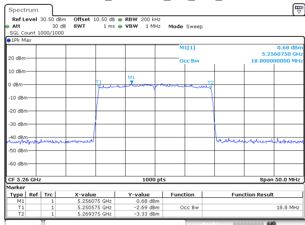
802.11be20_5260MHz_RU_Full_Chain 0
