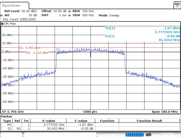
802.11be40_5795MHz_RU_Full_Chain 1
