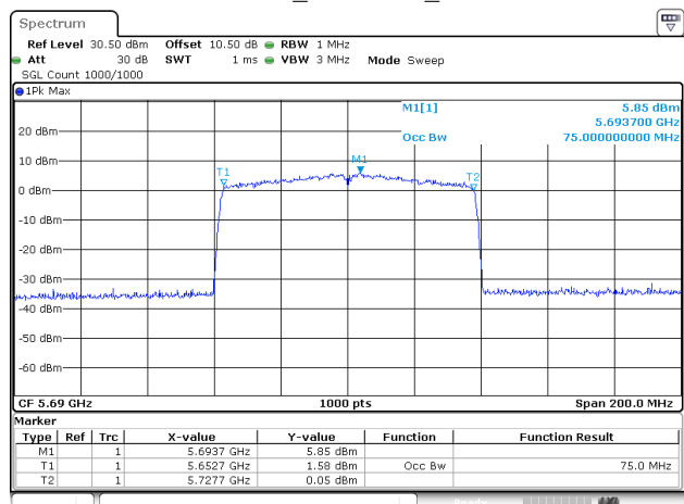
802.11ac80_5690MHz_Chain 1
