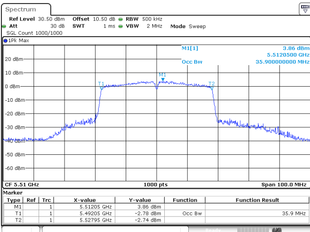
802.11ac40_5510MHz_Chain 0
