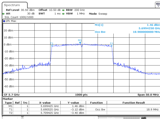
802.11be20_5700MHz_RU_Full_Chain 2
