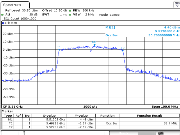
802.11ac40_5510MHz_Chain 2
