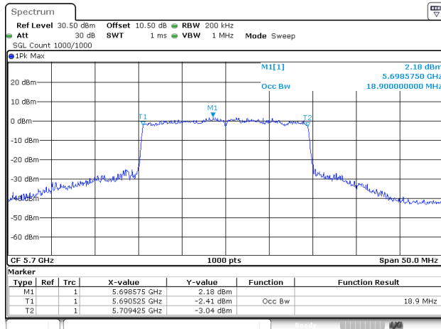
802.11be20_5700MHz_RU_Full_Chain 1
