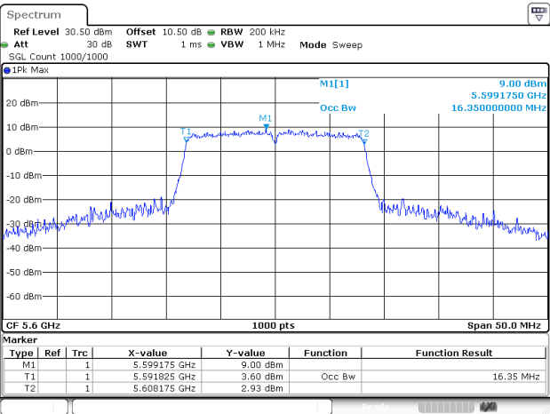
802.11a_5600MHz_Chain 2
