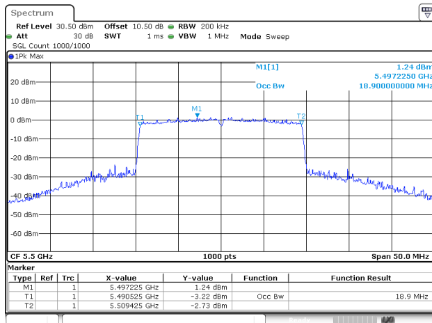
802.11be20_5500MHz_RU_Full_Chain 2
