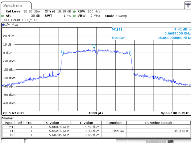
802.11ac40_5670MHz_Chain 2
