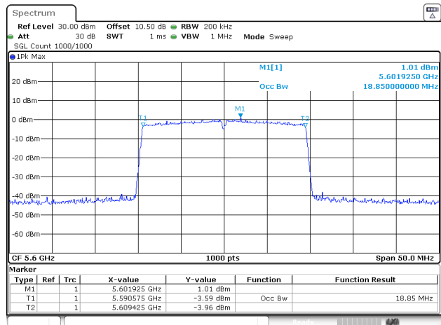
802.11be20_5600MHz_RU_Full_Chain 2
