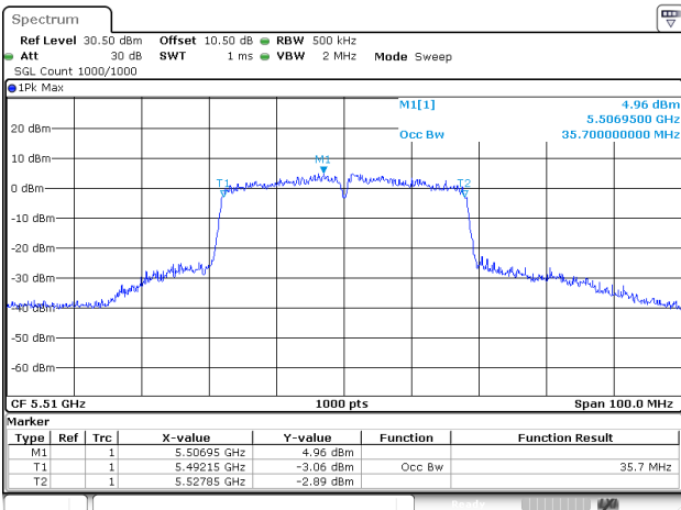
802.11ac40_5510MHz_Chain 1
