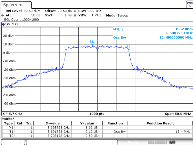
802.11a_5700MHz_Chain 2
