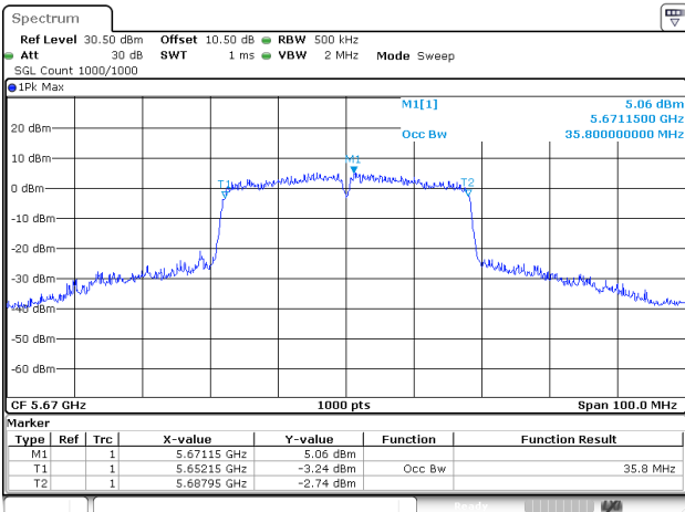
802.11ac40_5670MHz_Chain 1
