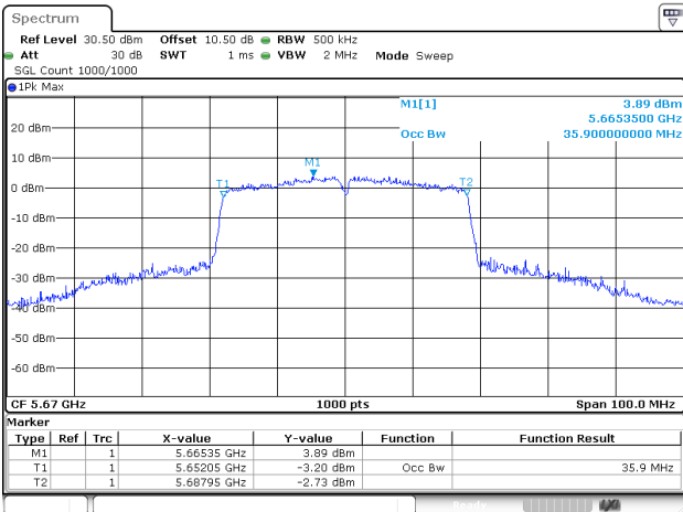
802.11ac40_5670MHz_Chain 0
