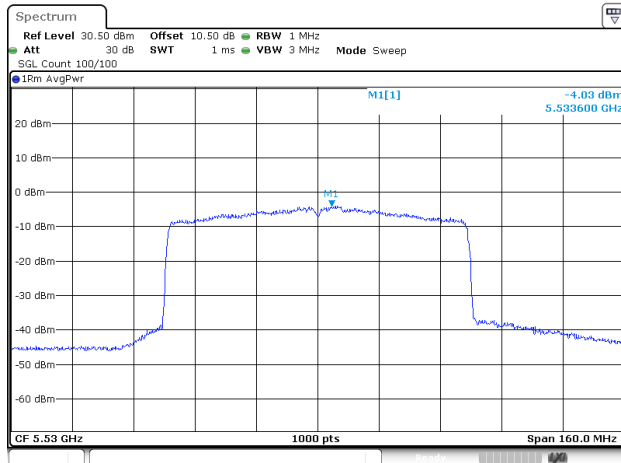
802.11be80_5530MHz_RU_Full_Chain 2
