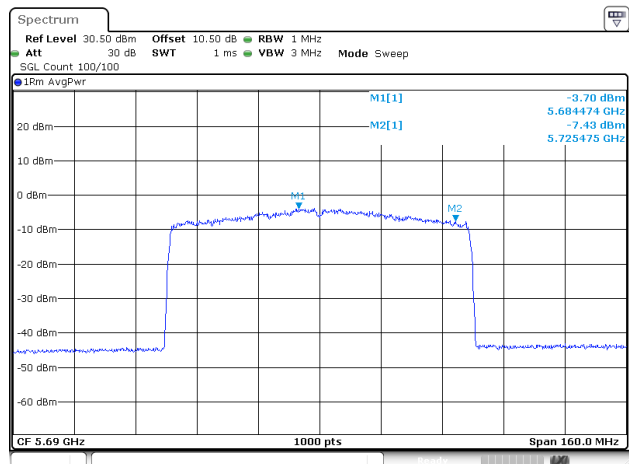
802.11be80_5690MHz_RU_Full_Chain 1
