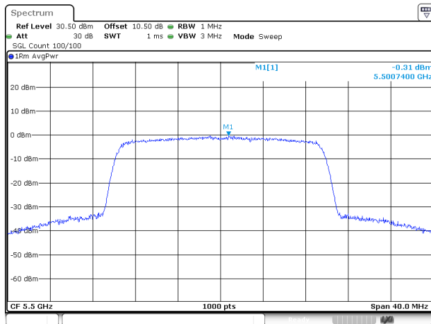
802.11be20_5500MHz_RU_Full_Chain 2
