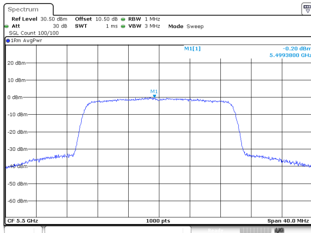
802.11be20_5500MHz_RU_Full_Chain 0
