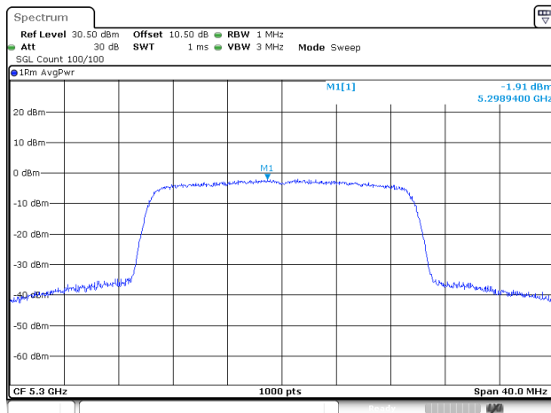
802.11be20_5300MHz_RU_Full_Chain 2
