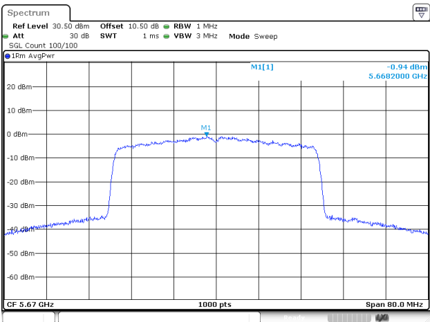
802.11be40_5670MHz_RU_Full_Chain 0
