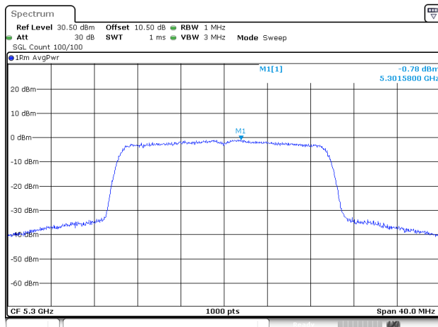
802.11be20_5300MHz_RU_Full_Chain 0
