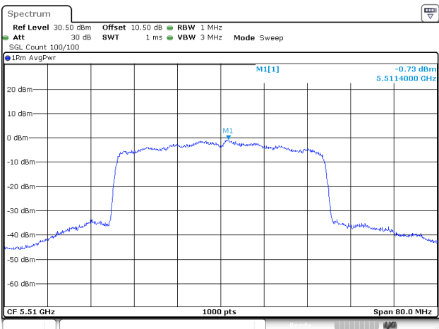
802.11be40_5510MHz_RU_Full_Chain 1
