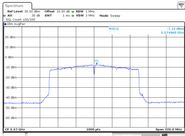
802.11be160_5570MHz_RU_FULL_Chain 2
