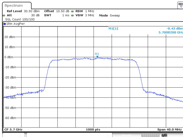
802.11be20_5700MHz_RU_Full_Chain 0
