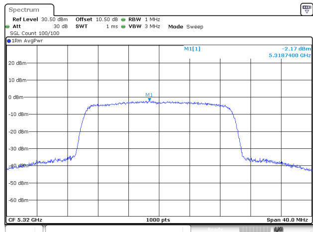
802.11be20_5320MHz_RU_Full_Chain 2
