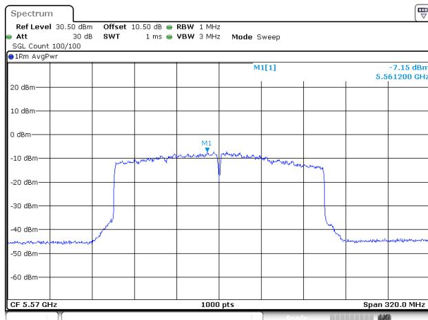
802.11be160_5570MHz_RU_FULL_Chain 1
