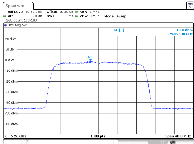
802.11be20_5260MHz_RU_Full_Chain 2
