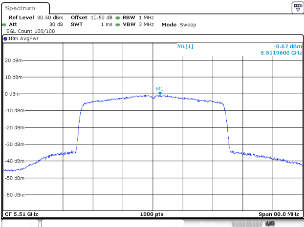
802.11be40_5510MHz_RU_Full_Chain 0
