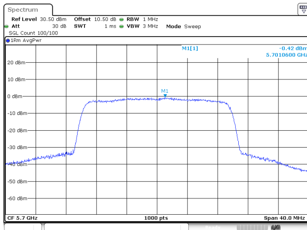
802.11be20_5700MHz_RU_Full_Chain 2
