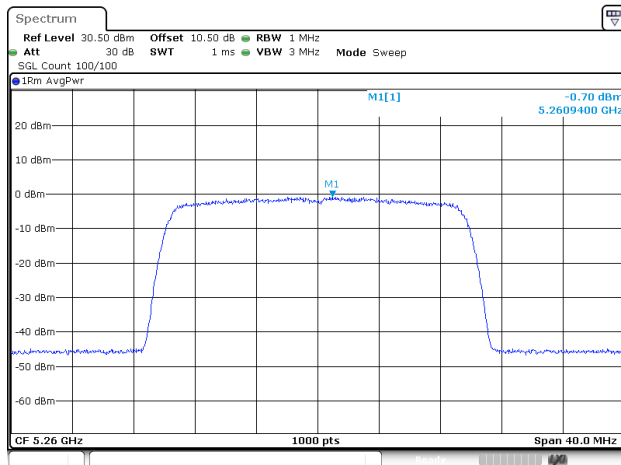
802.11be20_5260MHz_RU_Full_Chain 1
