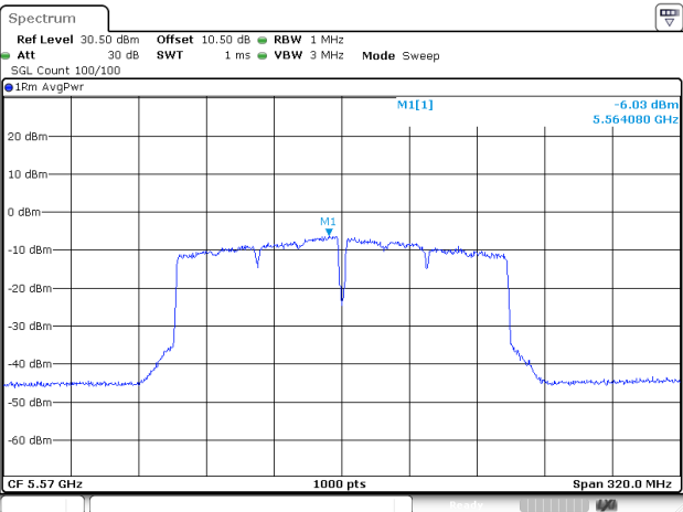
802.11ac160_5570MHz_RU_FULL_Chain 0
