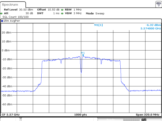
802.11ac160_5570MHz_RU_FULL_Chain 2
