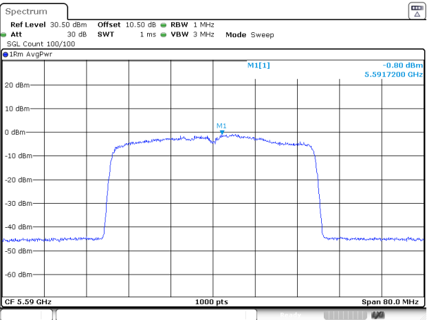
802.11be40_5590MHz_RU_Full_Chain 0
