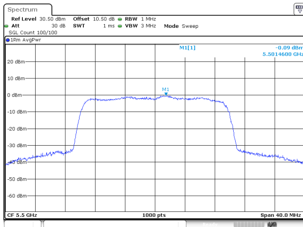
802.11be20_5500MHz_RU_Full_Chain 1
