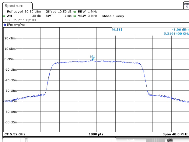
802.11be20_5320MHz_RU_Full_Chain 1
