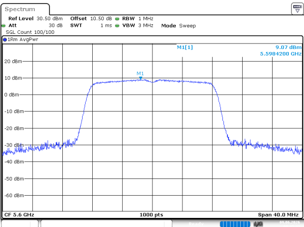
802.11a_5600MHz_Chain 0
