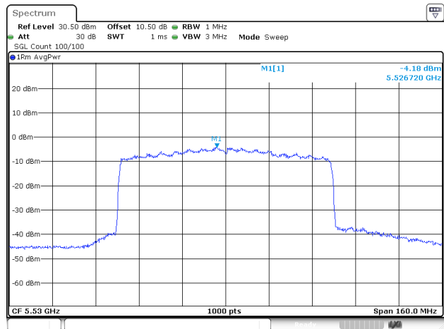
802.11be80_5530MHz_RU_Full_Chain 1
