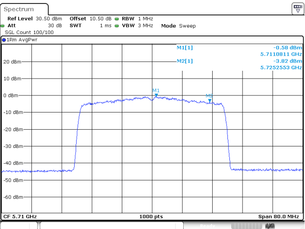
802.11be40_5710MHz_RU_Full_Chain 0
