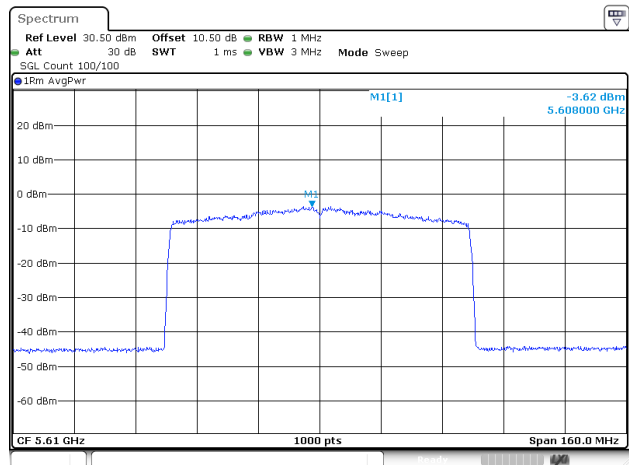
802.11be80_5610MHz_RU_Full_Chain 0
