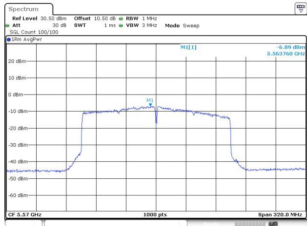
802.11be160_5570MHz_RU_FULL_Chain 0
