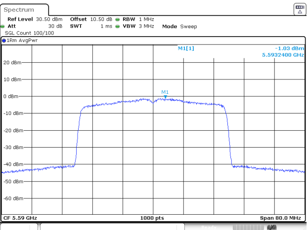
802.11be40_5590MHz_RU_Full_Chain 1
