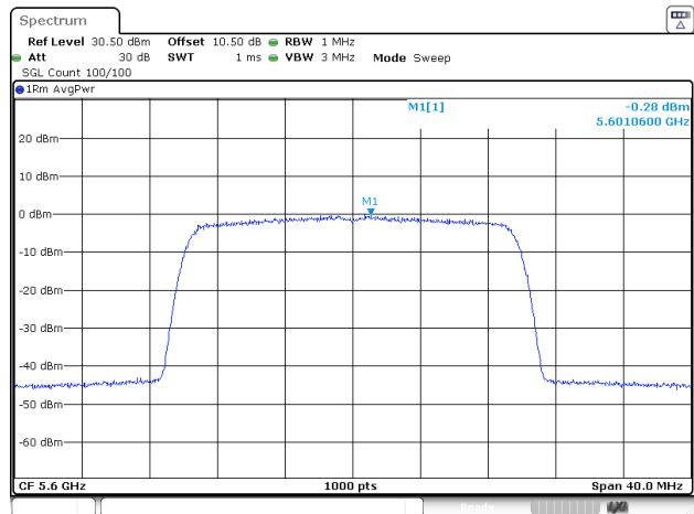
802.11be20_5600MHz_RU_Full_Chain 2
