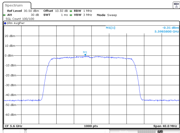
802.11be20_5600MHz_RU_Full_Chain 0
