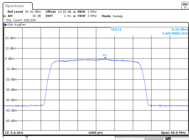
802.11be20_5600MHz_RU_Full_Chain 1
