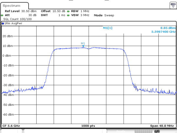
802.11a_5600MHz_Chain 1
