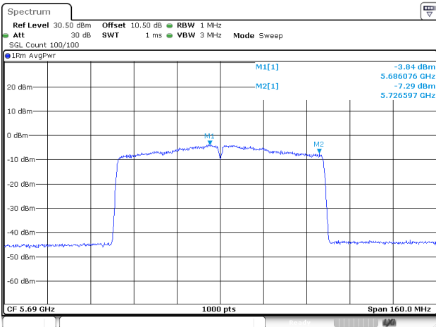
802.11ac80_5690MHz_Chain 2
