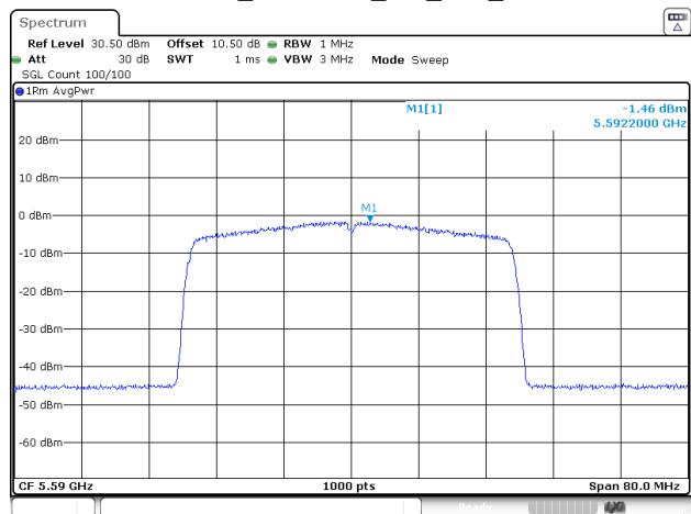
802.11be40_5590MHz_RU_Full_Chain 2
