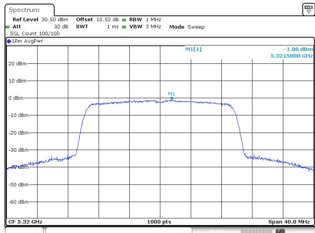
802.11be20_5320MHz_RU_Full_Chain 0
