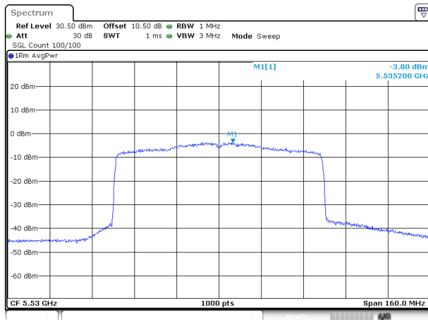
802.11be80_5530MHz_RU_Full_Chain 0
