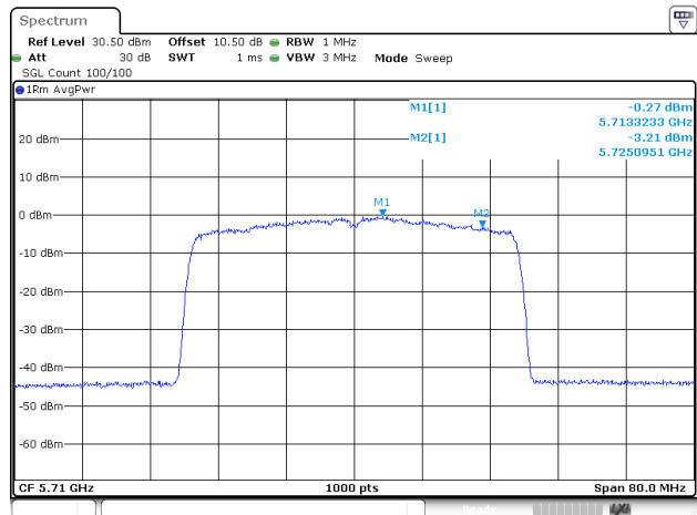
802.11be40_5710MHz_RU_Full_Chain 1
