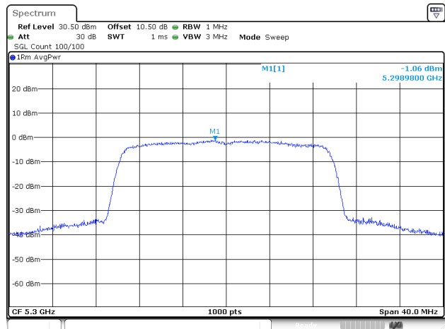
802.11be20_5300MHz_RU_Full_Chain 1
