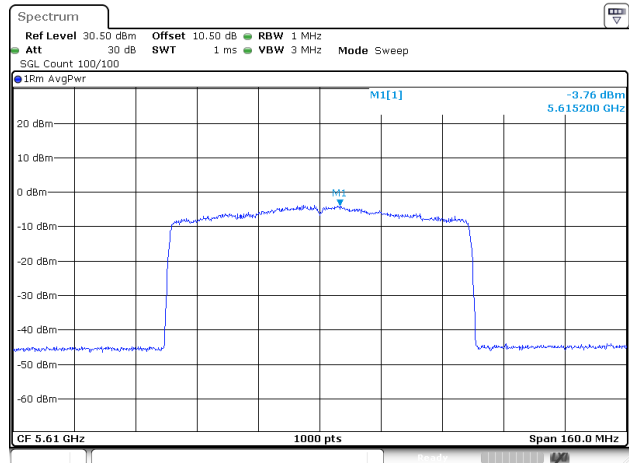
802.11be80_5610MHz_RU_Full_Chain 2
