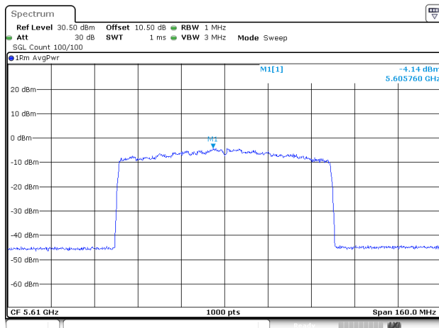
802.11be80_5610MHz_RU_Full_Chain 1
