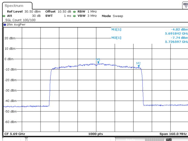
802.11be80_5690MHz_RU_Full_Chain 2
