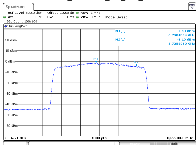
802.11be40_5710MHz_RU_Full_Chain 2
