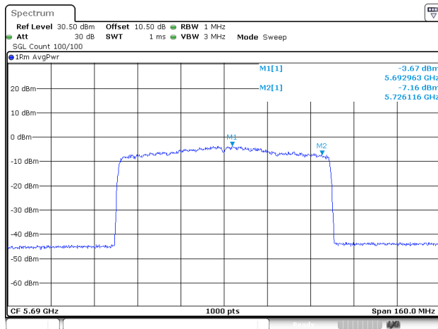
802.11be80_5690MHz_RU_Full_Chain 0
