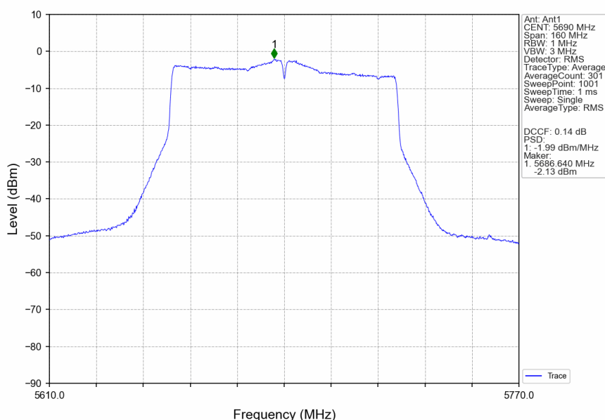
802.11ac(VHT80)_HCH_5690MHz_Ant1_NTNV
