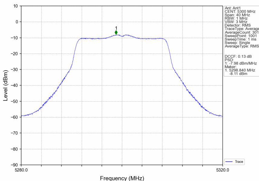
802.11ac(VHT20)_MCH_5300MHz_MIMO_NTNV
