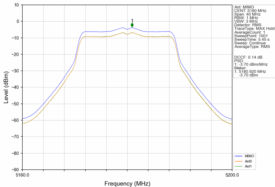
802.11ac(VHT20)_LCH_5180MHz_MIMO_NTNV
