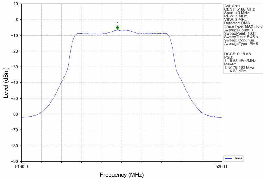
802.11ax(HEW20)_LCH_5180MHz_SU_/_MIMO_NTNV
