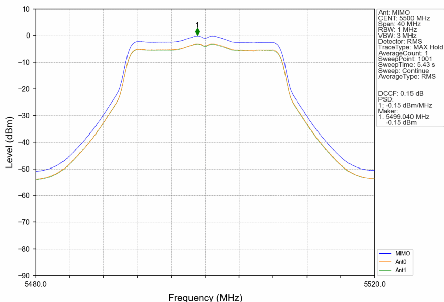
802.11ac(VHT20)_LCH_5500MHz_MIMO_NTNV
