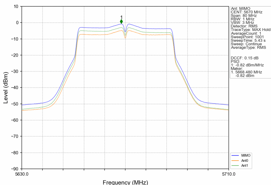
802.11n(HT40)_HCH_5670MHz_MIMO_NTNV
