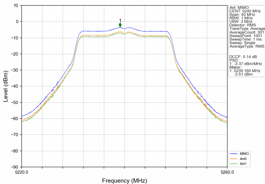
802.11ac(VHT20)_HCH_5240MHz_MIMO_NTNV
