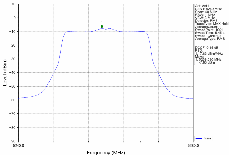
802.11ax(HEW20)_LCH_5260MHz_SU_ / _Ant1_NTNV
