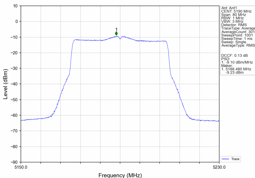
802.11ax(HEW40)_LCH_5190MHz_SU_ / _MIMO_NTNV
