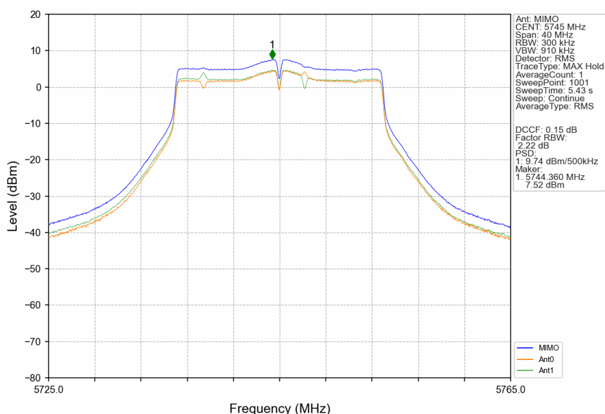
802.11ac(VHT20)_LCH_5745MHz_MIMO_NTNV
