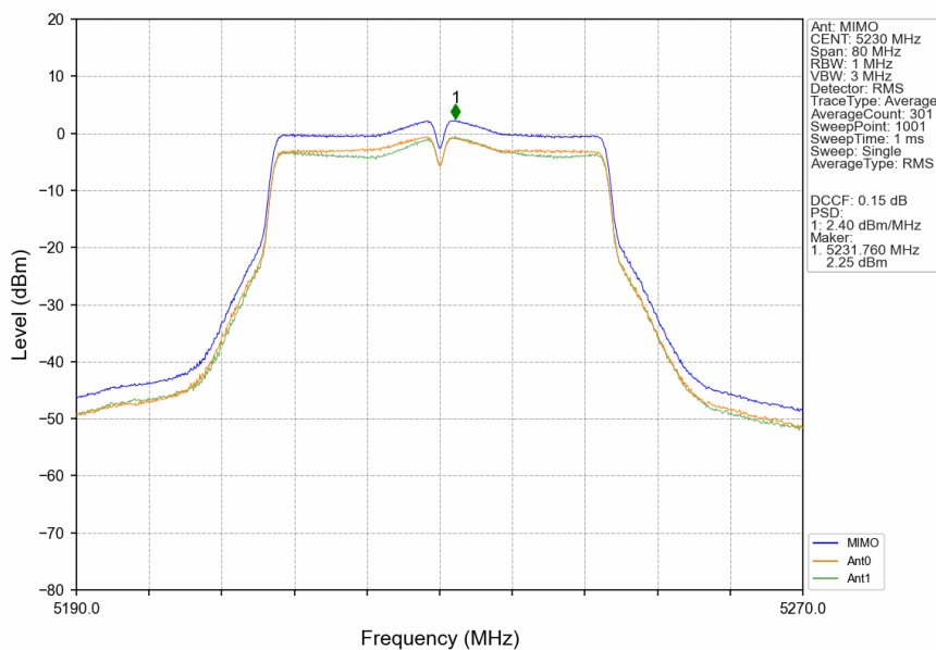
802.11ac(VHT40)_HCH_5230MHz_MIMO_NTNV
