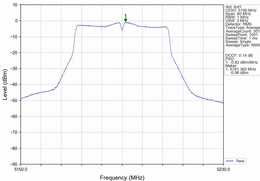
802.11ac(VHT40)_LCH_5190MHz_Ant1_NTNV
