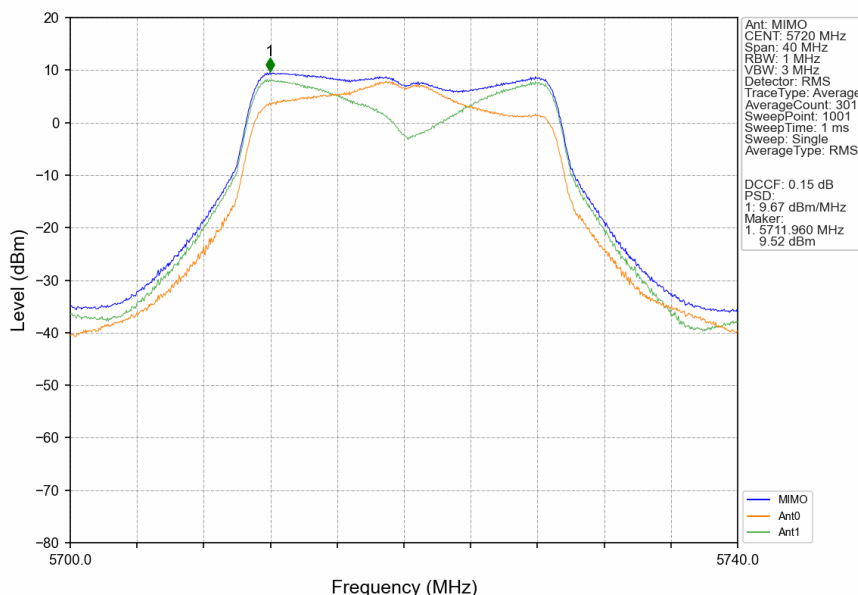
802.11ac(VHT20)_HCH_5720MHz_MIMO_NTNV
