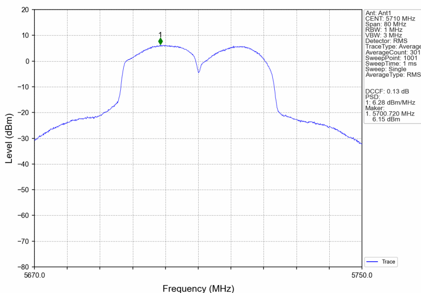
802.11n(HT40)_HCH_5710MHz_MIMO_NTNV
