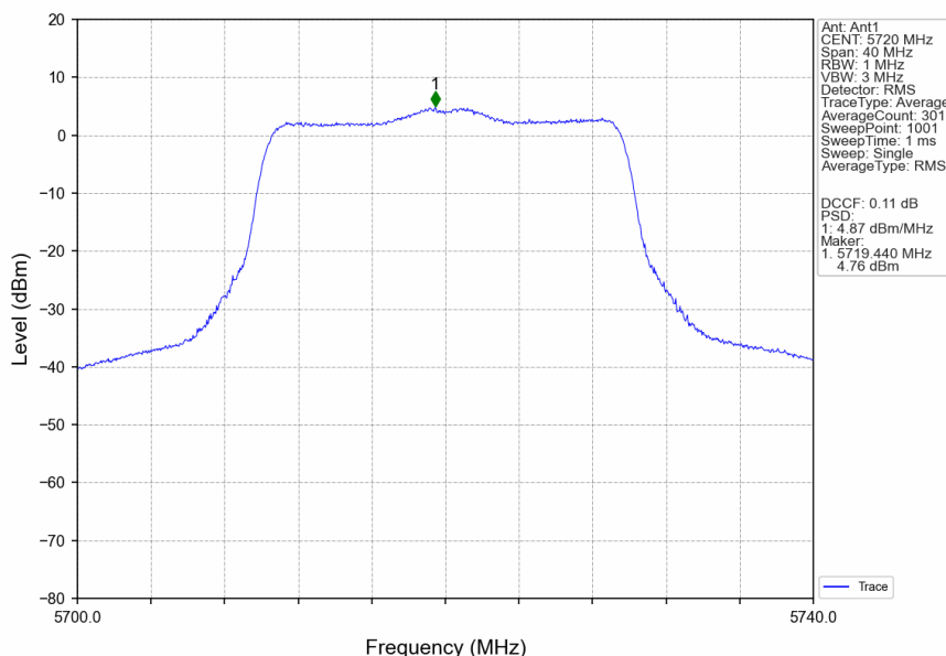
802.11ax(HEW20)_HCH_5720MHz_SU_/_Ant1_NTNV
