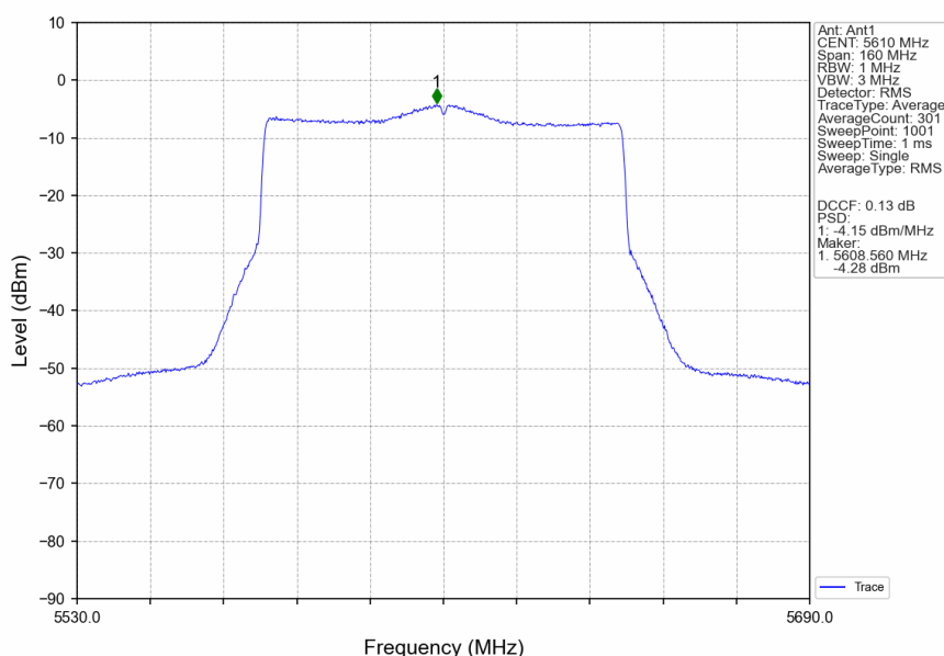
802.11ax(HEW80)_HCH_5610MHz_SU_/_Ant1_NTNV
