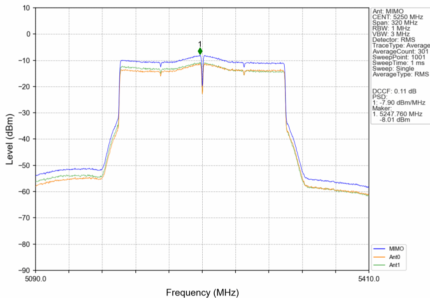
802.11ax(HEW160)_MCH_5250MHz_SU_/_MIMO_NTNV
