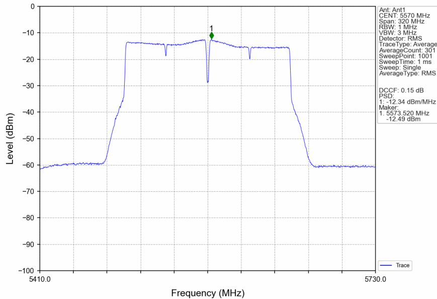
802.11ac(VHT160)_MCH_5570MHz_MIMO_NTNV
