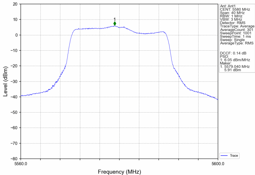
802.11ax(HEW20)_MCH_5580MHz_SU_/_Ant1_NTNV
