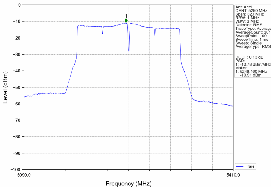
802.11ac(VHT160)_MCH_5250MHz_Ant1_NTNV
