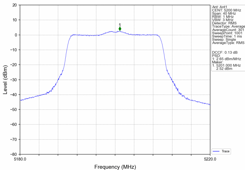
802.11ax(HEW20)_MCH_5200MHz_SU_/_Ant1_NTNV
