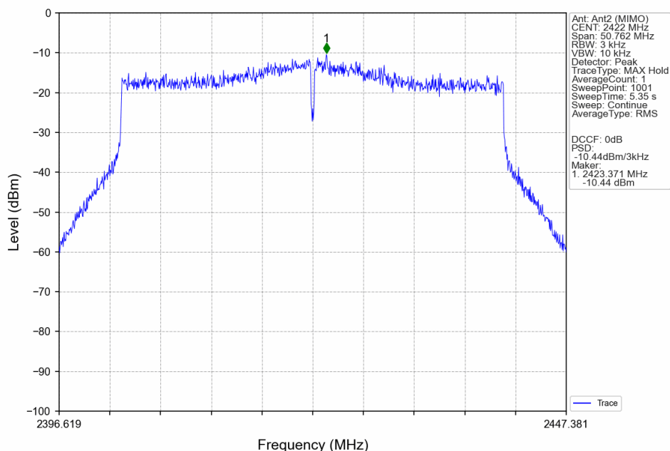
802.11ax(HEW40)_LCH_2422MHz_SU_/_MIMO_NTNV
