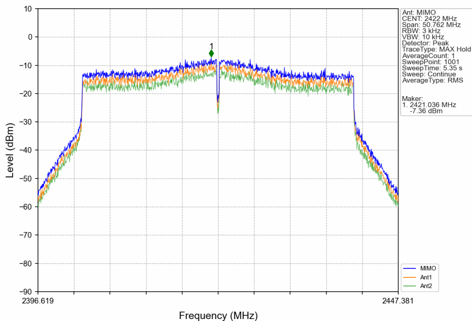
802.11ax(HEW40)_LCH_2422MHz_SU_/_MIMO_NTNV
