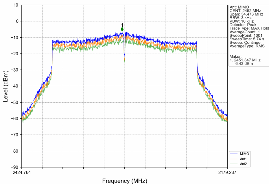
802.11ax(HEW40)_HCH_2452MHz_SU_/_MIMO_NTNV
