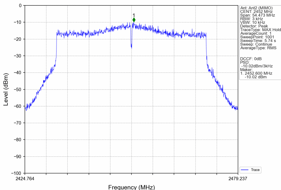
802.11ax(HEW40)_HCH_2452MHz_SU_/_MIMO_NTNV
