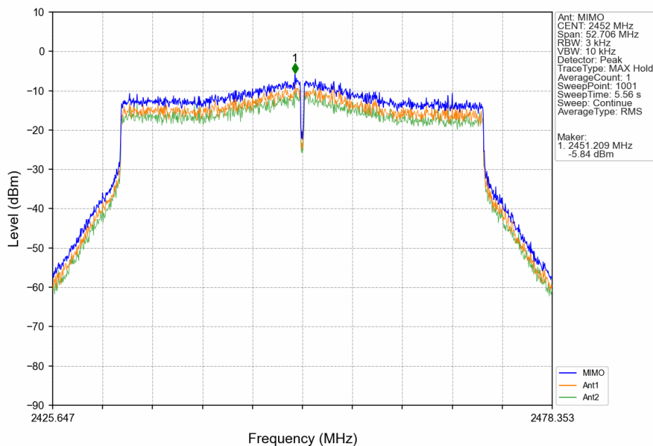
802.11be(EHT40)_HCH_2452MHz_SU_/_MIMO_NTNV
