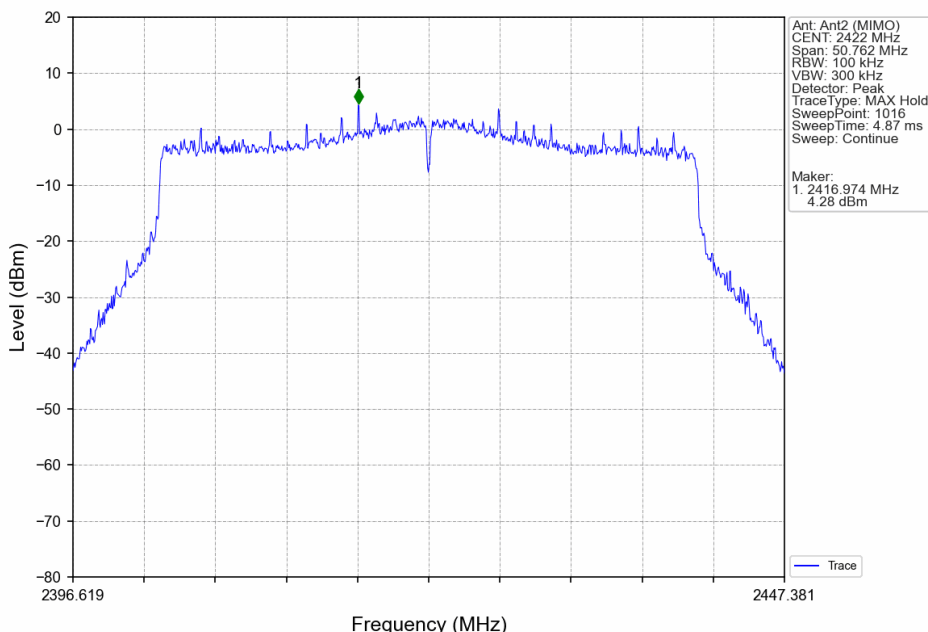
802.11ax(HEW40)_LCH_2422MHz_SU_/_Ant2 (MIMO)_NTNV
