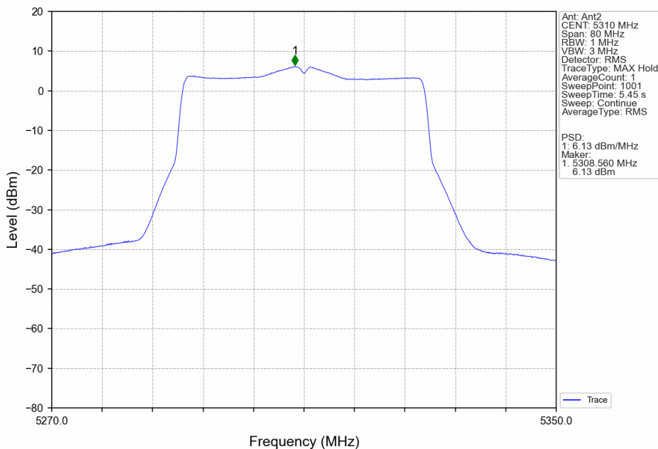
802.11ax(HEW40)_HCH_5310MHz_SU_/_MIMO_NTNV
