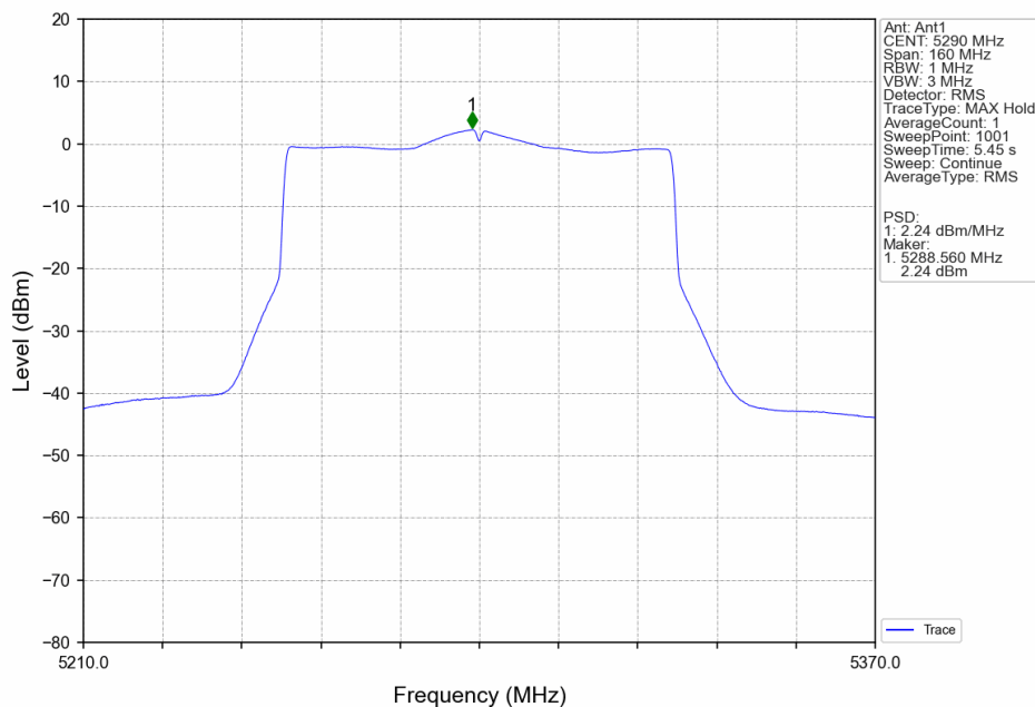
802.11ax(HEW80)_MCH_5290MHz_SU_/_Ant1_NTNV
