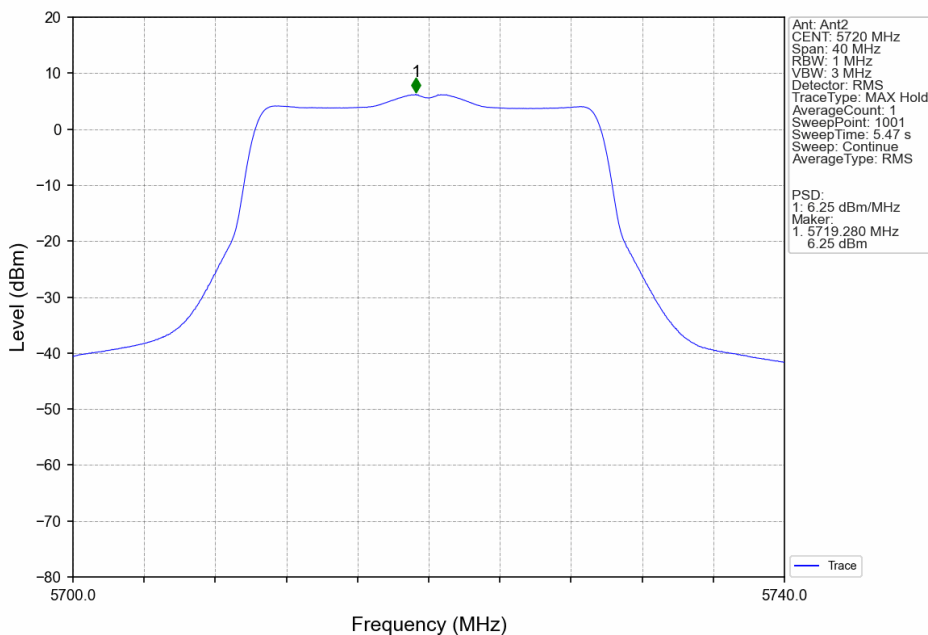
802.11ax(HEW20)_HCH_5720MHz_SU_/_Ant2_NTNV
