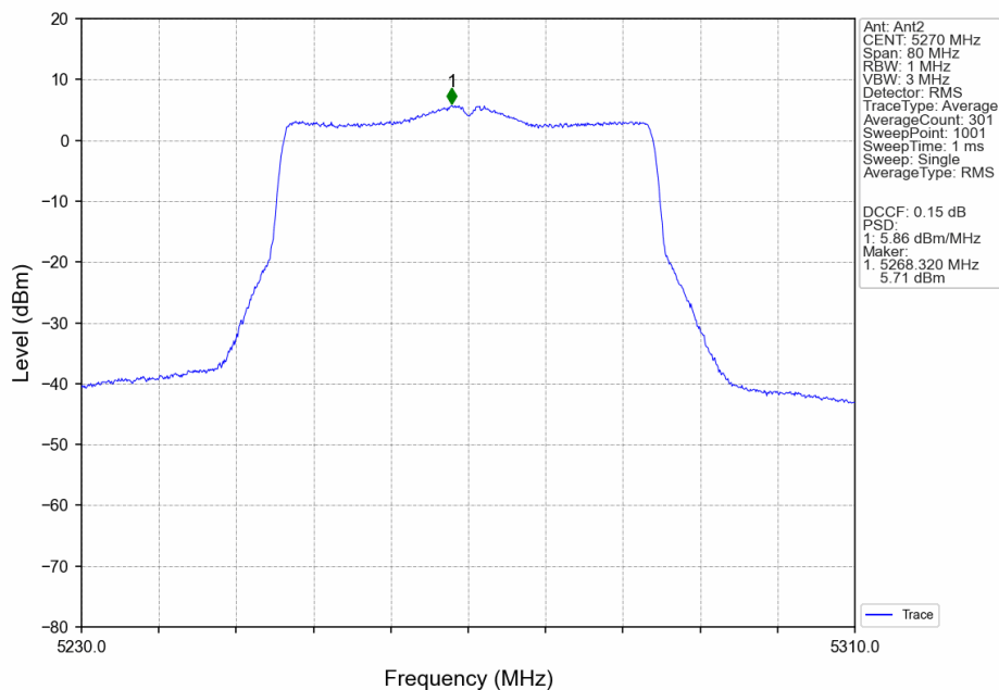
802.11ax(HEW40)_LCH_5270MHz_SU_ / _Ant2_NTNV
