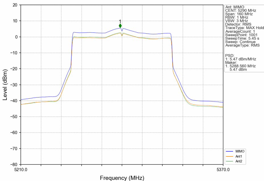
802.11ax(HEW80)_MCH_5290MHz_SU_/_MIMO_NTNV
