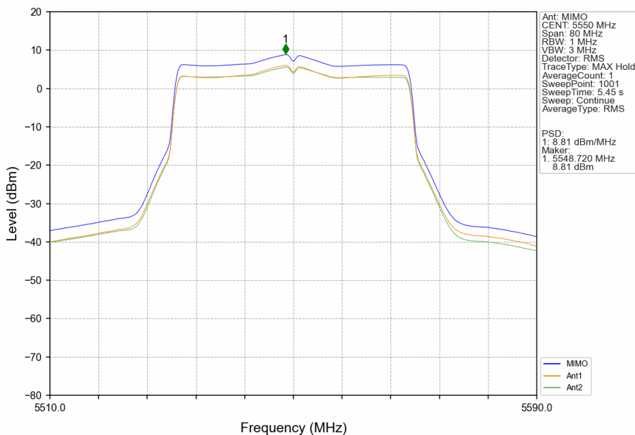
802.11ax(HEW40)_MCH_5550MHz_SU_/_MIMO_NTNV
