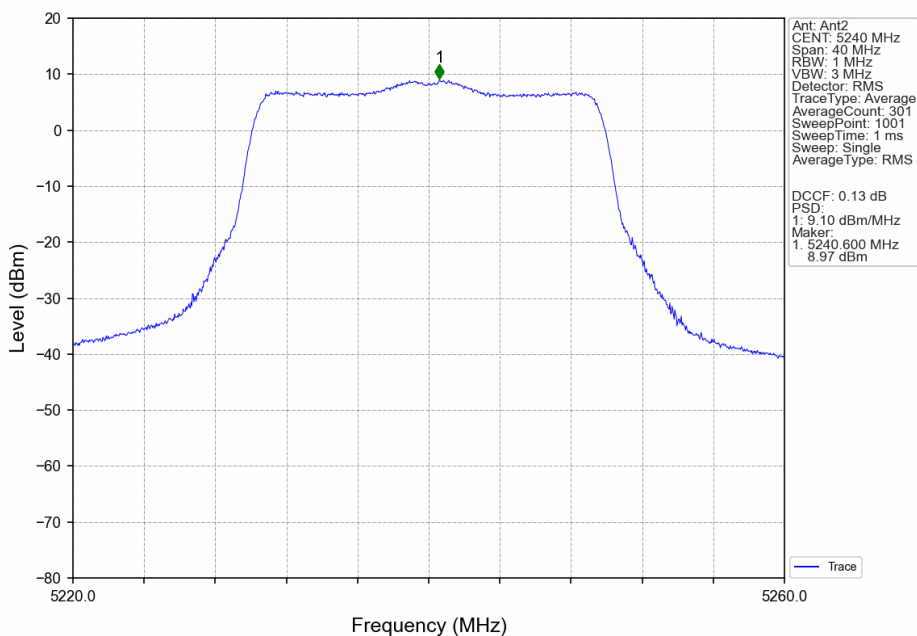
802.11be(EHT20)_HCH_5240MHz_SU_/_MIMO_NTNV
