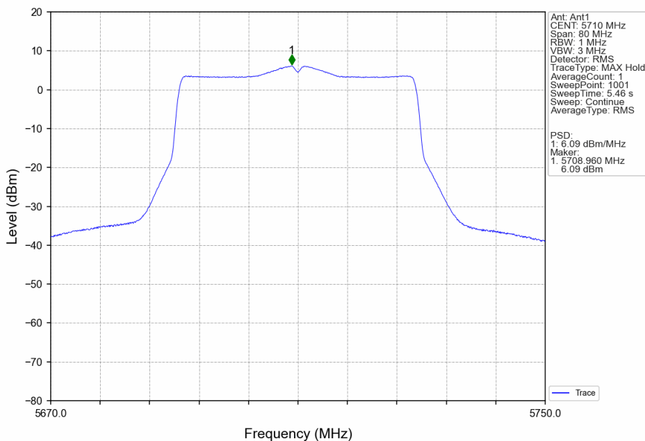
802.11ax(HEW40)_HCH_5710MHz_SU_/_Ant1_NTNV
