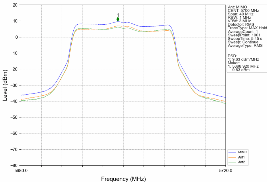
802.11ax(HEW20)_HCH_5700MHz_SU_/_MIMO_NTNV
