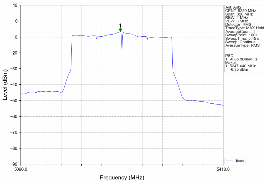
802.11ax(HEW160)_MCH_5250MHz_SU_/_MIMO_NTNV
