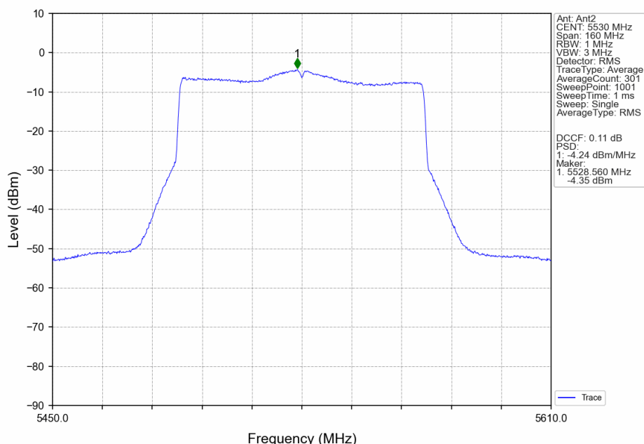
802.11ax(HEW80)_LCH_5530MHz_SU_ / _Ant2_NTNV
