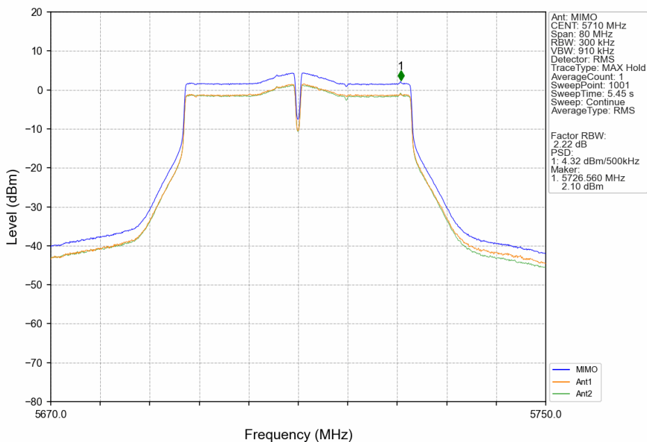
802.11ac(VHT40)_HCH_5710MHz_MIMO_NTNV
