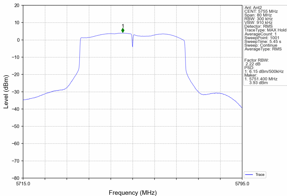
802.11ax(HEW40)_LCH_5755MHz_SU_ / _Ant2_NTNV
