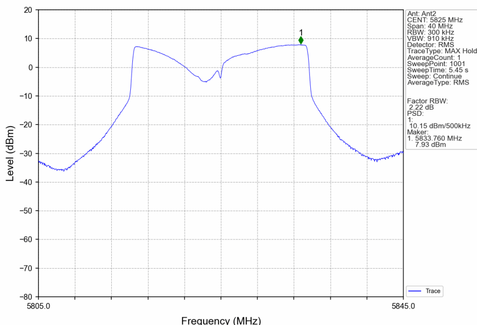
802.11ax(HEW20)_HCH_5825MHz_SU_ / _Ant2_NTNV
