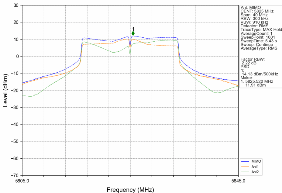
802.11ac(VHT20)_HCH_5825MHz_MIMO_NTNV
