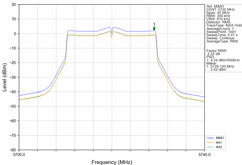
802.11ax(HEW20)_HCH_5720MHz_SU_/_MIMO_NTNV
