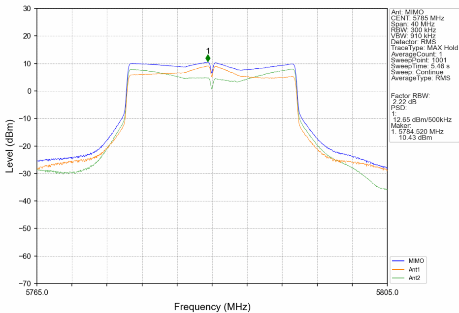
802.11ax(HEW20)_MCH_5785MHz_SU_/_MIMO_NTNV
