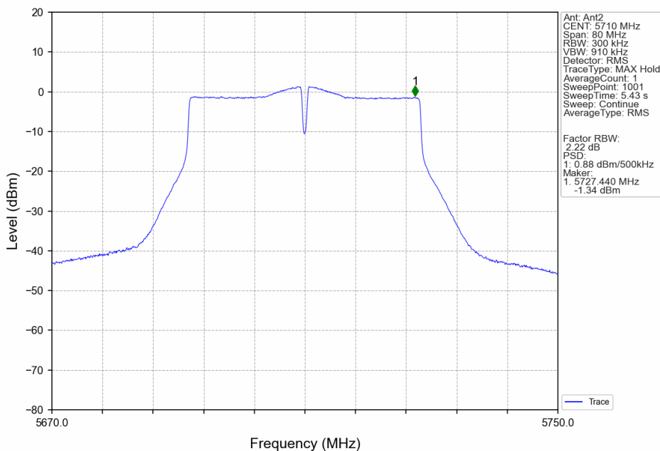
802.11n(HT40)_HCH_5710MHz_Ant2_NTNV
