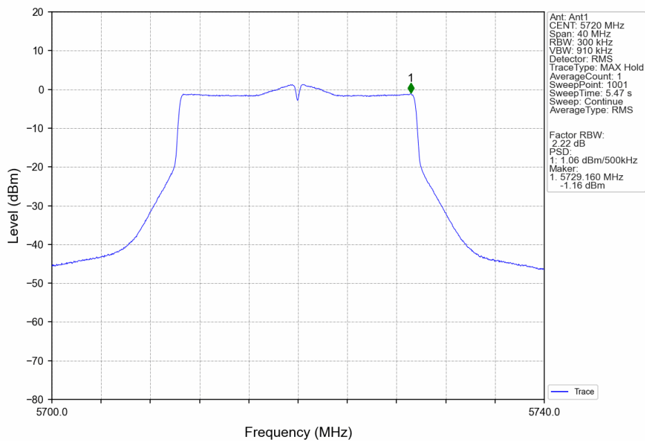
802.11ax(HEW20)_HCH_5720MHz_SU_/_Ant1_NTNV
