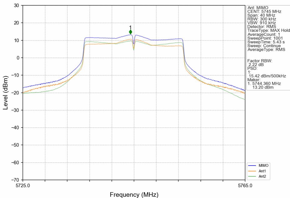
802.11ac(VHT20)_LCH_5745MHz_MIMO_NTNV
