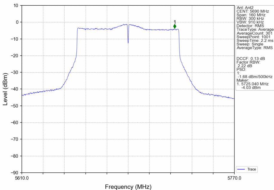
802.11ac(VHT80)_HCH_5690MHz_MIMO_NTNV
