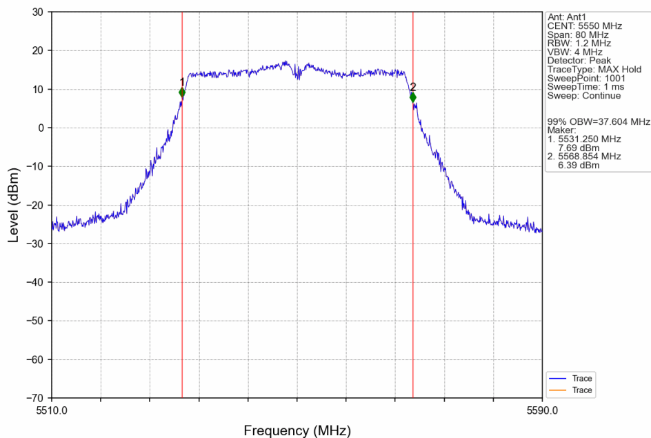
802.11ac(VHT40)_MCH_5550MHz_Ant1_NTNV
