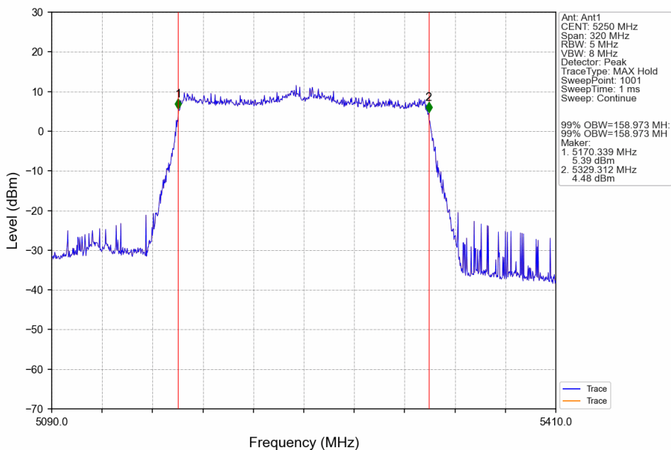
802.11ax(HEW160)_MCH_5250MHz_SU_/_Ant1_NTNV
