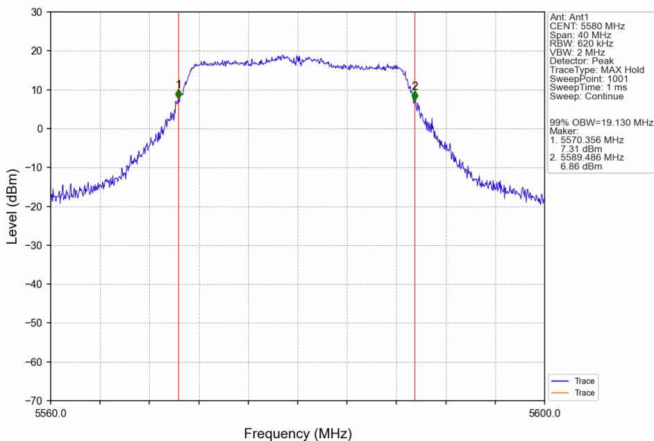
802.11ac(VHT20)_MCH_5580MHz_Ant1_NTNV
