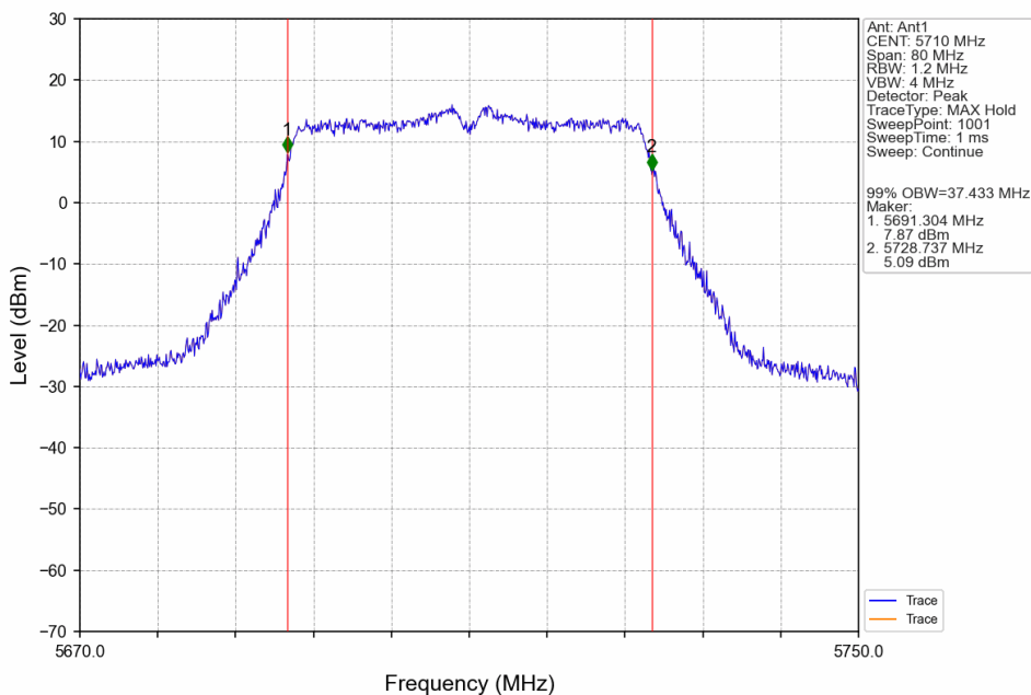
802.11ac(VHT40)_HCH_5710MHz_Ant1_NTNV
