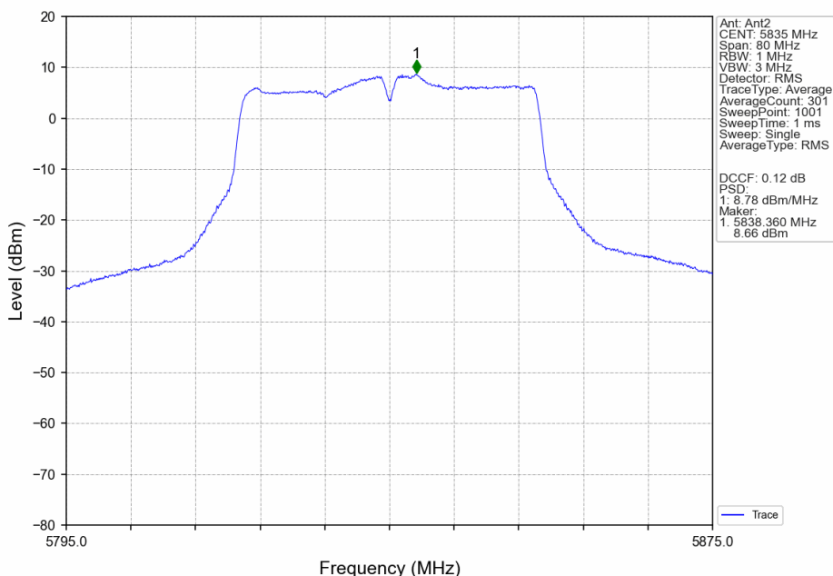
802.11ac(VHT40)_HCH_5835MHz_MIMO_NTNV
