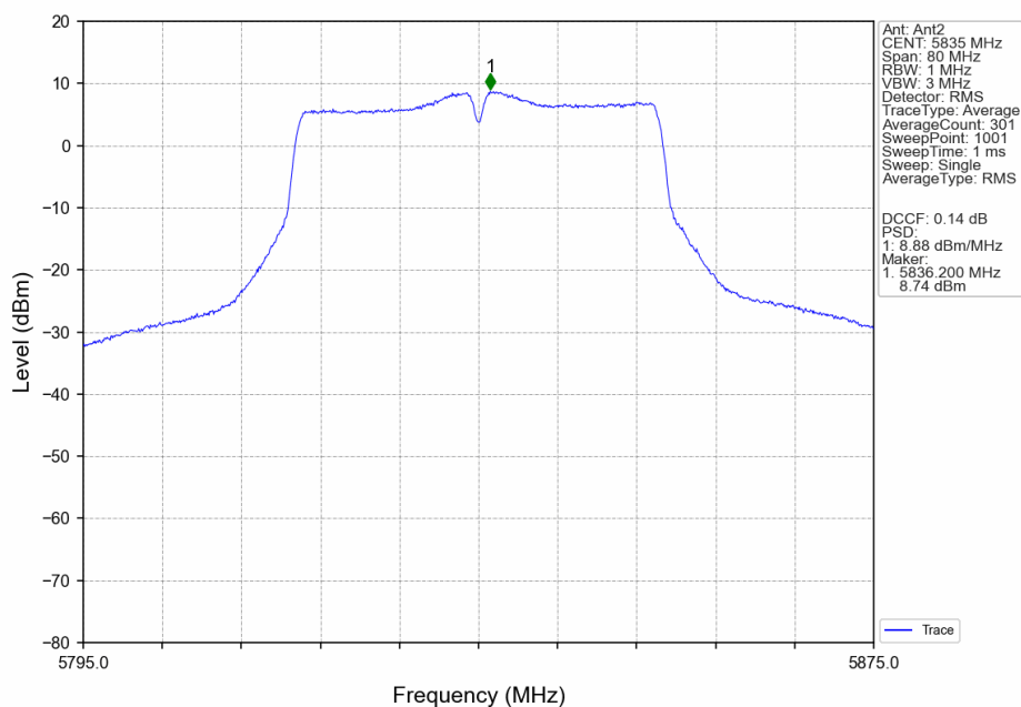
802.11n(HT40)_HCH_5835MHz_Ant2_NTNV
