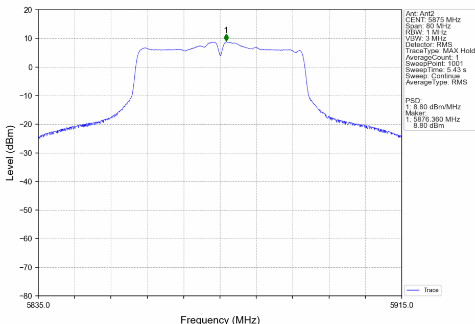
802.11ac(VHT40)_MCH_5875MHz_Ant2_NTNV
