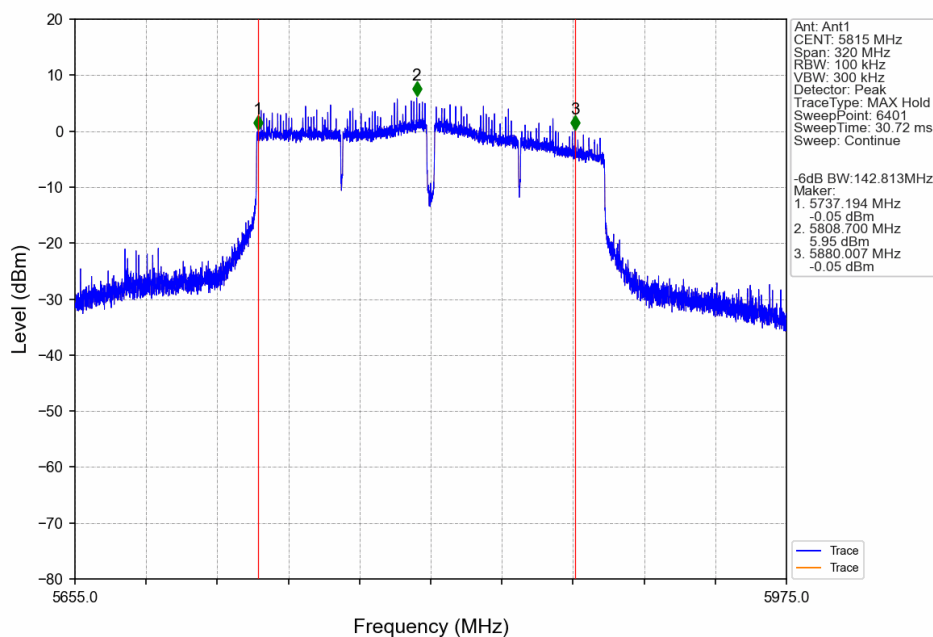
802.11ac(VHT160)_HCH_5815MHz_Ant1_NTNV
