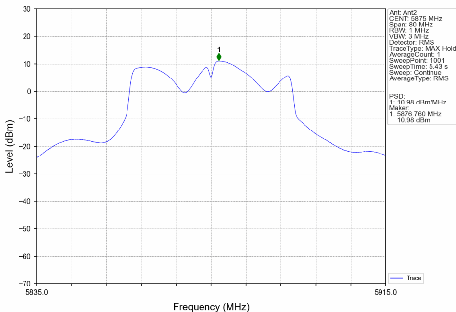
802.11n(HT40)_MCH_5875MHz_MIMO_NTNV
