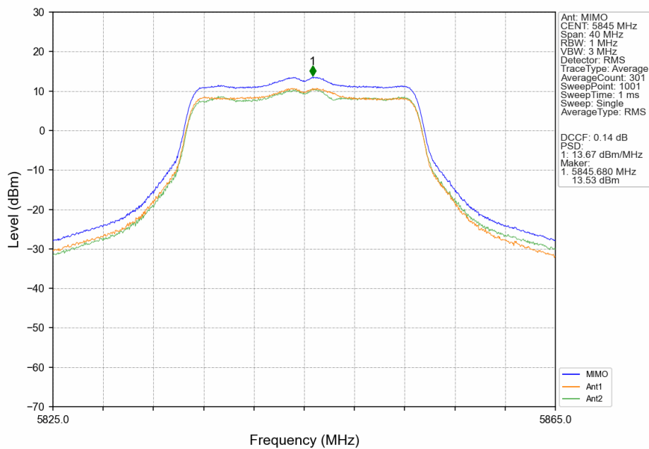
802.11ac(VHT20)_HCH_5845MHz_MIMO_NTNV
