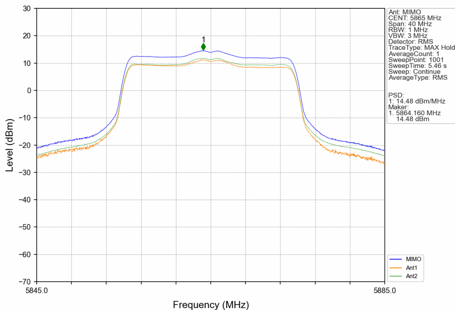
802.11ax(HEW20)_LCH_5865MHz_SU_ / _MIMO_NTNV
