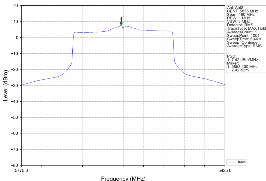
802.11ax(HEW80)_HCH_5855MHz_SU_/_Ant2_NTNV
