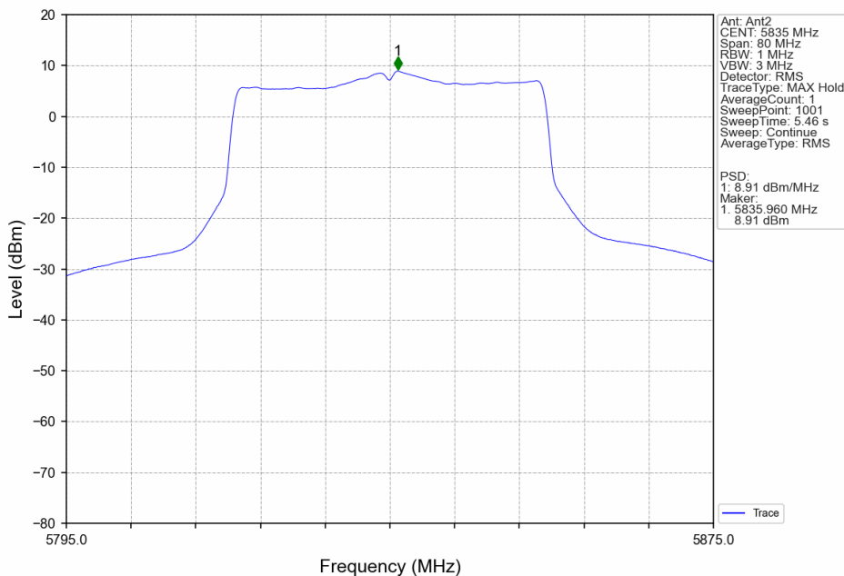
802.11ax(HEW40)_HCH_5835MHz_SU_/_MIMO_NTNV
