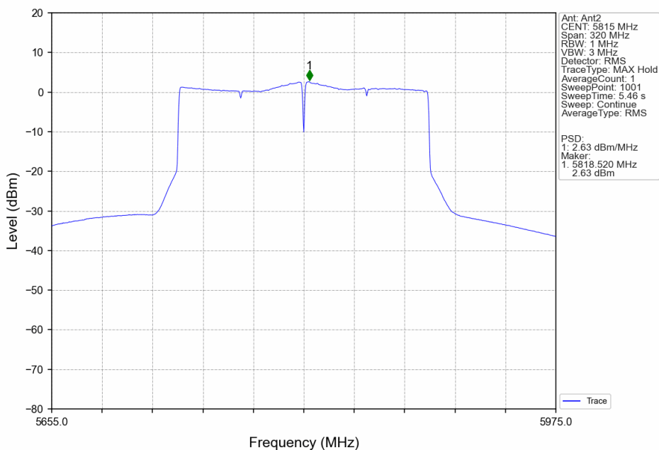
802.11ax(HEW160)_HCH_5815MHz_SU_/_MIMO_NTNV
