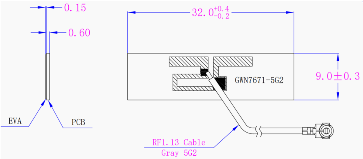
总成图 Mechanical Drawing(unit:mm)
