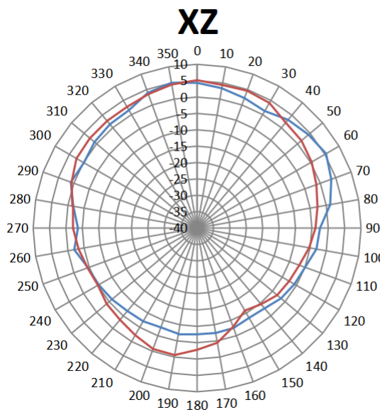
5G Antenna Radiation Patterns(unit:dB)
