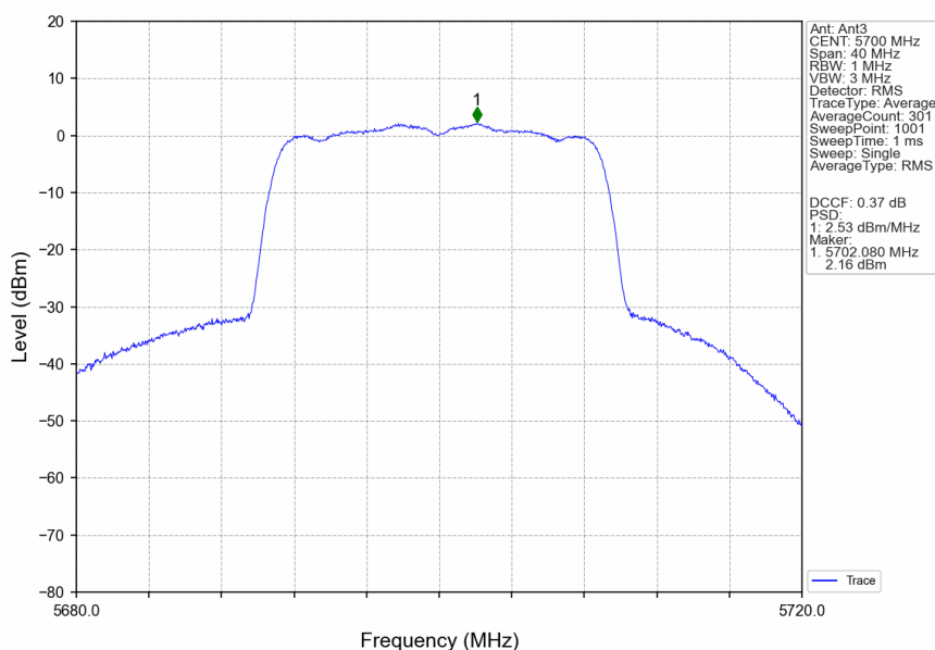
802.11ac(VHT20)_HCH_5700MHz_MIMO_NTNV
