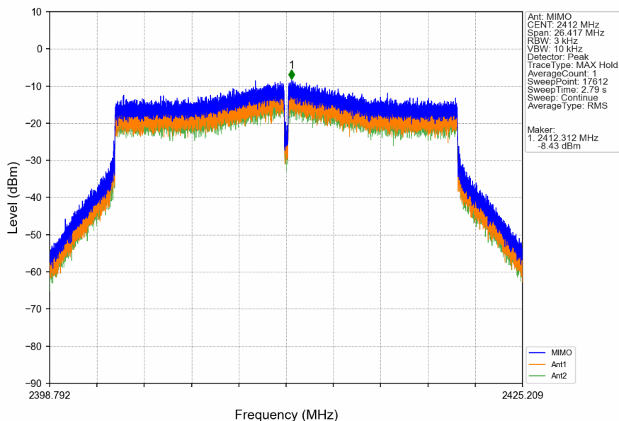
802.11ax(HEW20)_LCH_2412MHz_RU242_Left_MIMO_NTNV
