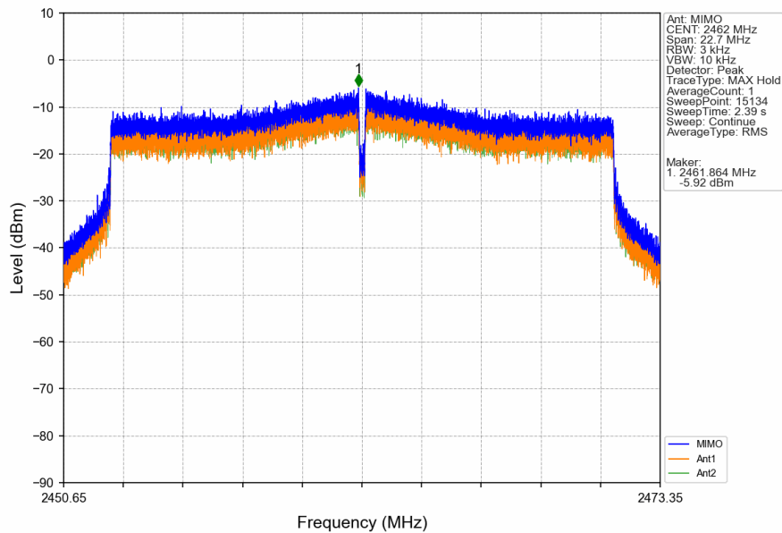
802.11ax(HEW20)_HCH_2462MHz_RU242_Left_MIMO_NTNV
