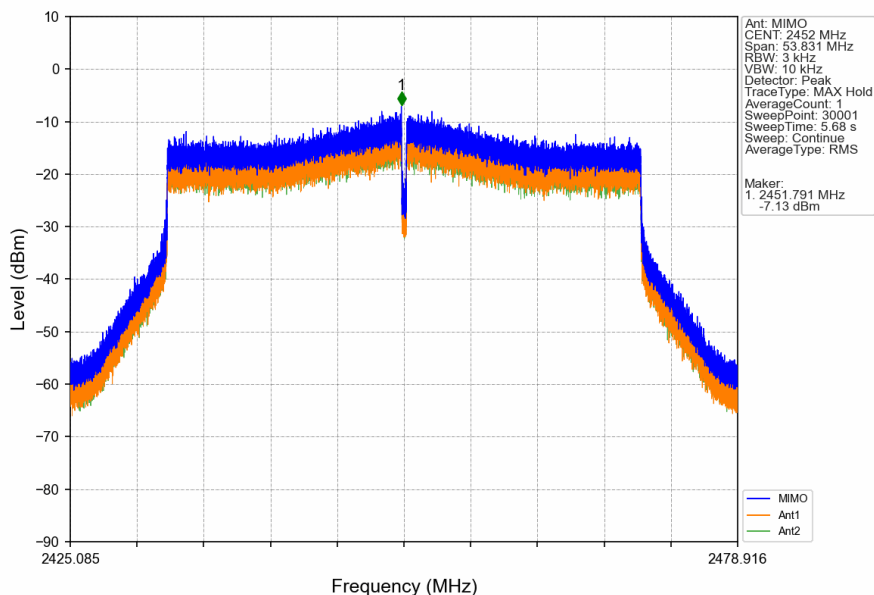
802.11ax(HEW40)_HCH_2452MHz_RU484_Left_MIMO_NTNV
