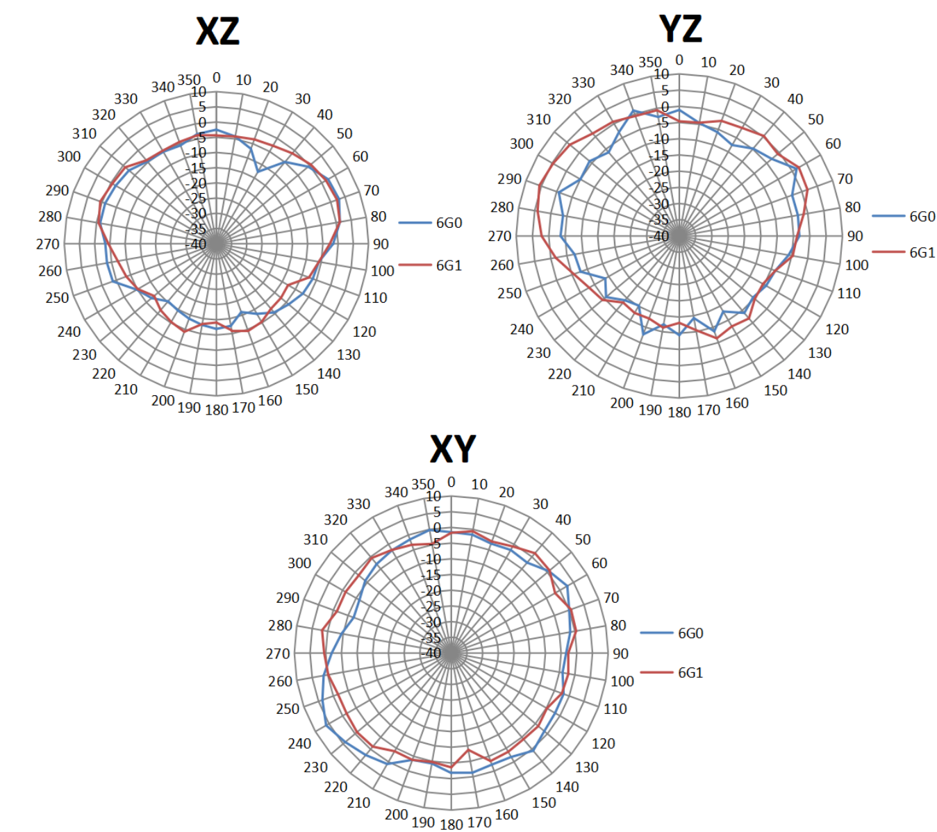
6G Antenna Radiation Patterns(unit: dB)
