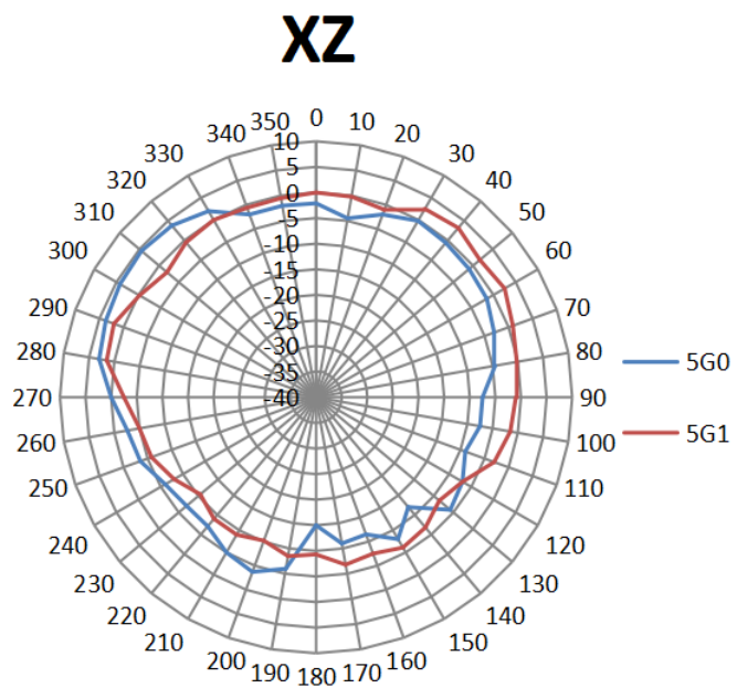
5G Antenna Radiation Patterns (unit: dB)
