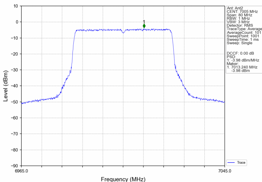
802.11ax(HEW40)_MCH_7005MHz_RU484_Left_Ant2_NTNV
