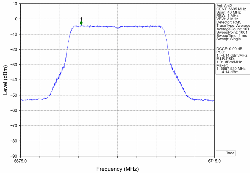
802.11ax(HEW20)_MCH_6695MHz_RU242_Left_Ant2_NTNV
