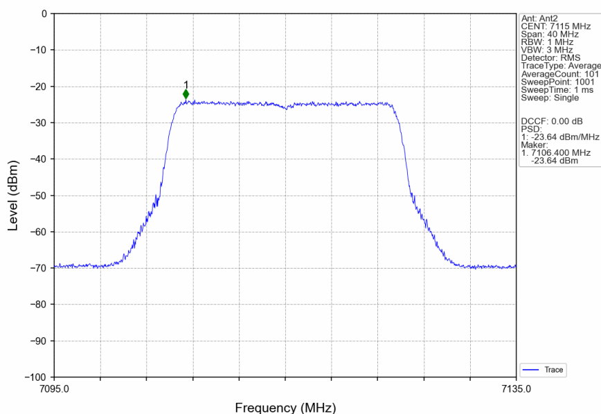
802.11ax(HEW20)_HCH_7115MHz_RU242_Left_Ant2_NTNV
