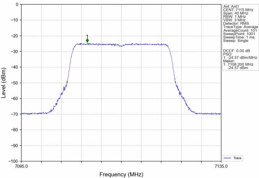
802.11ax(HEW20)_HCH_7115MHz_RU242_Left_Ant1_NTNV
