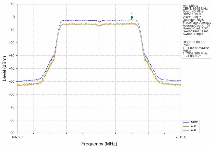
802.11ax(HEW20)_MCH_6995MHz_RU242_Left_MIMO_NTNV
