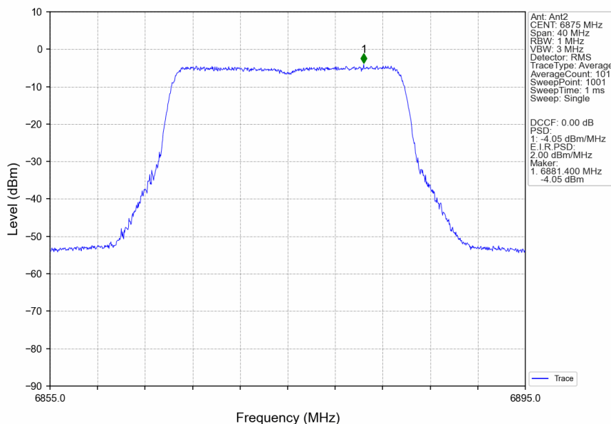
802.11ax(HEW20)_HCH_6875MHz_RU242_Left_Ant2_NTNV
