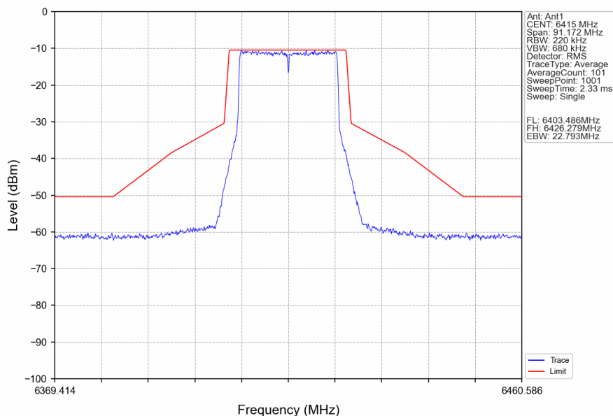
802.11ax(HEW20)_HCH_6415MHz_RU242_Left_Ant1_NTNV
