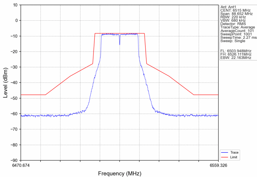
802.11a_HCH_6515MHz_Ant1_NTNV
