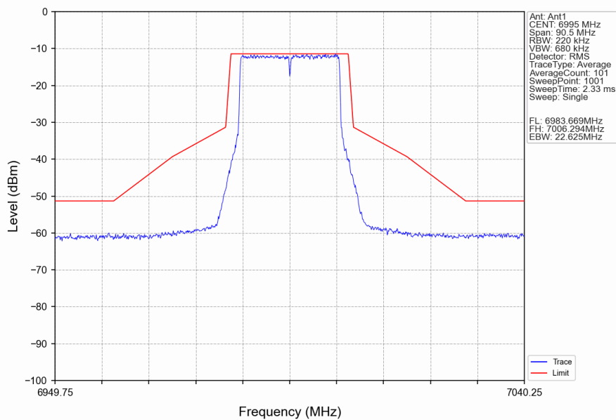
802.11ax(HEW20)_MCH_6995MHz_RU242_Left_Ant1_NTNV
