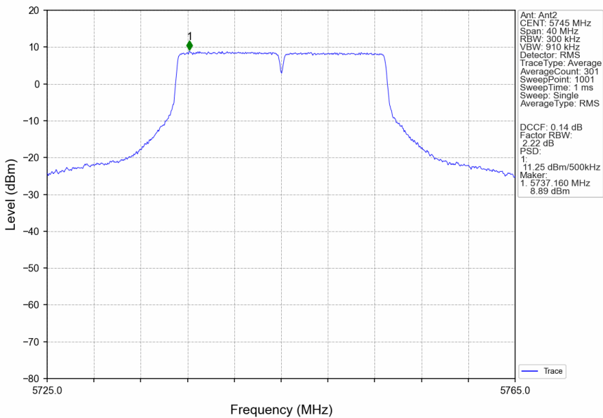
802.11ac(VHT20)_LCH_5745MHz_Ant2_NTNV
