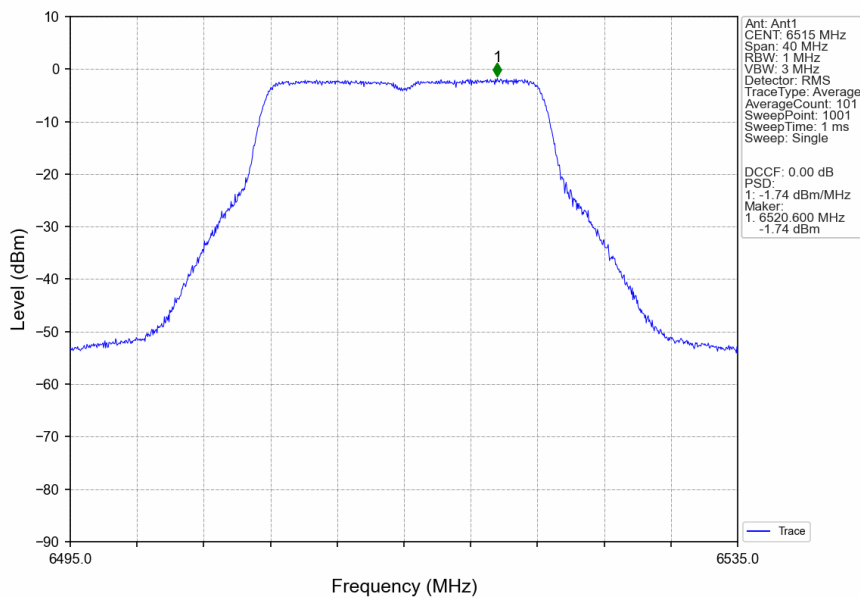
802.11a_HCH_6515MHz_Ant1_NTNV
