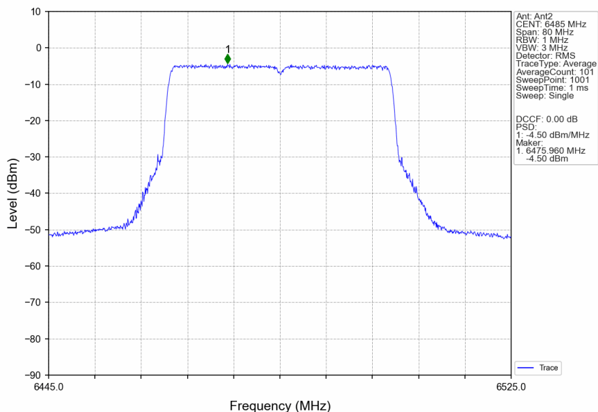
802.11ax(HEW40)_MCH_6485MHz_RU484_Left_Ant2_NTNV
