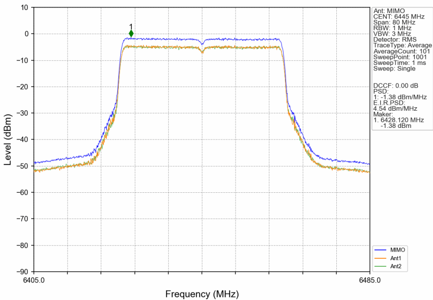
802.11ax(HEW40)_LCH_6445MHz_RU484_Left_MIMO_NTNV
