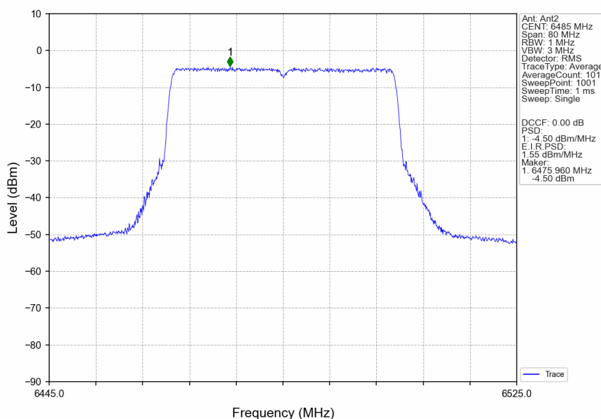
802.11ax(HEW40)_MCH_6485MHz_RU484_Left_Ant2_NTNV
