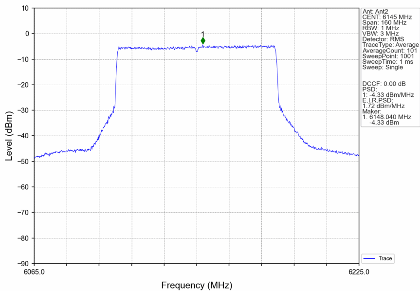
802.11ax(HEW80)_MCH_6145MHz_RU996_Left_Ant2_NTNV
