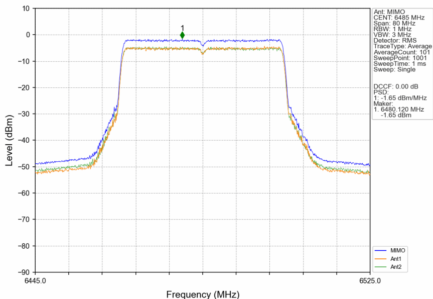
802.11ax(HEW40)_MCH_6485MHz_RU484_Left_MIMO_NTNV
