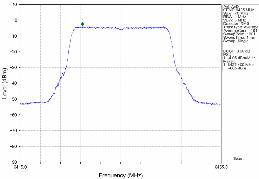
802.11ax(HEW20)_LCH_6435MHz_RU242_Left_Ant2_NTNV
