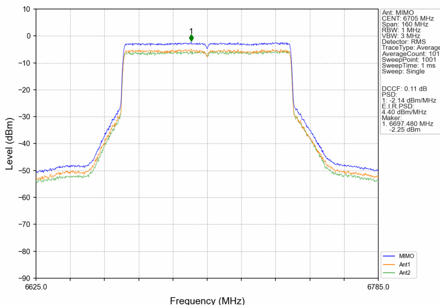
802.11ax(HEW80)_MCH_6705MHz_SU_/_MIMO_NTNV
