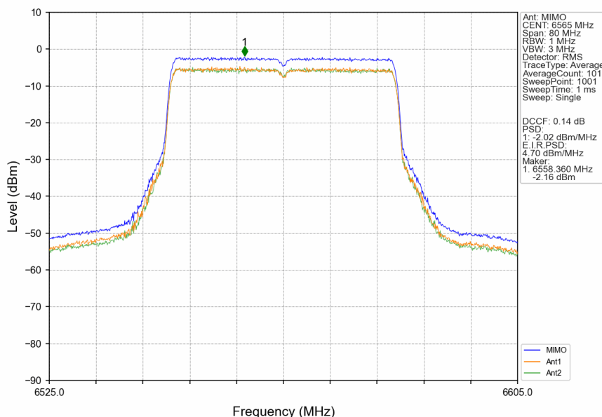
802.11ax(HEW40)_LCH_6565MHz_SU_ / _MIMO_NTNV
