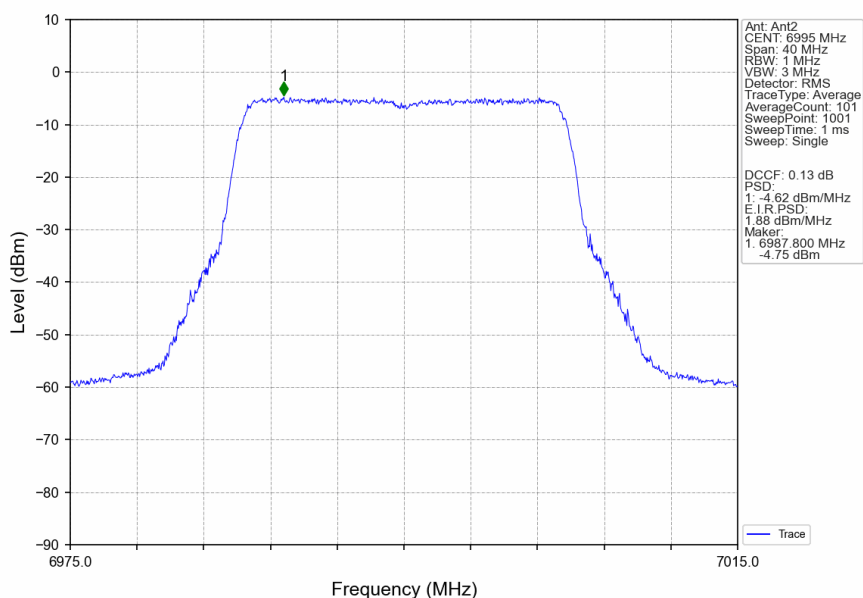
802.11ax(HEW20)_MCH_6995MHz_SU_/_MIMO_NTNV
