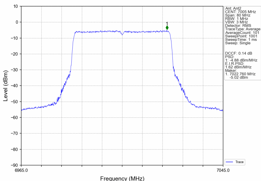
802.11ax(HEW40)_MCH_7005MHz_SU_/_Ant2_NTNV
