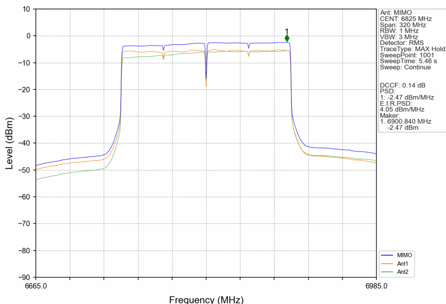
802.11ax(HEW160)_HCH_6825MHz_SU_/_MIMO_NTNV
