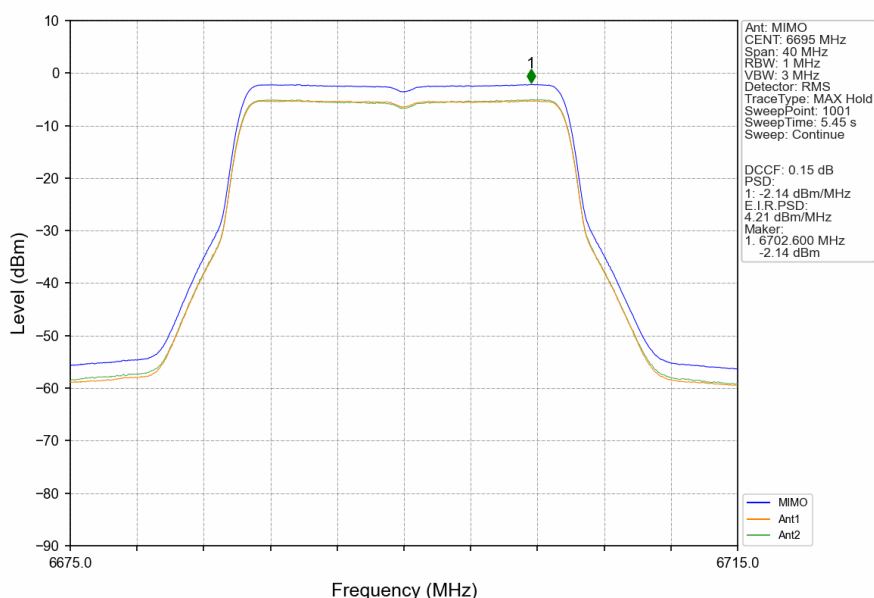
802.11ax(HEW20)_MCH_6695MHz_SU_/_MIMO_NTNV
