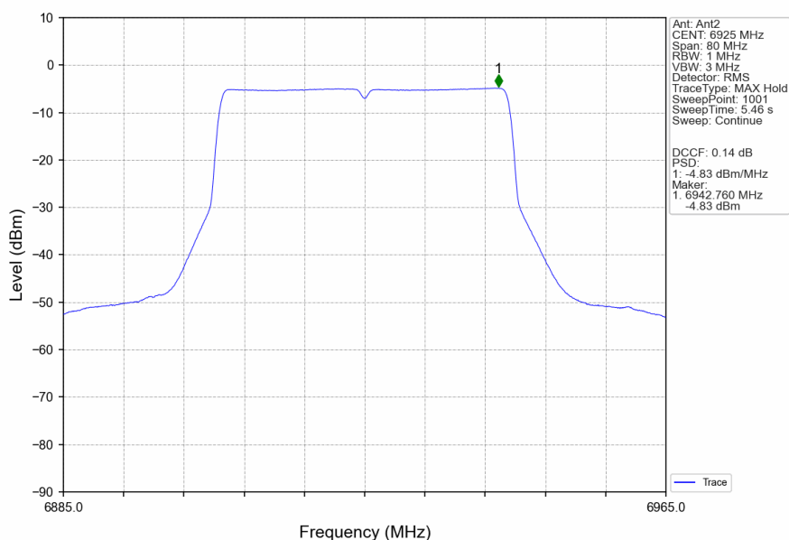
802.11ax(HEW40)_LCH_6925MHz_SU_/_MIMO_NTNV
