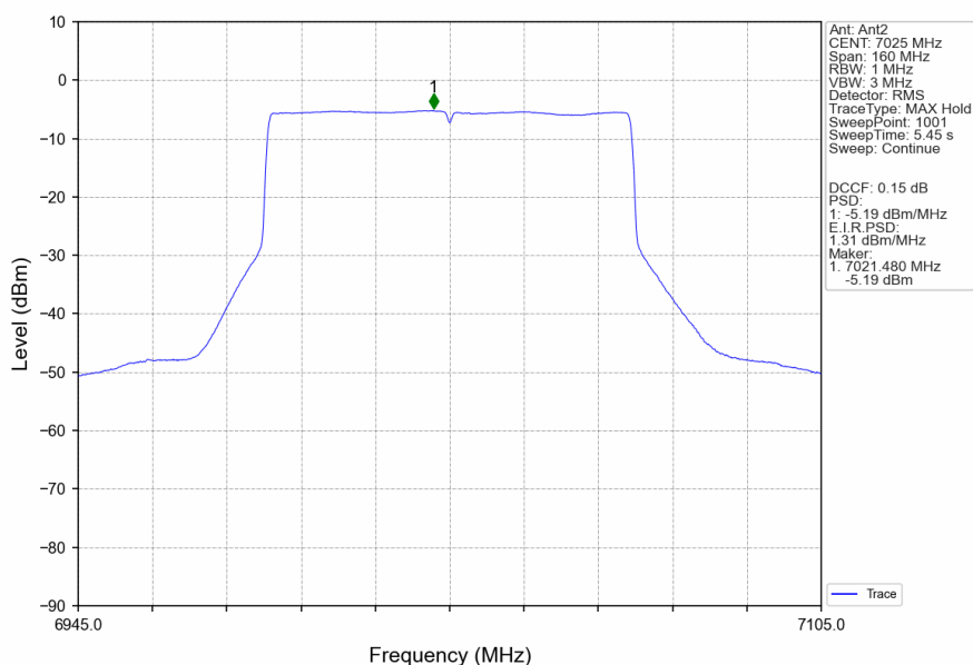
802.11ax(HEW80)_HCH_7025MHz_SU_/_MIMO_NTNV
