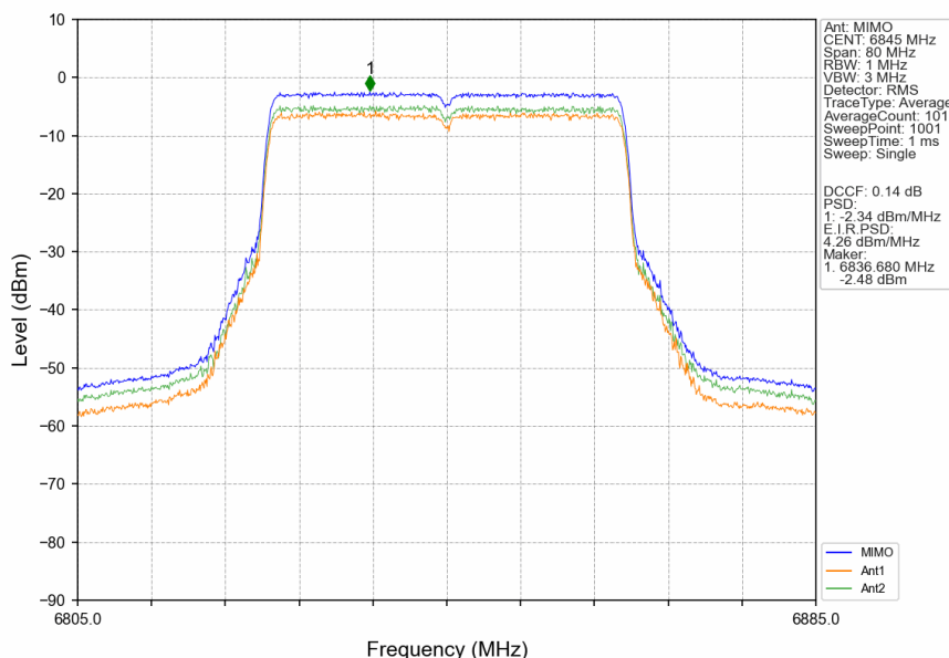
802.11ax(HEW40)_HCH_6845MHz_SU_/_MIMO_NTNV
