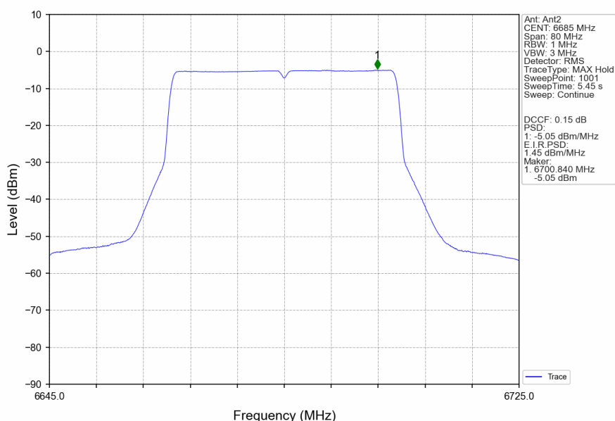
802.11ax(HEW40)_MCH_6685MHz_SU_/_Ant2_NTNV
