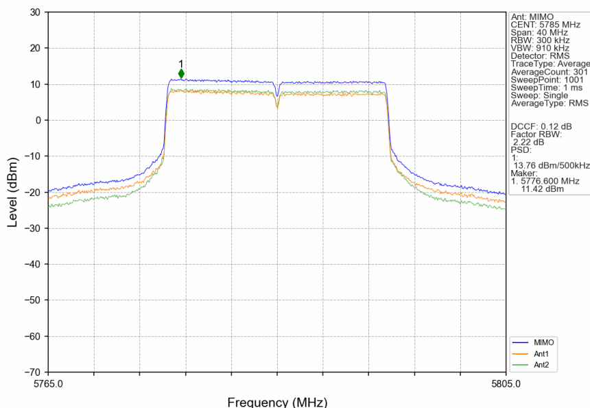
802.11ax(HEW20)_MCH_5785MHz_SU_/_MIMO_NTNV
