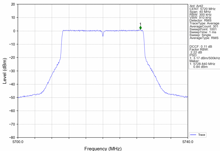
802.11ax(HEW20)_HCH_5720MHz_SU_/_MIMO_NTNV
