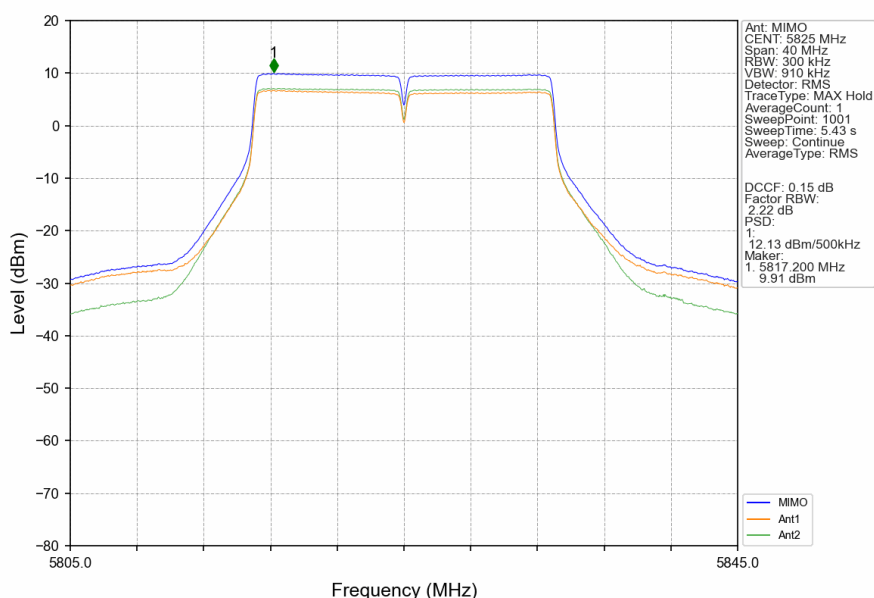
802.11ac(VHT20)_HCH_5825MHz_MIMO_NTNV
