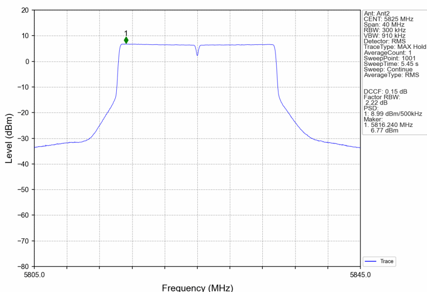
802.11ax(HEW20)_HCH_5825MHz_SU_/_Ant2_NTNV
