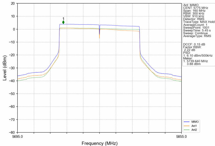
802.11ax(HEW80)_MCH_5775MHz_SU_/_MIMO_NTNV
