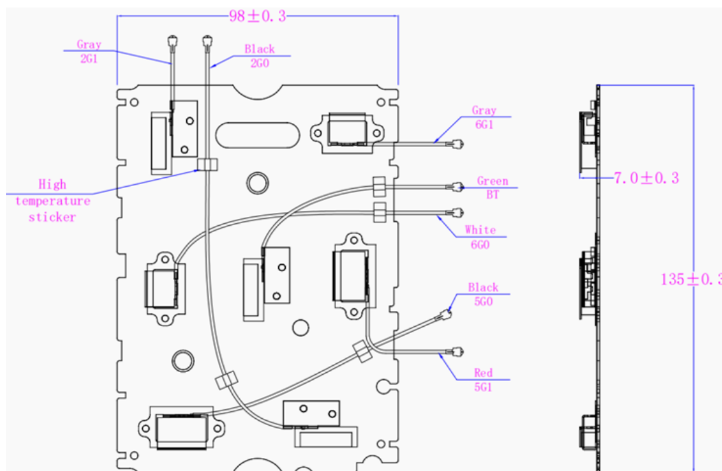
总成图 Mechanical Drawing(unit:mm)
