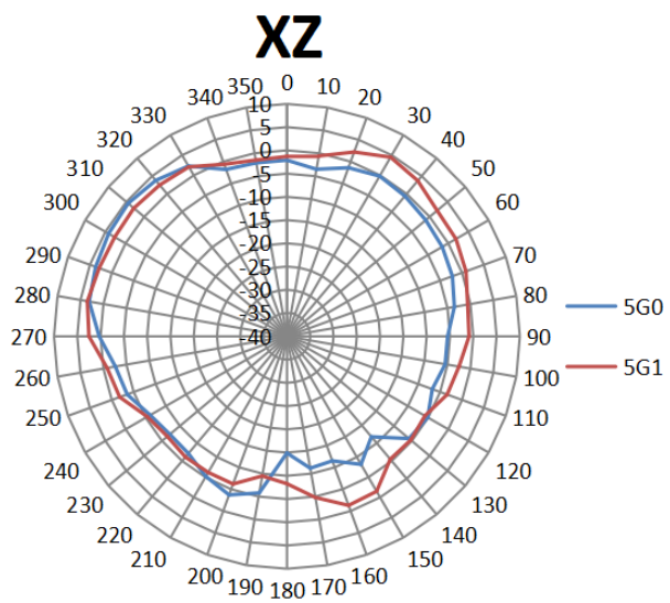
5G Antenna Radiation Patterns(unit:dB)
