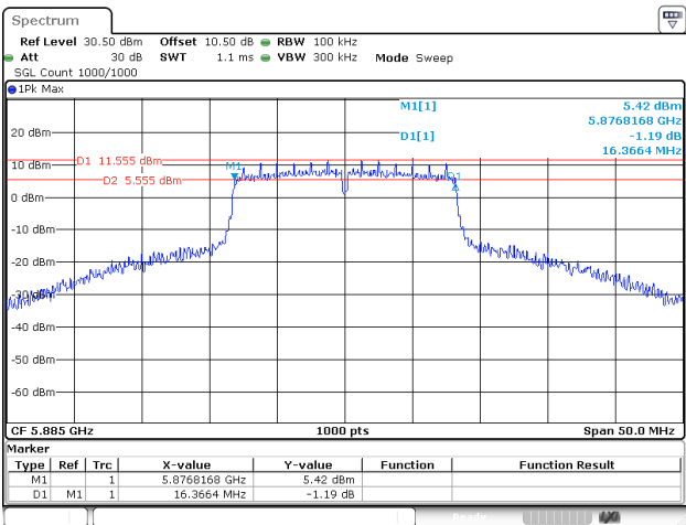
802.11a_5885MHz_Chain 2
