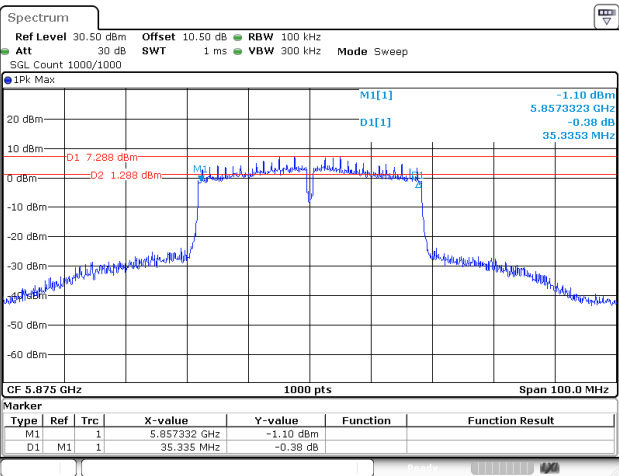
802.11ac40_5875MHz_Chain 2
