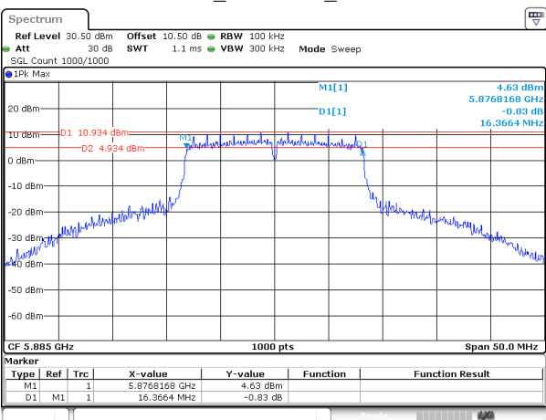
802.11a_5885MHz_Chain 1
