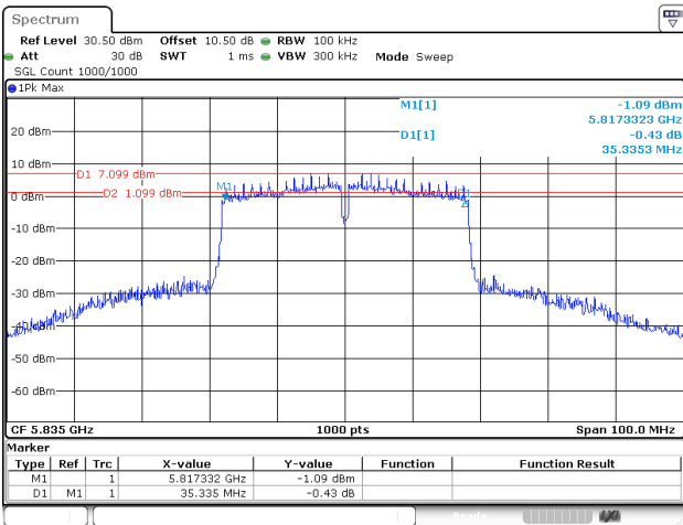
802.11ac40_5835MHz_Chain 2
