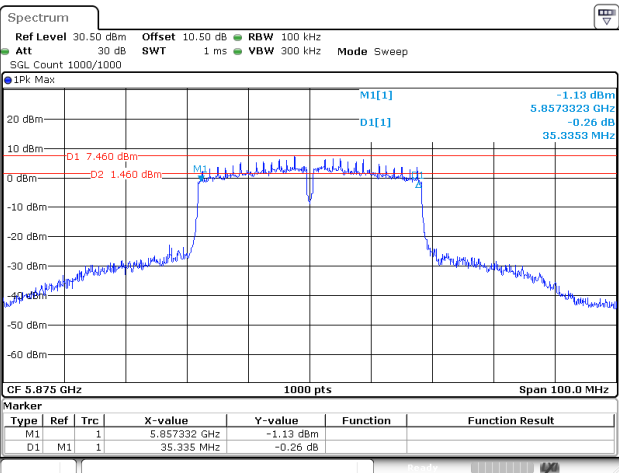
802.11ac40_5875MHz_Chain 0
