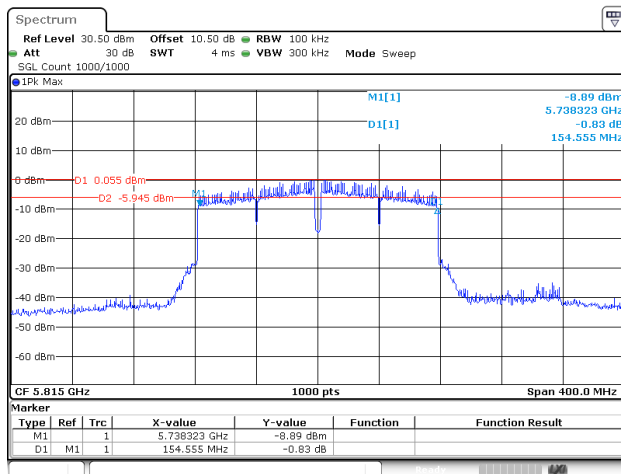
802.11ac160_5815MHz_Chain 1
