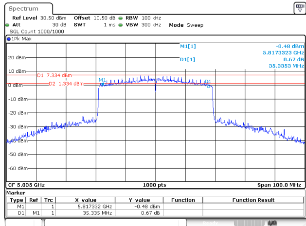
802.11be40_5835MHz_RU_Full_Chain 2
