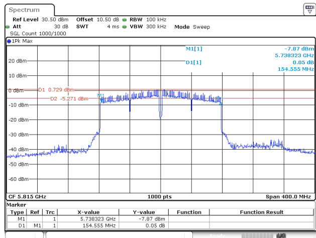
802.11ac160_5815MHz_Chain 2
