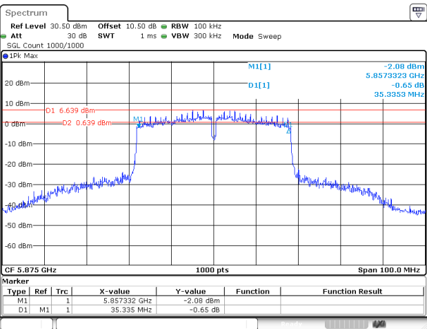
802.11ac40_5875MHz_Chain 1
