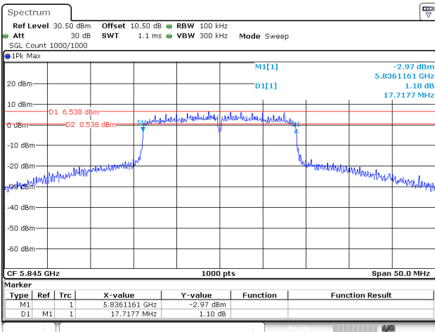
802.11ac20_5845MHz_Chain 1
