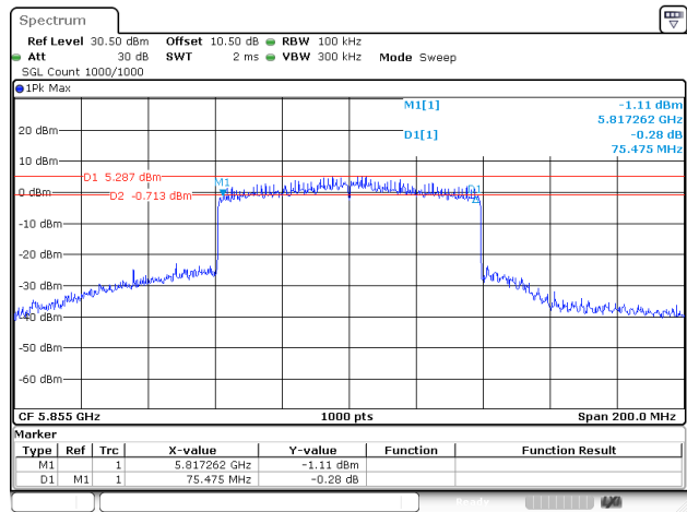
802.11be80_5855MHz_RU_Full_Chain 0
