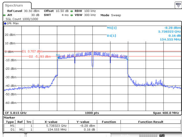
802.11ac160_5815MHz_Chain 0
