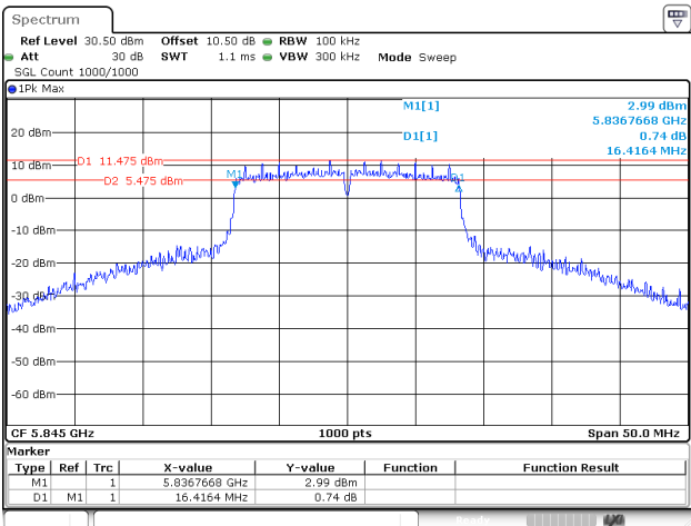
802.11a_5845MHz_Chain 2
