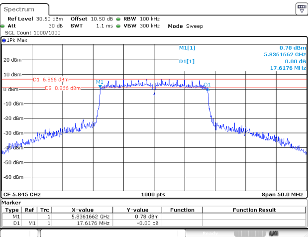
802.11ac20_5845MHz_Chain 2
