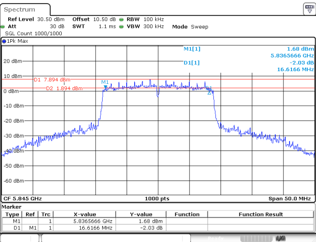
802.11ac20_5845MHz_Chain 0
