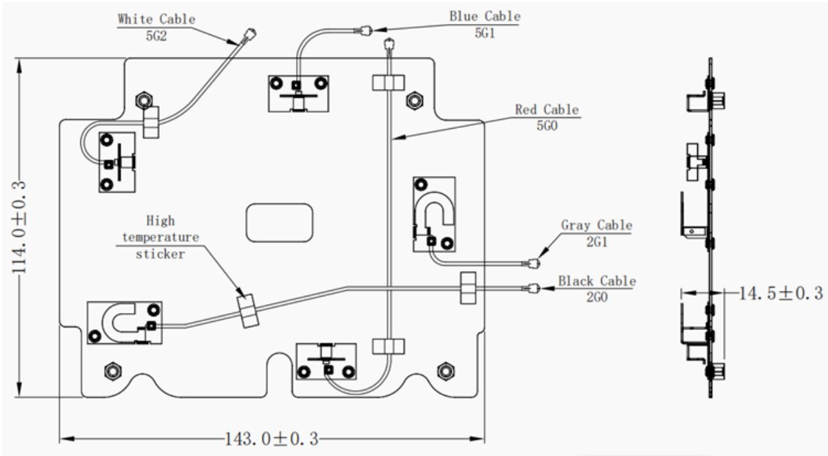
总成图 Mechanical Drawing(unit:mm)
