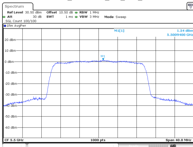
802.11be20_5500MHz_RU_Full_Chain 1
