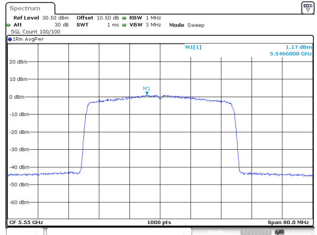
802.11be40_5550MHz_RU_Full_Chain 0
