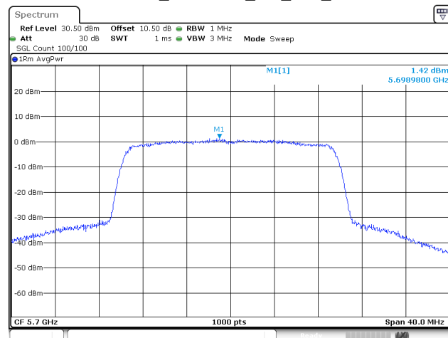
802.11be20_5700MHz_RU_Full_Chain 2
