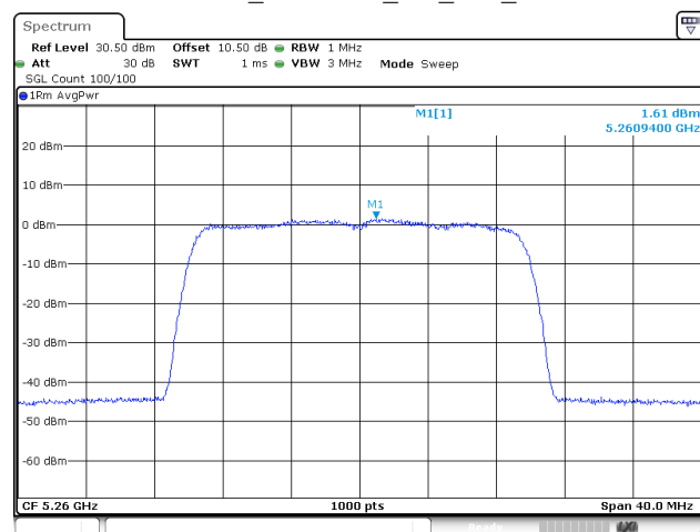
802.11be20_5260MHz_RU_Full_Chain 1
