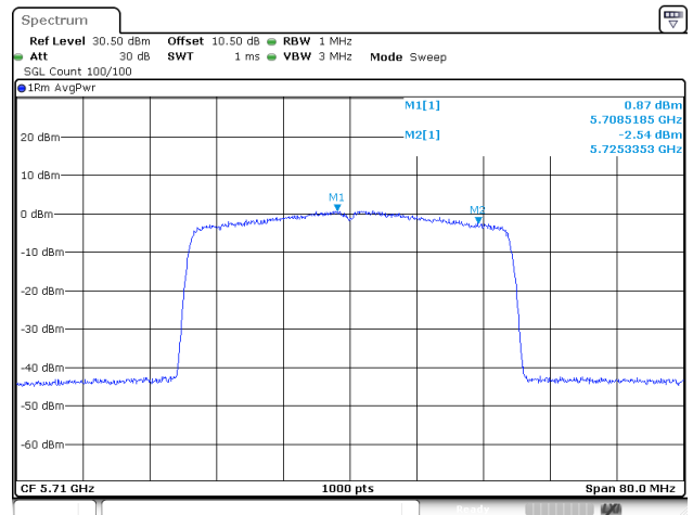
802.11be40_5710MHz_RU_Full_Chain 0
