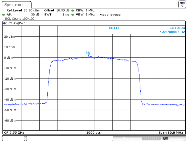
802.11be40_5550MHz_RU_Full_Chain 2
