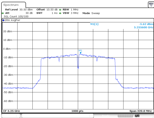
802.11ac160_5250MHz_Chain 0
