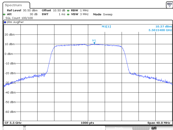
802.11a_5500MHz_Chain 0
