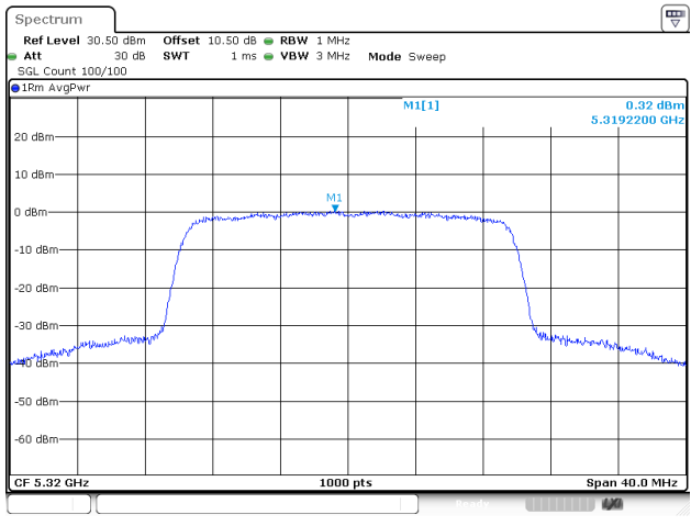
802.11be20_5320MHz_RU_Full_Chain 0
