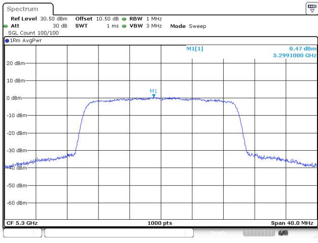
802.11be20_5300MHz_RU_Full_Chain 0
