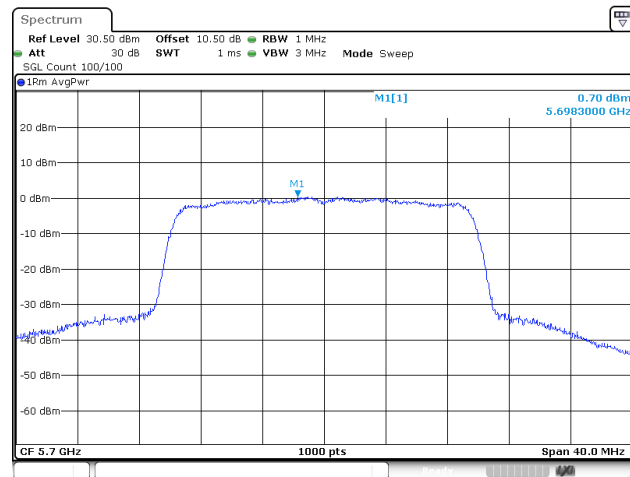
802.11be20_5700MHz_RU_Full_Chain 1
