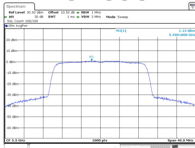
802.11be20_5500MHz_RU_Full_Chain 2
