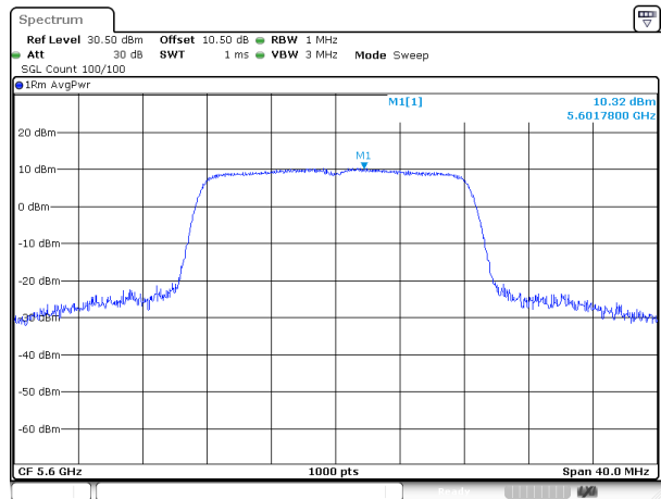
802.11a_5600MHz_Chain 0
