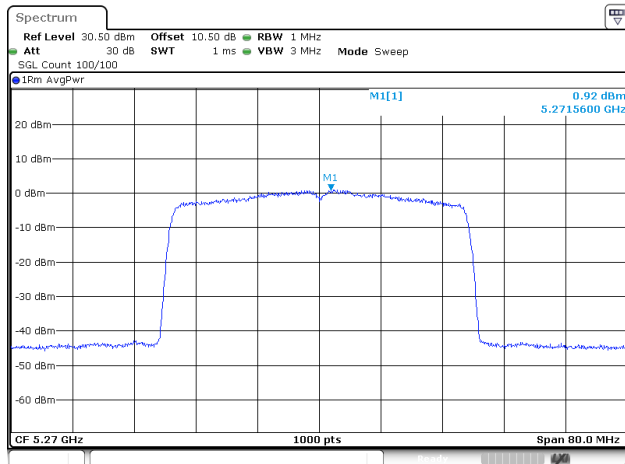
802.11be40_5270MHz_RU_Full_Chain 2
