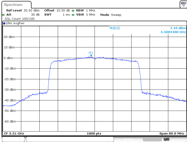
802.11be40_5510MHz_RU_Full_Chain 2
