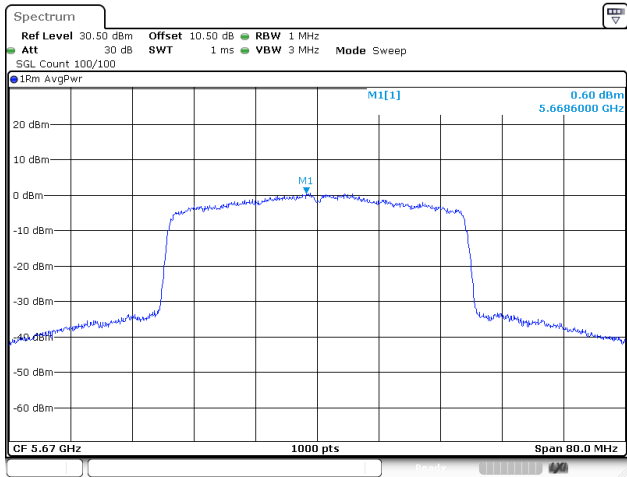
802.11be40_5670MHz_RU_Full_Chain 1
