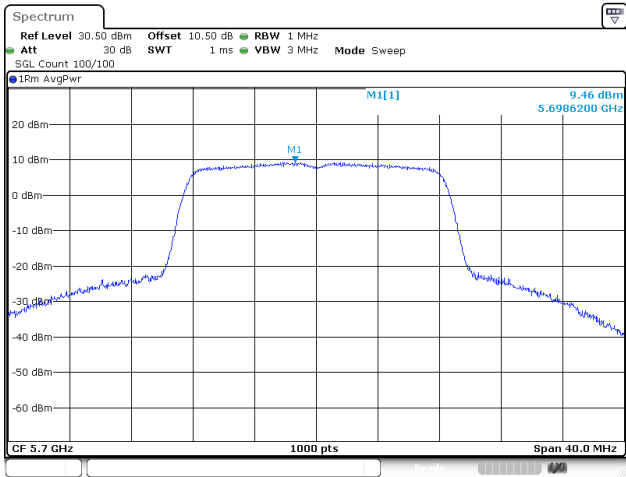
802.11a_5700MHz_Chain 1
