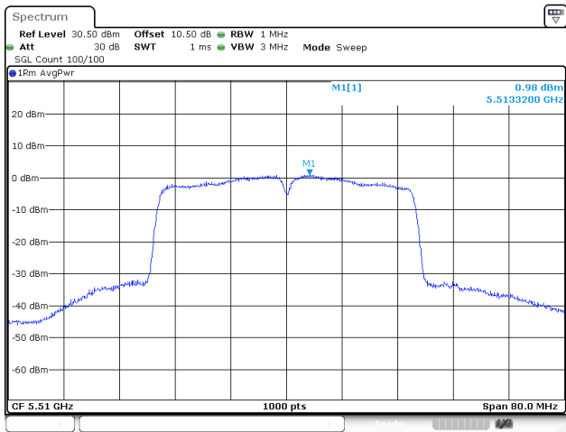
802.11ac40_5510MHz_Chain 2
