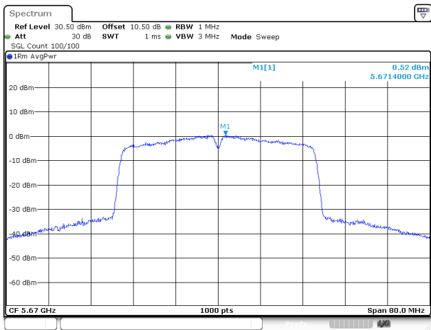
802.11ac40_5670MHz_Chain 1
