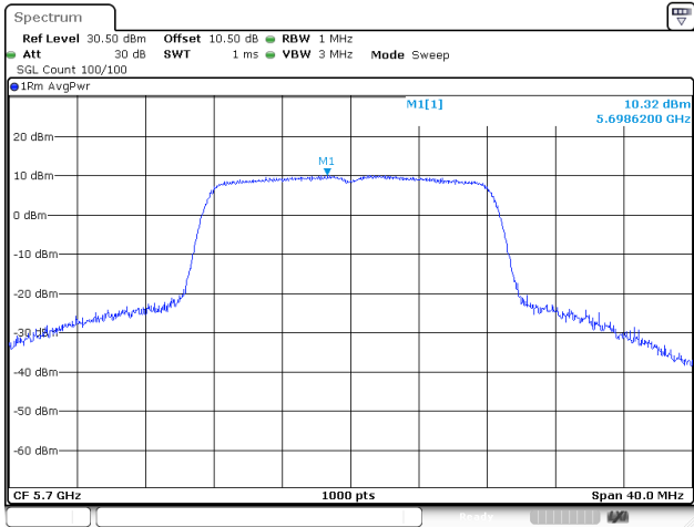
802.11a_5700MHz_Chain 2
