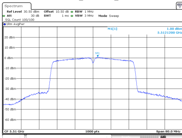
802.11ac40_5510MHz_Chain 1
