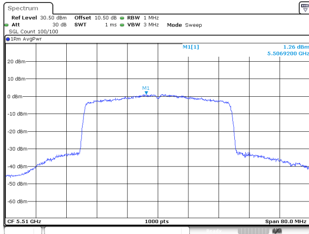
802.11be40_5510MHz_RU_Full_Chain 0
