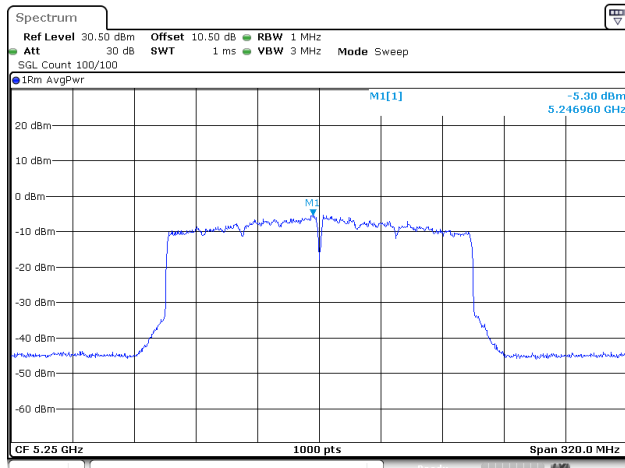
802.11be160_5250MHz_RU_FULL_Chain 1
