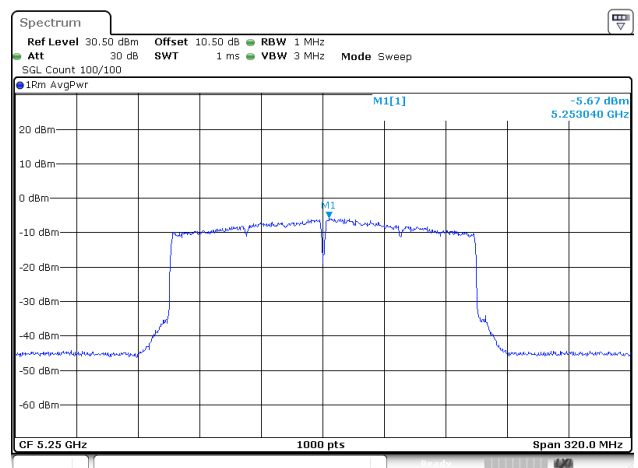
802.11be160_5250MHz_RU_FULL_Chain 2
