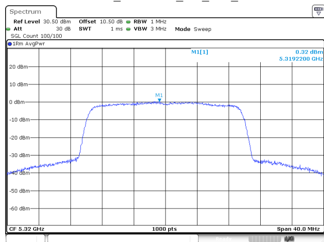
802.11be20_5320MHz_RU_Full_Chain 2
