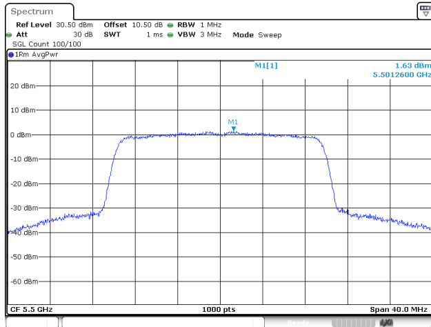
802.11be20_5500MHz_RU_Full_Chain 0
