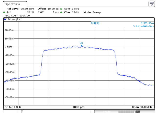
802.11be40_5310MHz_RU_Full_Chain 0
