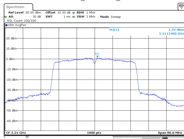
802.11ac40_5310MHz_Chain 1
