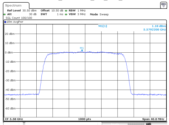
802.11be20_5580MHz_RU_Full_Chain 1
