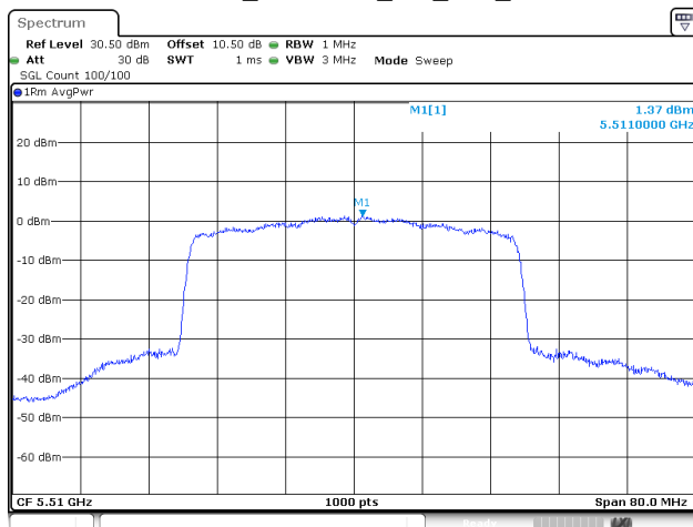
802.11be40_5510MHz_RU_Full_Chain 1
