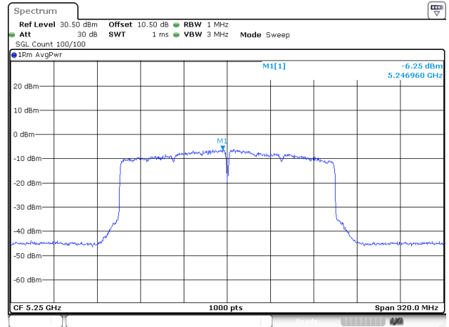
802.11be160_5250MHz_RU_FULL_Chain 0
