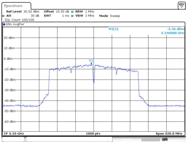
802.11ac160_5250MHz_Chain 1
