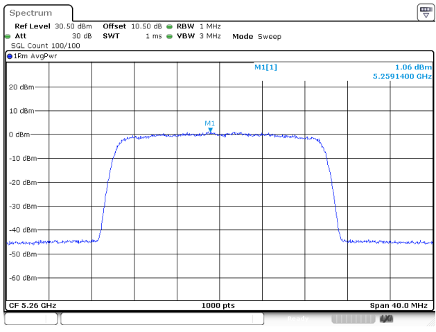
802.11be20_5260MHz_RU_Full_Chain 0
