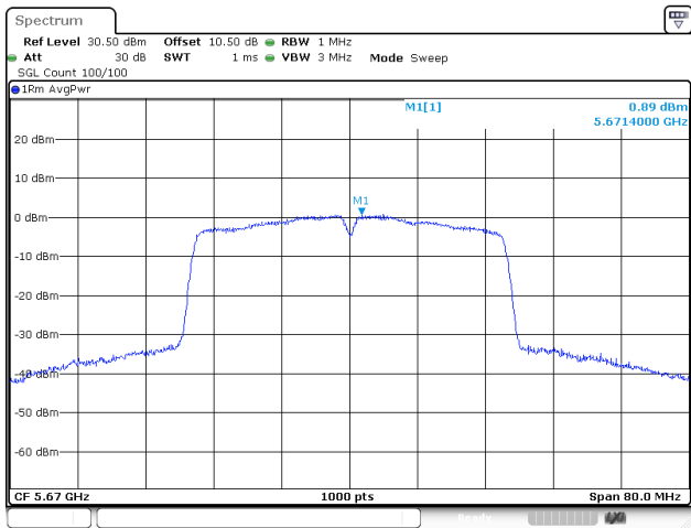
802.11ac40_5670MHz_Chain 2
