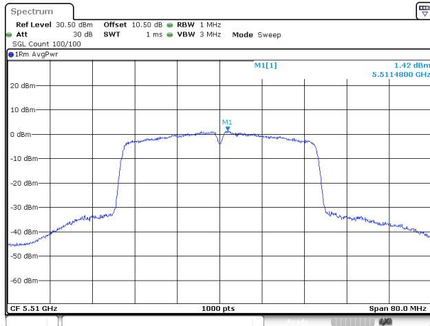
802.11ac40_5510MHz_Chain 0
