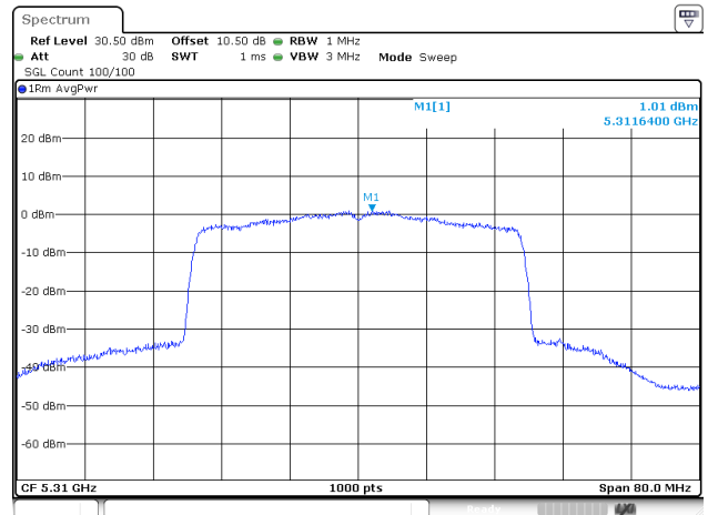
802.11be40_5310MHz_RU_Full_Chain 2
