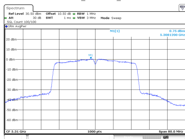
802.11ac40_5310MHz_Chain 2
