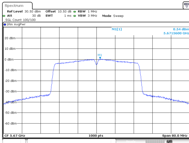
802.11ac40_5670MHz_Chain 0
