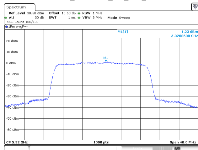
802.11be20_5320MHz_RU_Full_Chain 1
