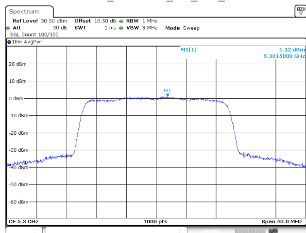
802.11be20_5300MHz_RU_Full_Chain 1
