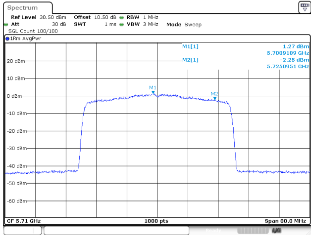
802.11be40_5710MHz_RU_Full_Chain 2
