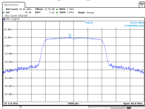
802.11a_5600MHz_Chain 1
