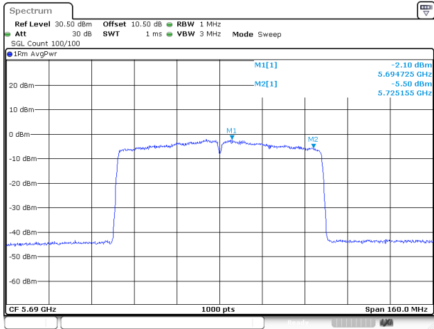
802.11ac80_5690MHz_Chain 2
