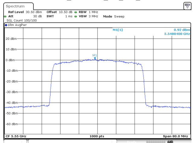
802.11be40_5550MHz_RU_Full_Chain 1
