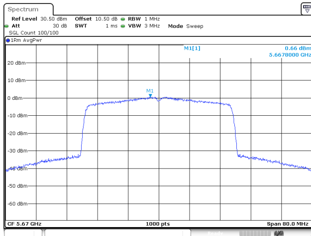
802.11be40_5670MHz_RU_Full_Chain 0
