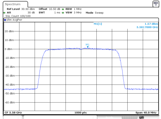
802.11be20_5580MHz_RU_Full_Chain 0
