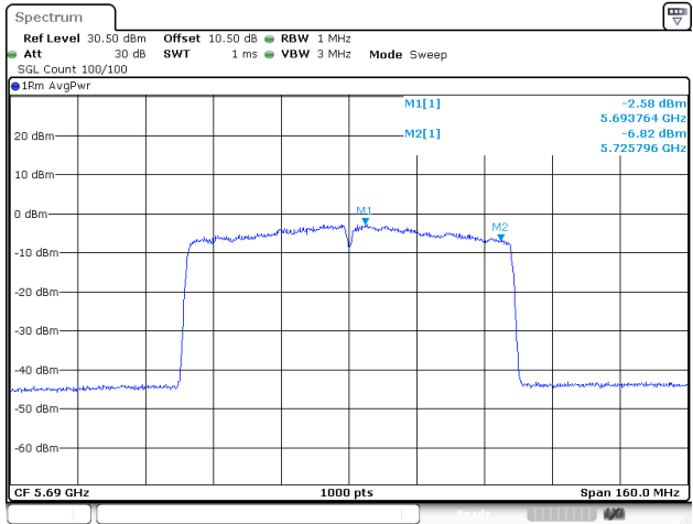
802.11ac80_5690MHz_Chain 1
