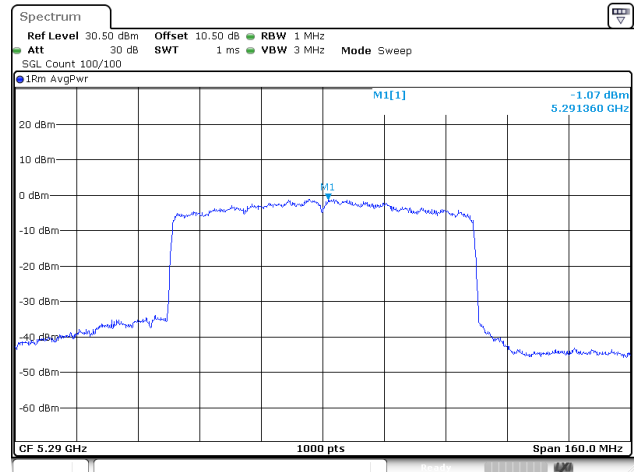
802.11be80_5290MHz_RU_Full_Chain 1
