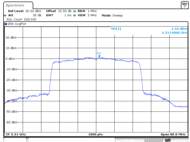
802.11be40_5310MHz_RU_Full_Chain 1
