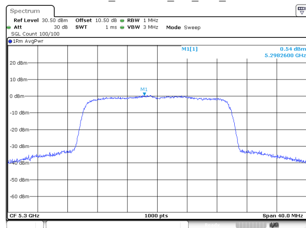
802.11be20_5300MHz_RU_Full_Chain 2
