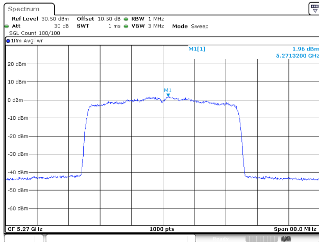
802.11be40_5270MHz_RU_Full_Chain 1
