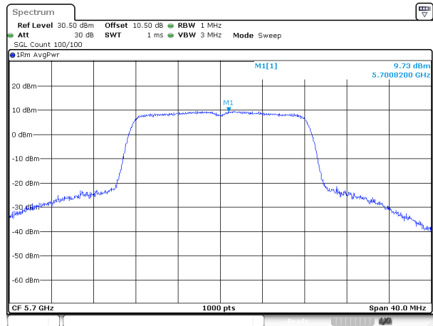
802.11a_5700MHz_Chain 0
