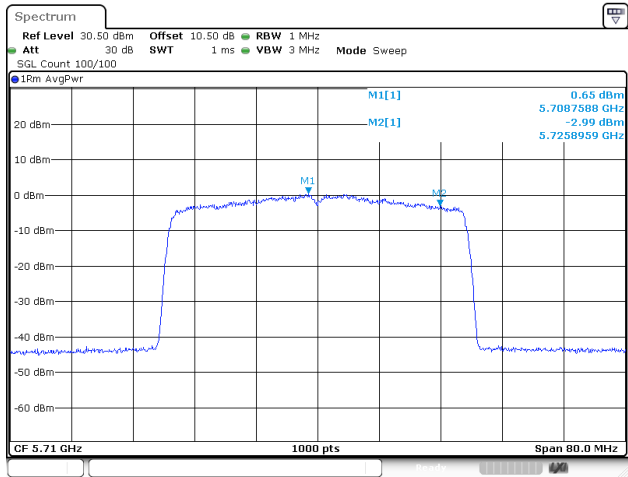
802.11be40_5710MHz_RU_Full_Chain 1
