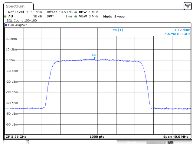
802.11be20_5580MHz_RU_Full_Chain 2
