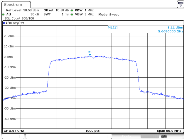
802.11be40_5670MHz_RU_Full_Chain 2
