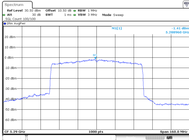
802.11be80_5290MHz_RU_Full_Chain 2
