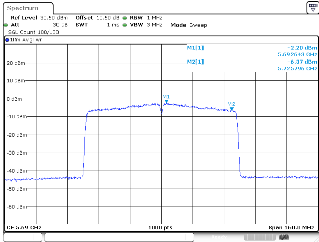
802.11ac80_5690MHz_Chain 0
