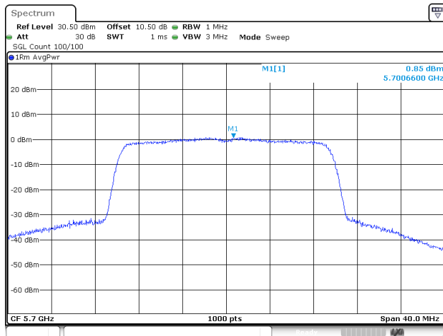
802.11be20_5700MHz_RU_Full_Chain 0
