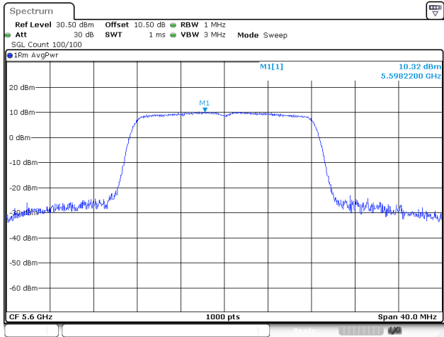
802.11a_5600MHz_Chain 2
