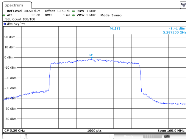
802.11be80_5290MHz_RU_Full_Chain 0
