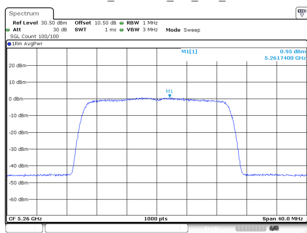
802.11be20_5260MHz_RU_Full_Chain 2
