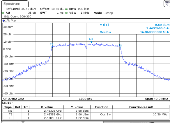
802.11g_2462MHz_Chain 0
