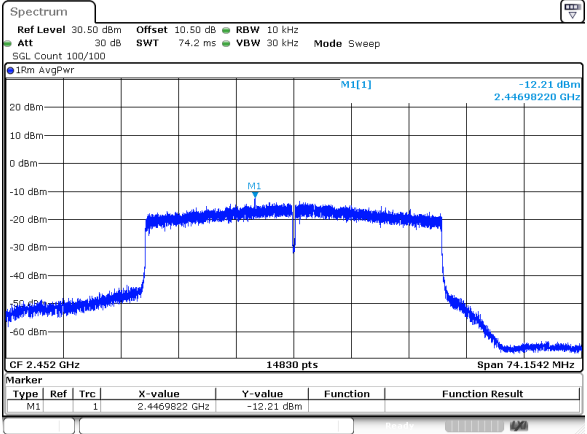
802.11be40_RU_Full_2452MHz_Chain 1
