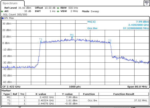
802.11be40_RU_Full_2422MHz_Chain 1
