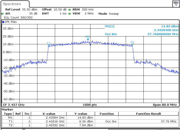
802.11be40_RU_Full_2437MHz_Chain 0
