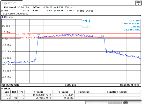
802.11be40_RU_Full_2422MHz_Chain 1
