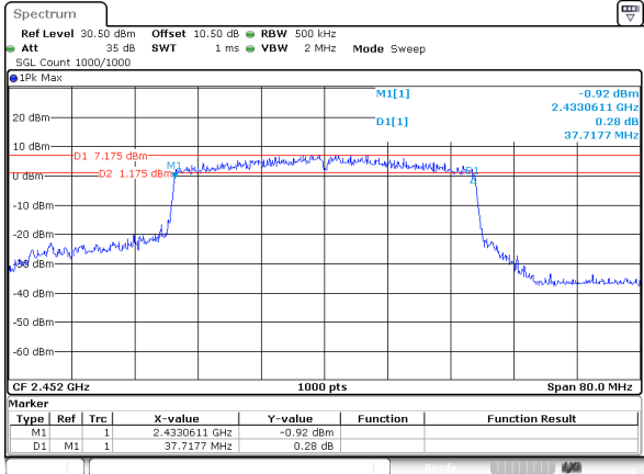
802.11be40_RU_Full_2452MHz_Chain 0
