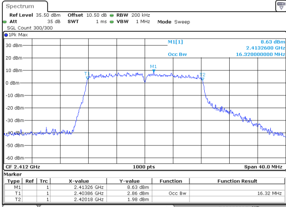
802.11g_2412MHz_Chain 0
