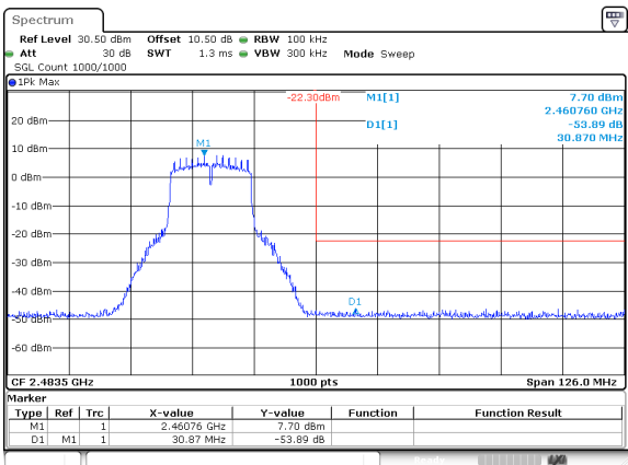
802.11g_2462MHz_Chain 1
