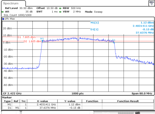
802.11be40_RU_Full_2422MHz_Chain 0
