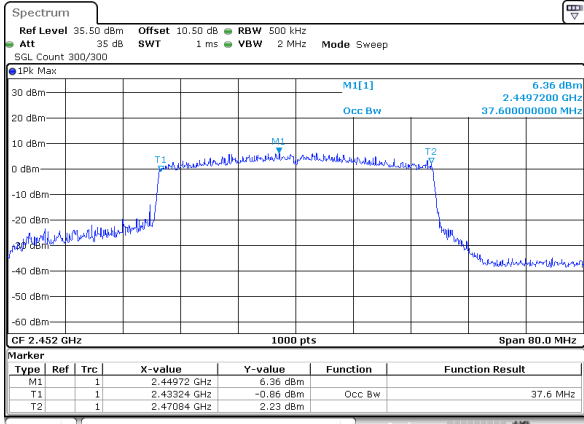
802.11be40_RU_Full_2452MHz_Chain 0
