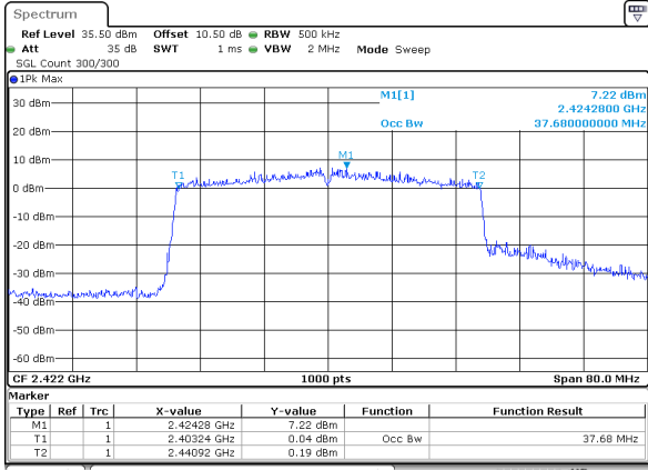
802.11be40_RU_Full_2422MHz_Chain 0
