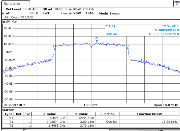
802.11g_2437MHz_Chain 1
