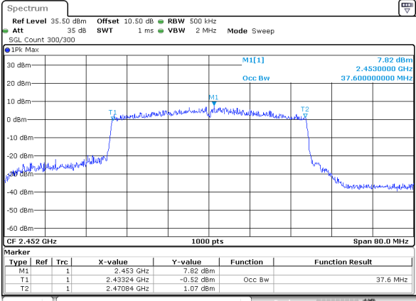
802.11be40_RU_Full_2452MHz_Chain 1
