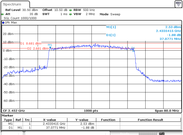
802.11be40_RU_Full_2452MHz_Chain 1
