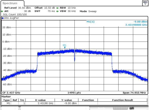
802.11be40_RU_Full_2437MHz_Chain 0
