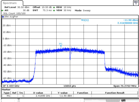
802.11be40_RU_Full_2422MHz_Chain 0
