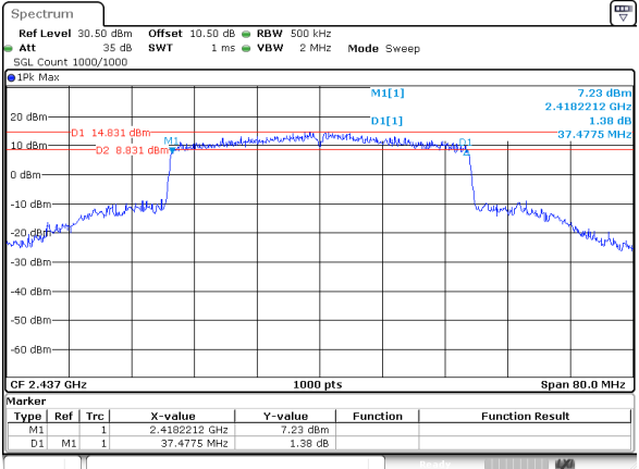
802.11be40_RU_Full_2437MHz_Chain 0
