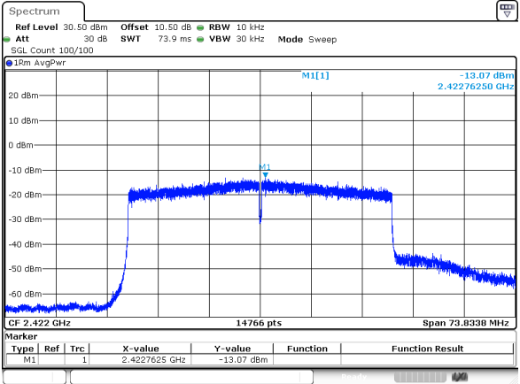
802.11be40_RU_Full_2422MHz_Chain 1
