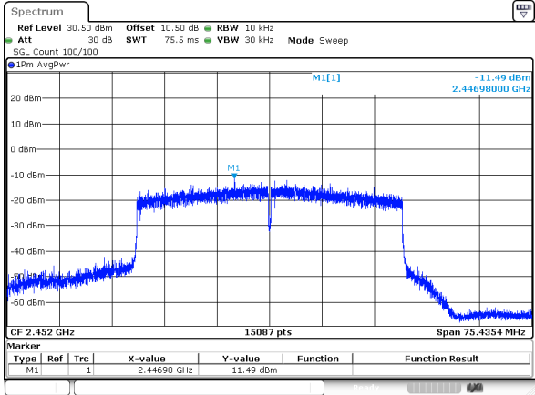
802.11be40_RU_Full_2452MHz_Chain 0
