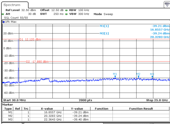
802.11g_2412MHz_Chain 0
