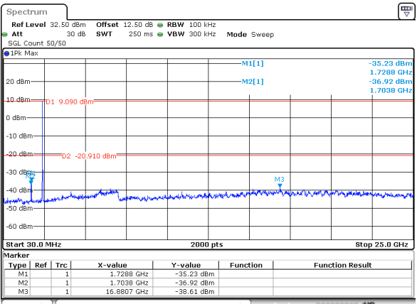
802.11g_2412MHz_Chain 1
