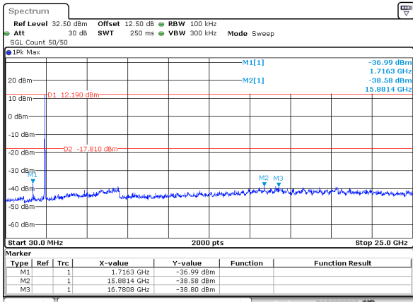
802.11g_2437MHz_Chain 1
