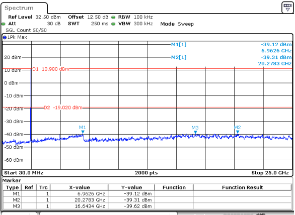
802.11g_2462MHz_Chain 1
