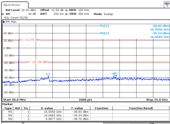
802.11g_2462MHz_Chain 0
