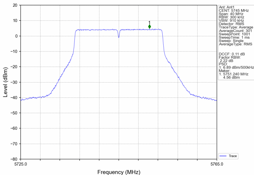
802.11ac(VHT20)_LCH_5745MHz_Ant1_NTNV
