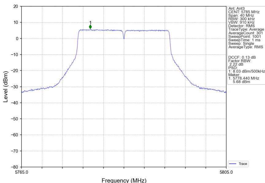
802.11n(HT20)_MCH_5785MHz_Ant3_NTNV
