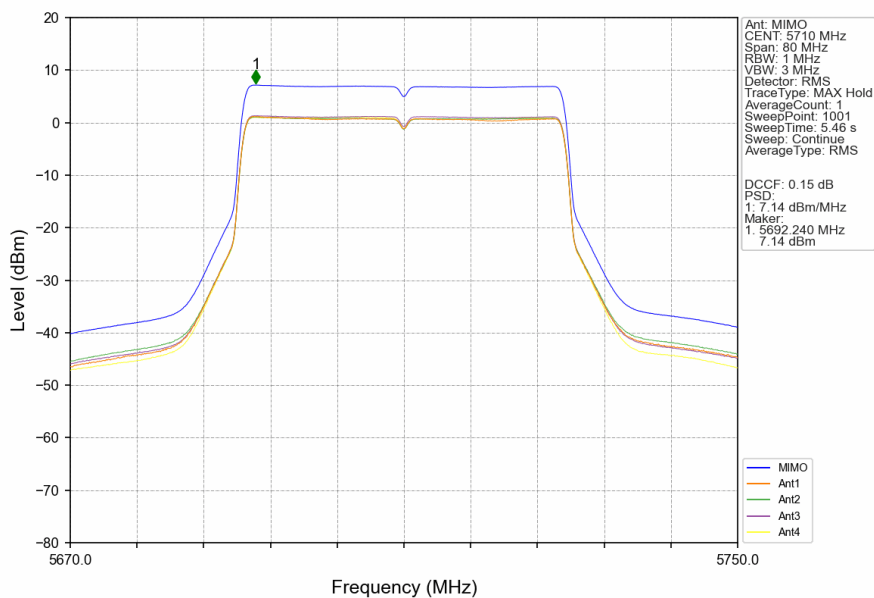
802.11be(EHT40)_HCH_5710MHz_SU_/_MIMO_NTNV
