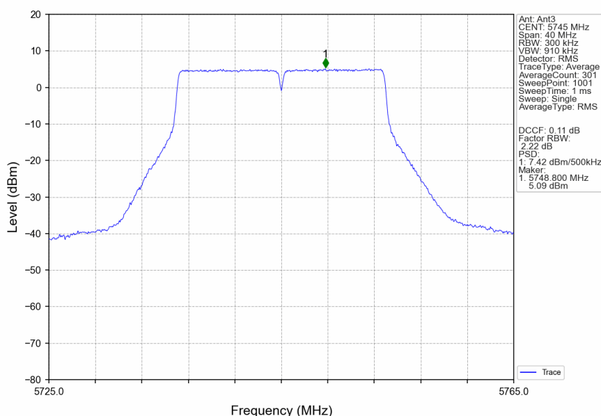
802.11ac(VHT20)_LCH_5745MHz_Ant3_NTNV
