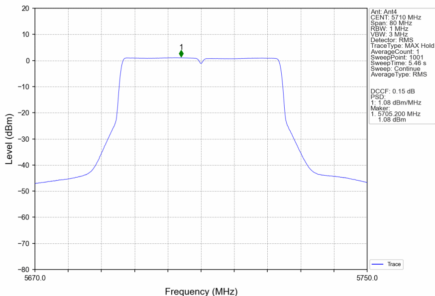
802.11be(EHT40)_HCH_5710MHz_SU_/_MIMO_NTNV
