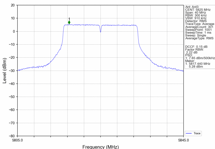
802.11ac(VHT20)_HCH_5825MHz_Ant3_NTNV
