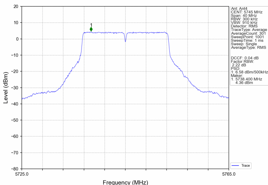
802.11a_LCH_5745MHz_Ant4_NTNV
