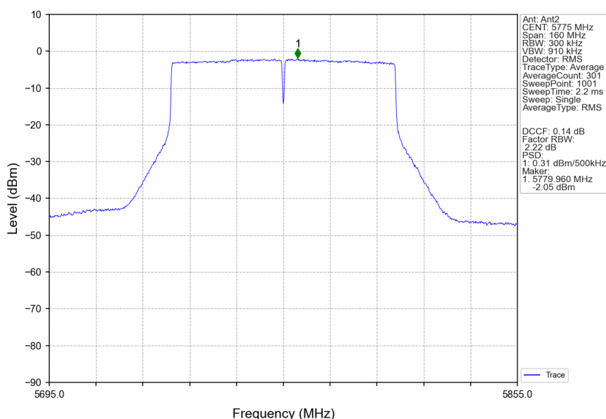
802.11ac(VHT80)_MCH_5775MHz_Ant2_NTNV
