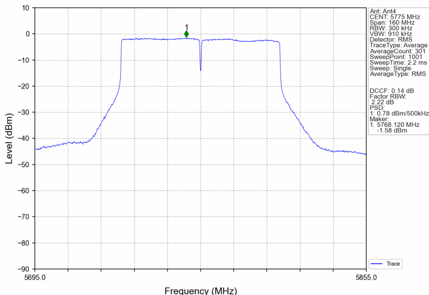
802.11ac(VHT80)_MCH_5775MHz_Ant4_NTNV
