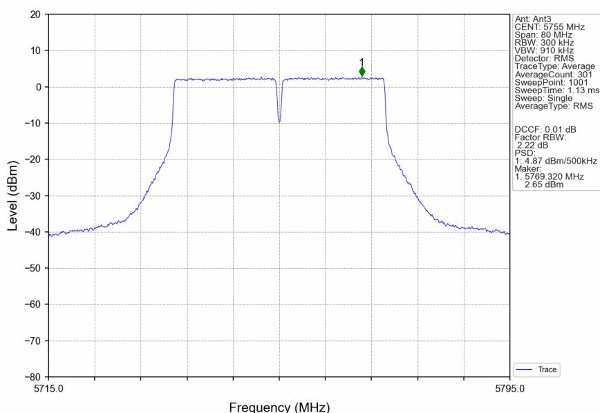
802.11ac(VHT40)_LCH_5755MHz_Ant3_NTNV
