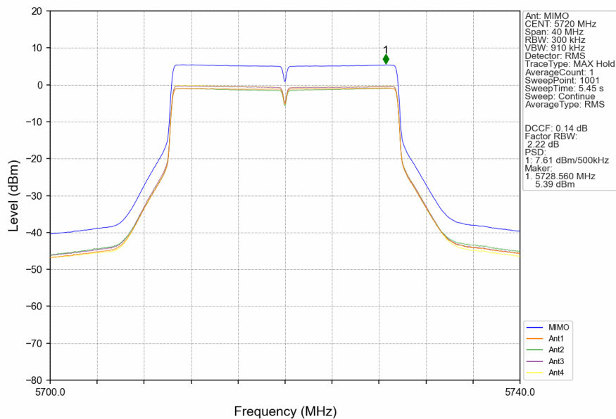
802.11ax(HEW20)_HCH_5720MHz_SU_/_MIMO_NTNV
