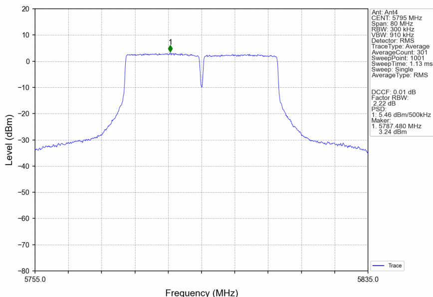
802.11ac(VHT40)_HCH_5795MHz_Ant4_NTNV
