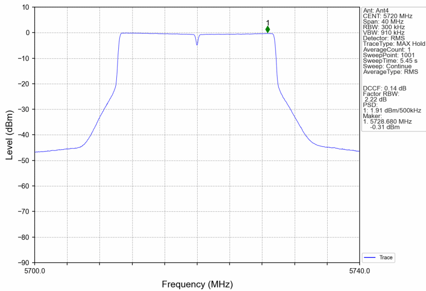
802.11ax(HEW20)_HCH_5720MHz_SU_/_MIMO_NTNV
