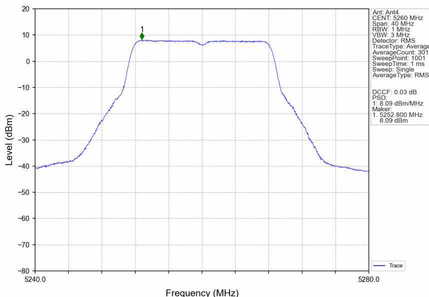
802.11a_LCH_5260MHz_Ant4_NTNV
