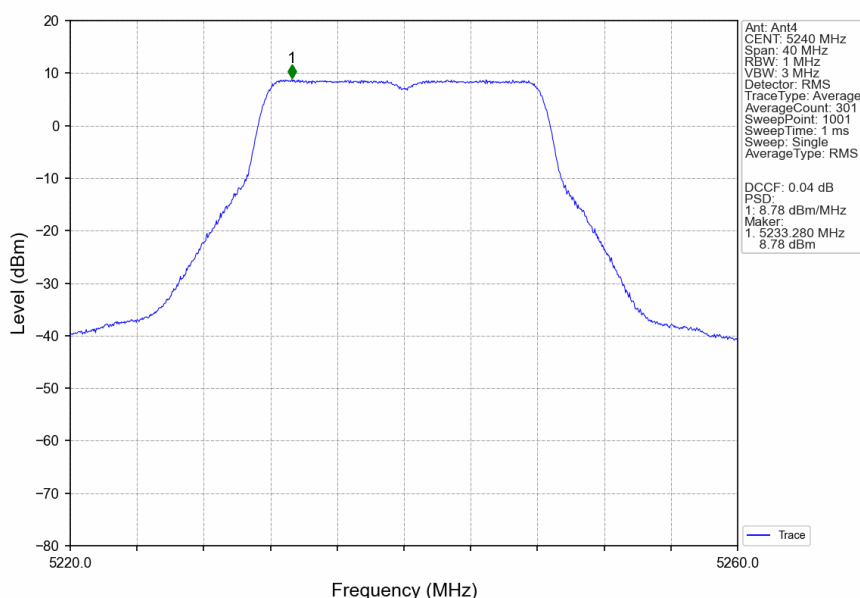
802.11a_HCH_5240MHz_Ant4_NTNV
