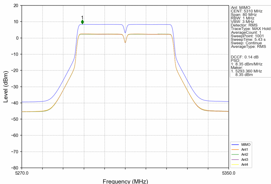
802.11n(HT40)_HCH_5310MHz_MIMO_NTNV
