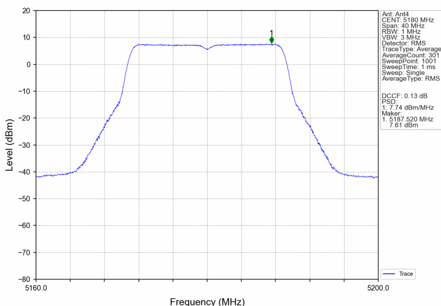
802.11ac(VHT20)_LCH_5180MHz_Ant4_NTNV
