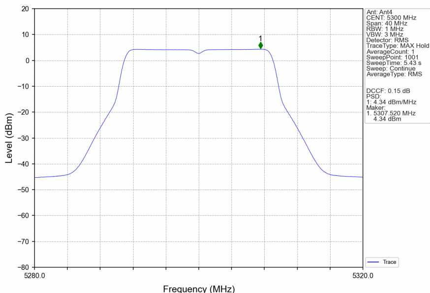
802.11n(HT20)_MCH_5300MHz_Ant4_NTNV
