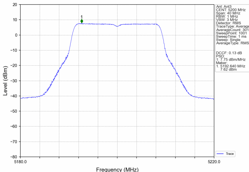
802.11ac(VHT20)_MCH_5200MHz_Ant3_NTNV
