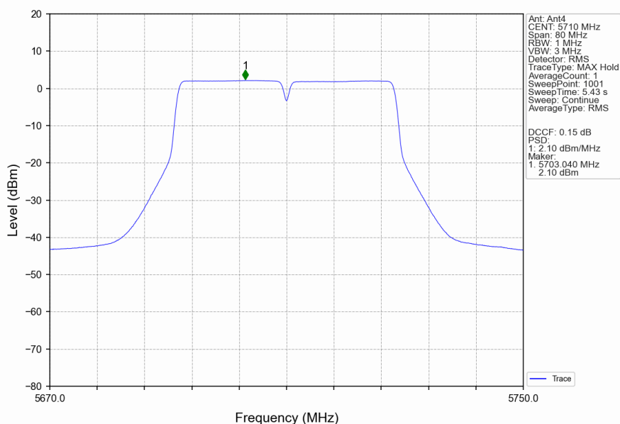
802.11n(HT40)_HCH_5710MHz_MIMO_NTNV
