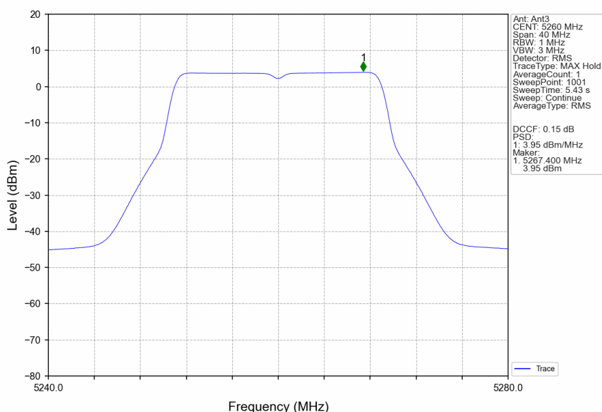
802.11n(HT20)_LCH_5260MHz_Ant3_NTNV
