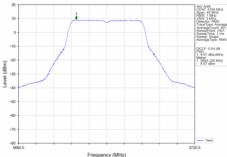
802.11a_HCH_5700MHz_Ant4_NTNV
