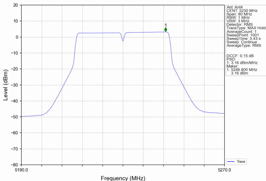
802.11n(HT40)_HCH_5230MHz_MIMO_NTNV
