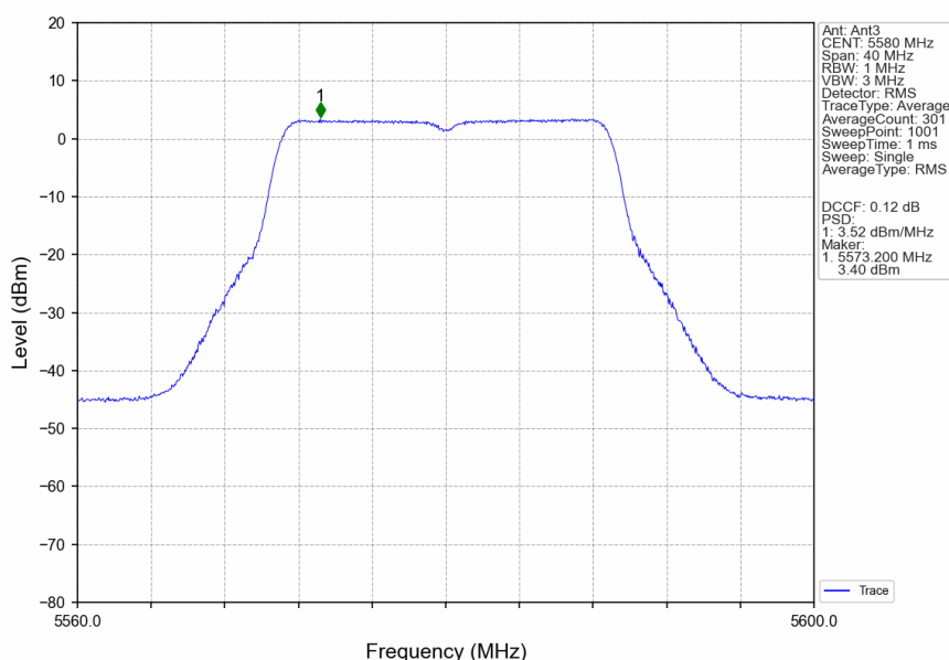
802.11n(HT20)_MCH_5580MHz_Ant3_NTNV
