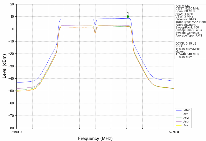
802.11n(HT40)_HCH_5230MHz_MIMO_NTNV
