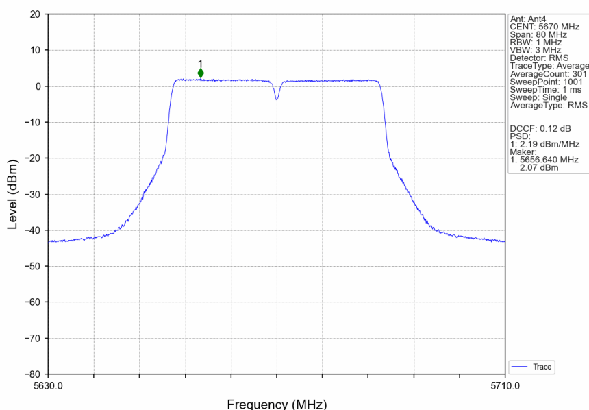
802.11n(HT40)_HCH_5670MHz_Ant4_NTNV
