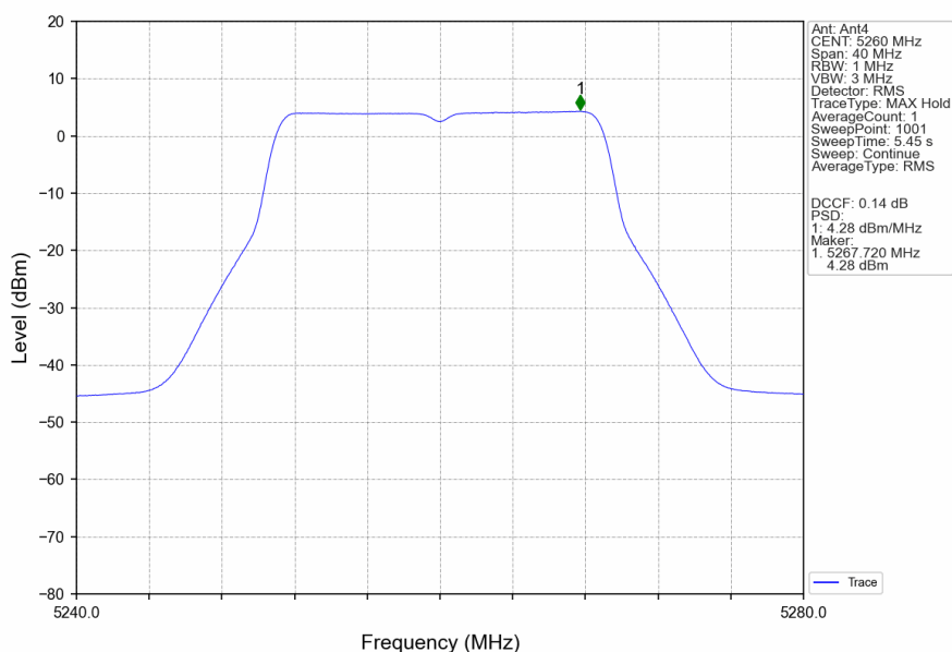
802.11ac(VHT20)_LCH_5260MHz_MIMO_NTNV
