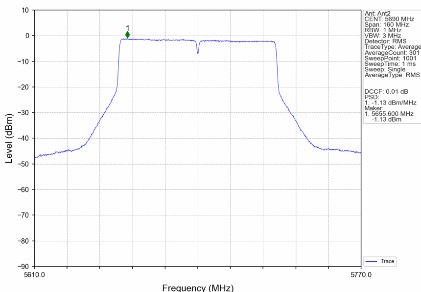
802.11ac(VHT80)_HCH_5690MHz_Ant2_NTNV
