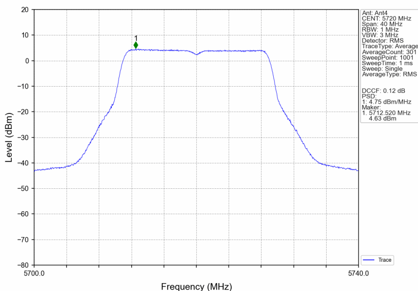
802.11ac(VHT20)_HCH_5720MHz_MIMO_NTNV
