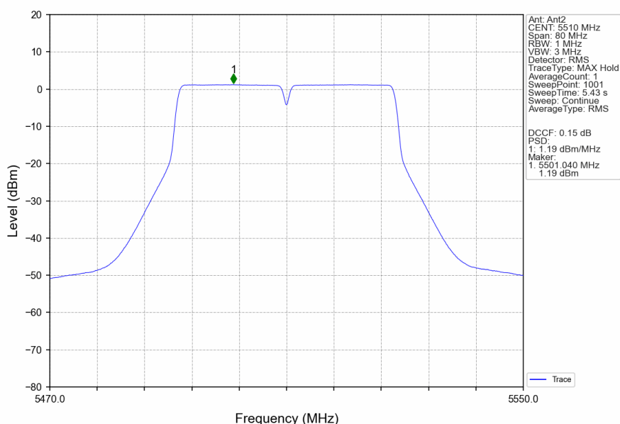
802.11ac(VHT40)_LCH_5510MHz_Ant2_NTNV
