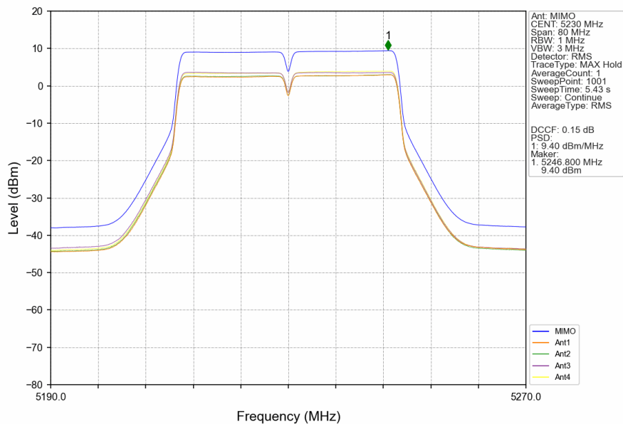
802.11ac(VHT40)_HCH_5230MHz_MIMO_NTNV
