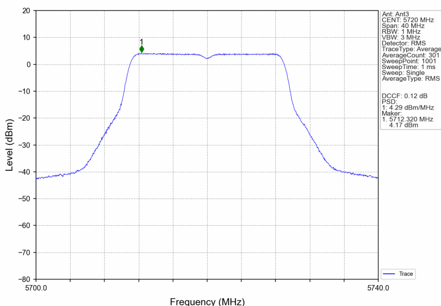
802.11ac(VHT20)_HCH_5720MHz_Ant3_NTNV
