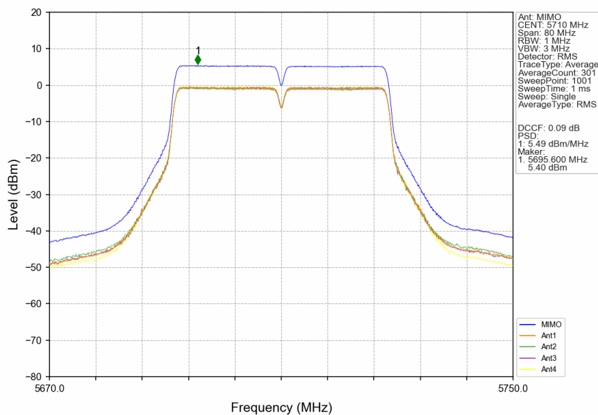
802.11ac(VHT40)_HCH_5710MHz_MIMO_NTNV
