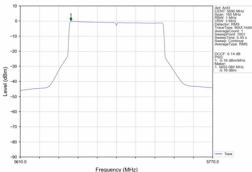
802.11ax(HEW80)_HCH_5690MHz_SU_/_Ant3_NTNV
