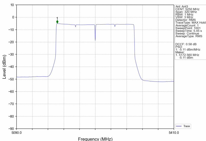
802.11ax(HEW160)_MCH_5250MHz_SU_/_Ant3_NTNV
