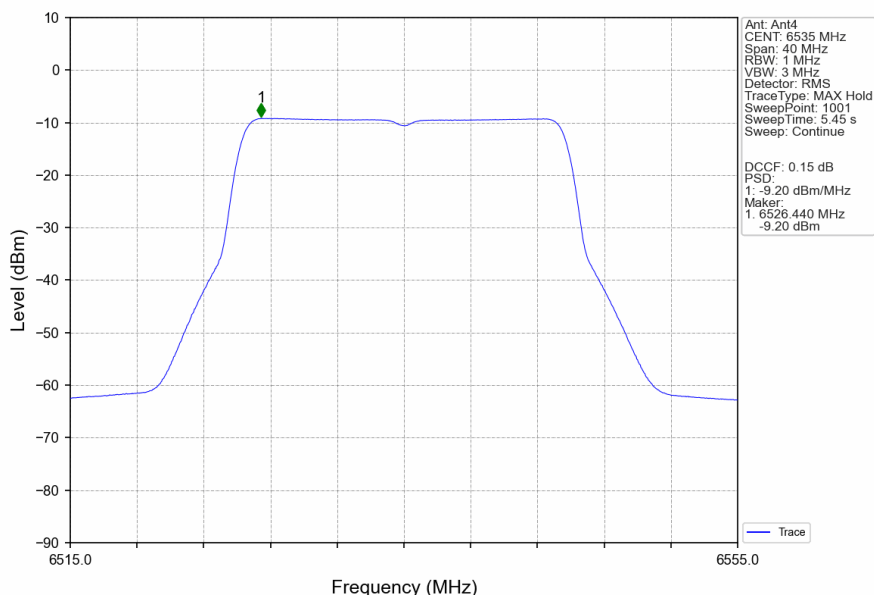
802.11ax(HEW20)_LCH_6535MHz_RU242_Left_Ant4_NTNV
