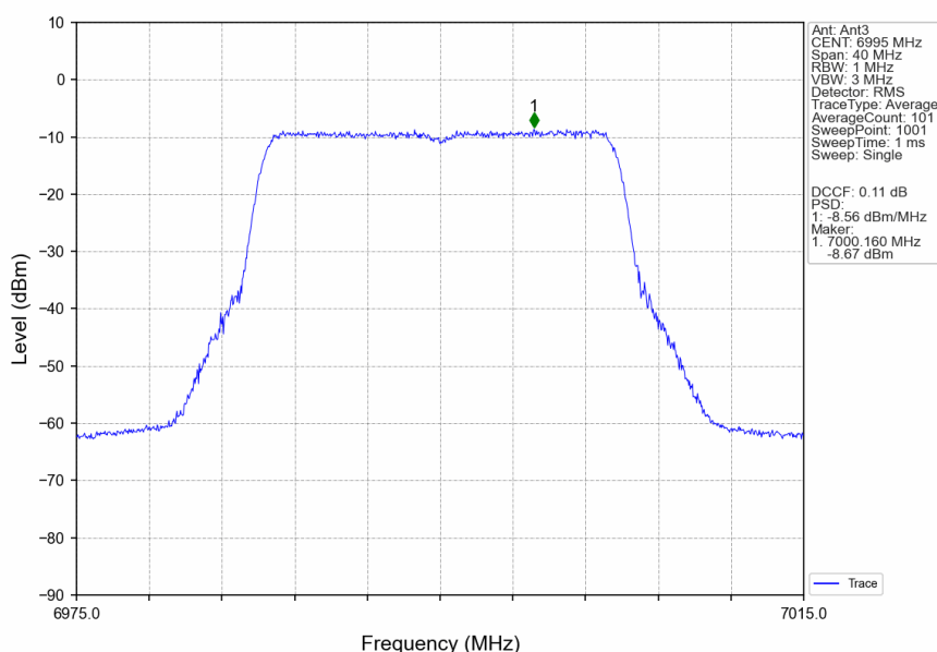
802.11ax(HEW20)_MCH_6995MHz_RU242_Left_Ant3_NTNV
