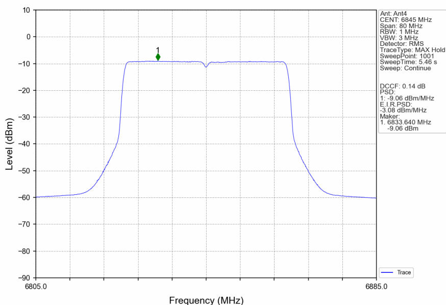
802.11ax(HEW40)_HCH_6845MHz_RU484_Left_MIMO_NTNV
