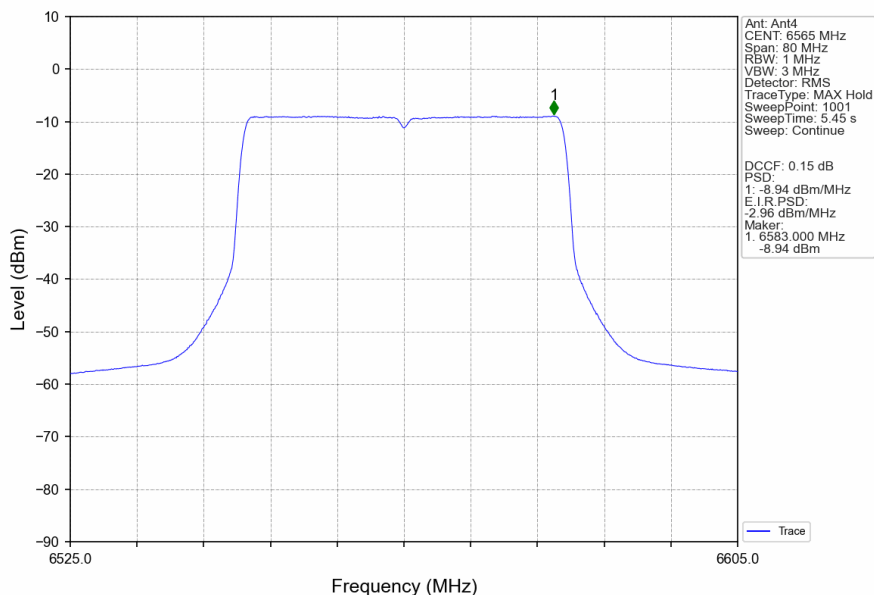
802.11ax(HEW40)_LCH_6565MHz_RU484_Left_MIMO_NTNV
