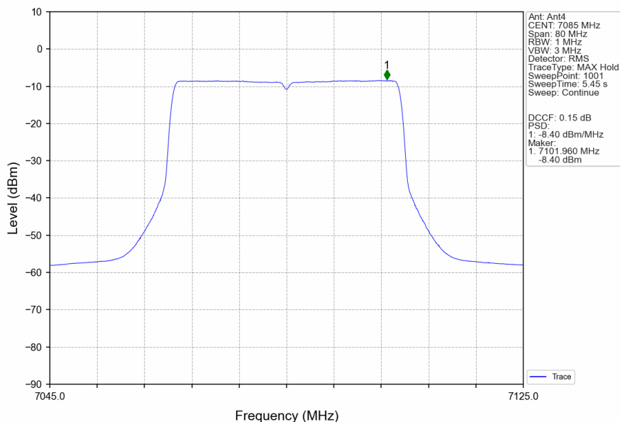
802.11ax(HEW40)_HCH_7085MHz_RU484_Left_MIMO_NTNV
