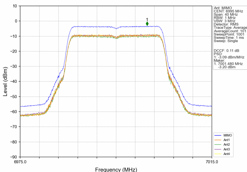
802.11ax(HEW20)_MCH_6995MHz_RU242_Left_MIMO_NTNV
