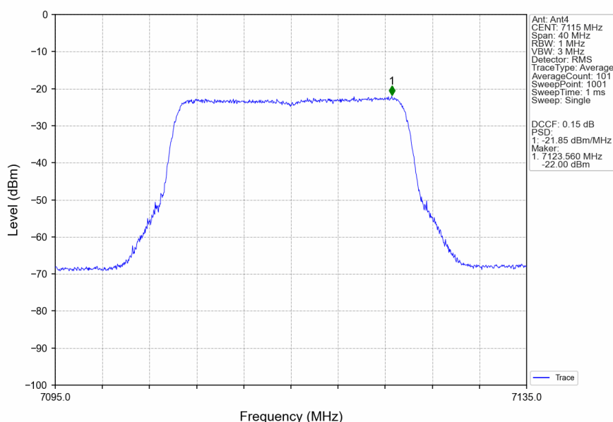
802.11ax(HEW20)_HCH_7115MHz_RU242_Left_Ant4_NTNV
