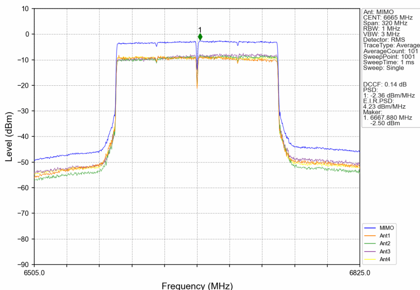
802.11ax(HEW160)_MCH_6665MHz_2xRU996_Left_MIMO_NTNV
