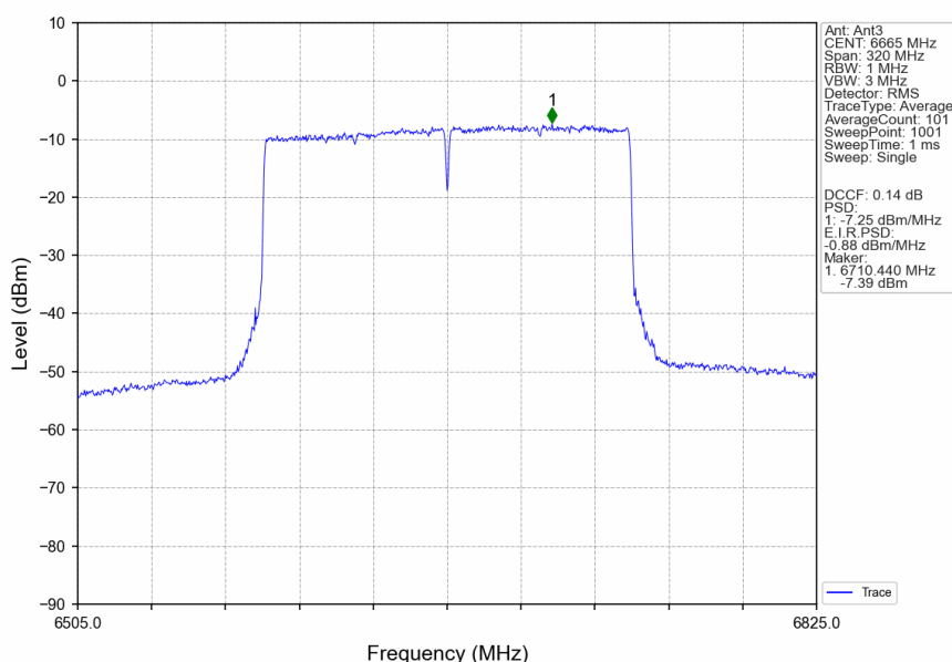
802.11ax(HEW160)_MCH_6665MHz_2xRU996_Left_Ant3_NTNV
