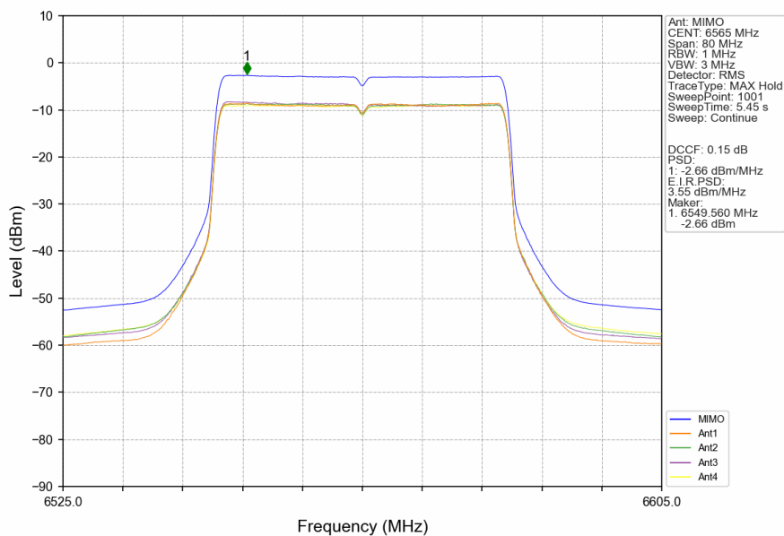
802.11ax(HEW40)_LCH_6565MHz_RU484_Left_MIMO_NTNV
