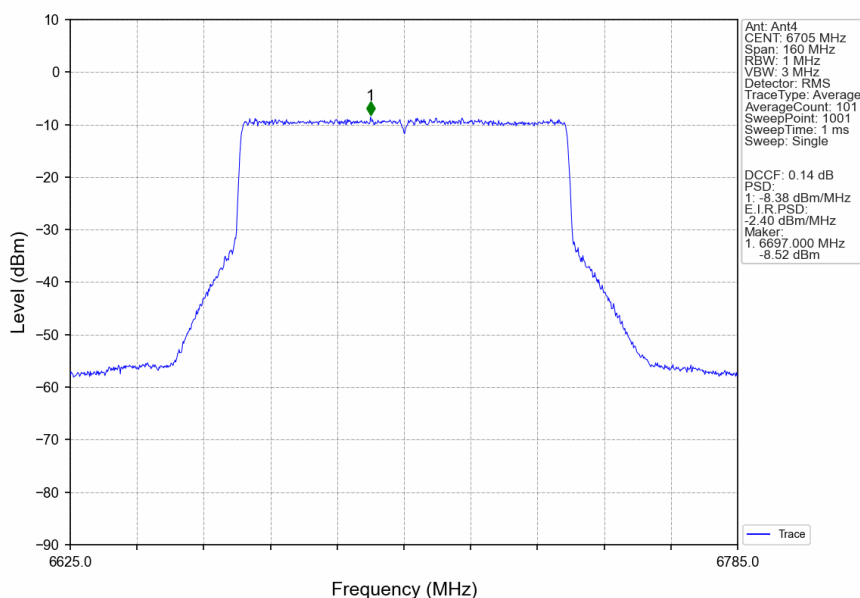
802.11ax(HEW80)_MCH_6705MHz_RU996_Left_MIMO_NTNV
