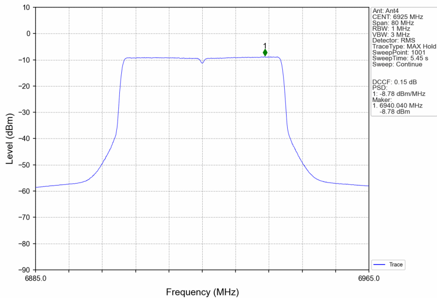
802.11ax(HEW40)_LCH_6925MHz_RU484_Left_MIMO_NTNV
