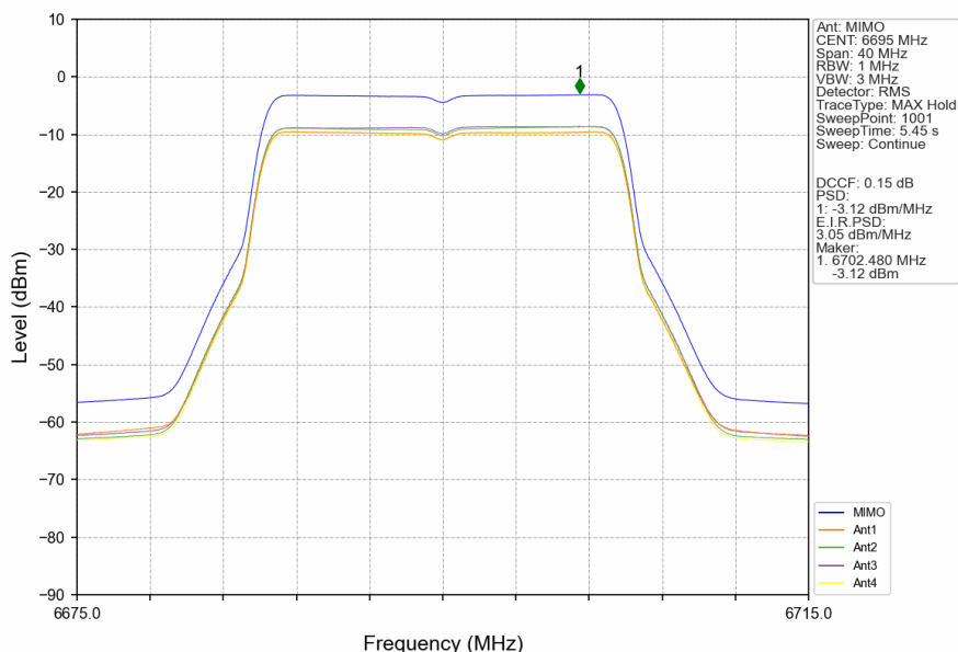
802.11ax(HEW20)_MCH_6695MHz_RU242_Left_MIMO_NTNV
