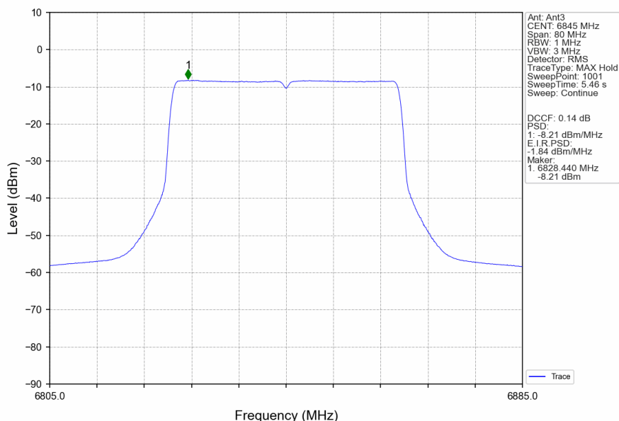
802.11ax(HEW40)_HCH_6845MHz_RU484_Left_Ant3_NTNV
