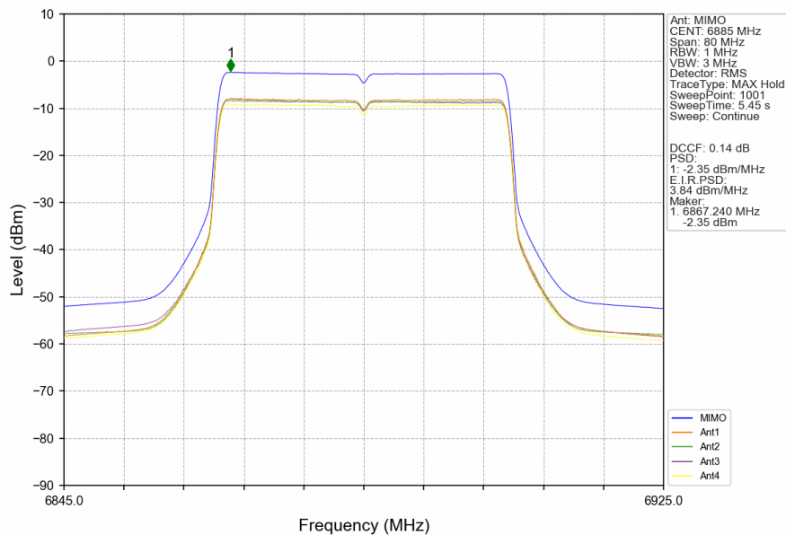
802.11ax(HEW40)_HCH_6885MHz_RU484_Left_MIMO_NTNV
