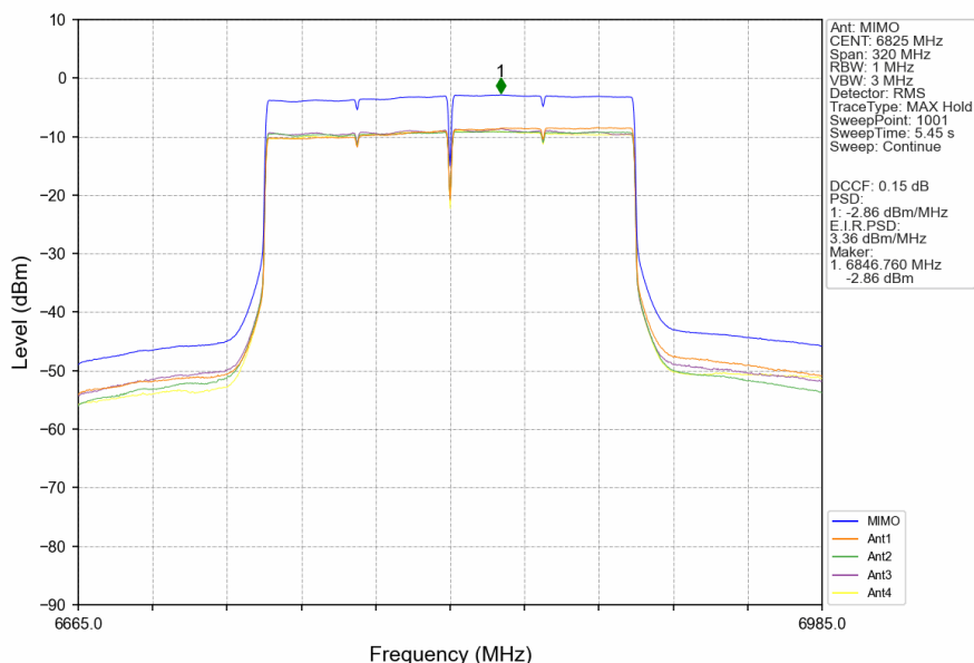
802.11ax(HEW160)_HCH_6825MHz_2xRU996_Left_MIMO_NTNV
