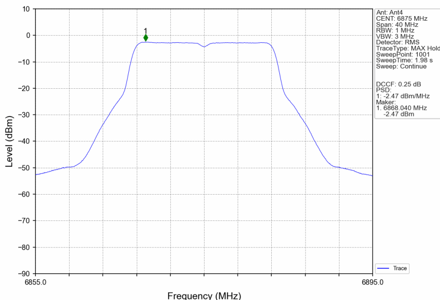
802.11a_HCH_6875MHz_Ant4_NTNV
