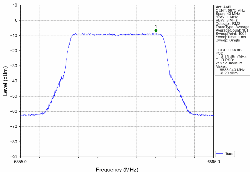
802.11ax(HEW20)_HCH_6875MHz_RU242_Left_Ant2_NTNV
