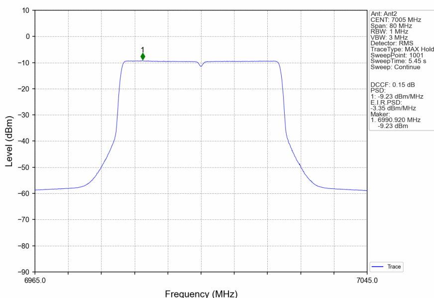
802.11ax(HEW40)_MCH_7005MHz_RU484_Left_Ant2_NTNV
