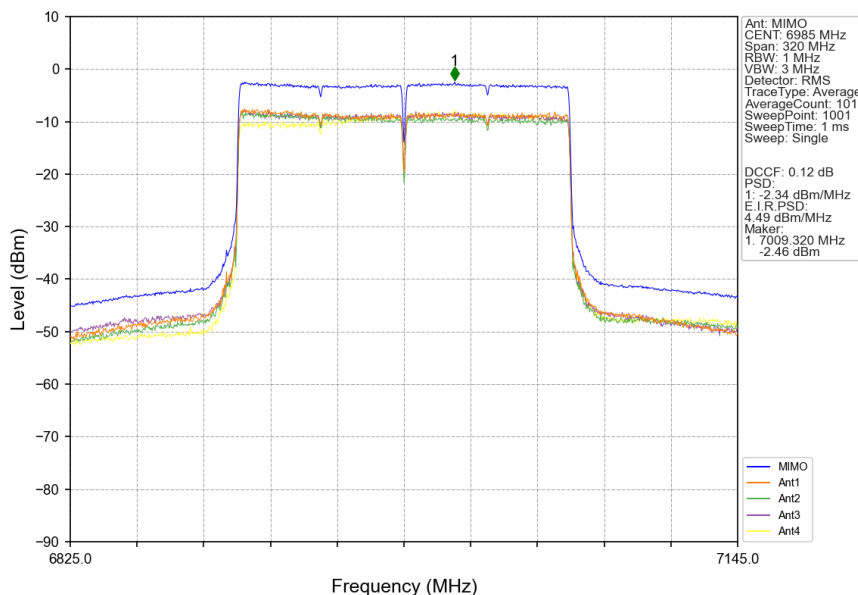
802.11ax(HEW160)_MCH_6985MHz_2xRU996_Left_MIMO_NTNV
