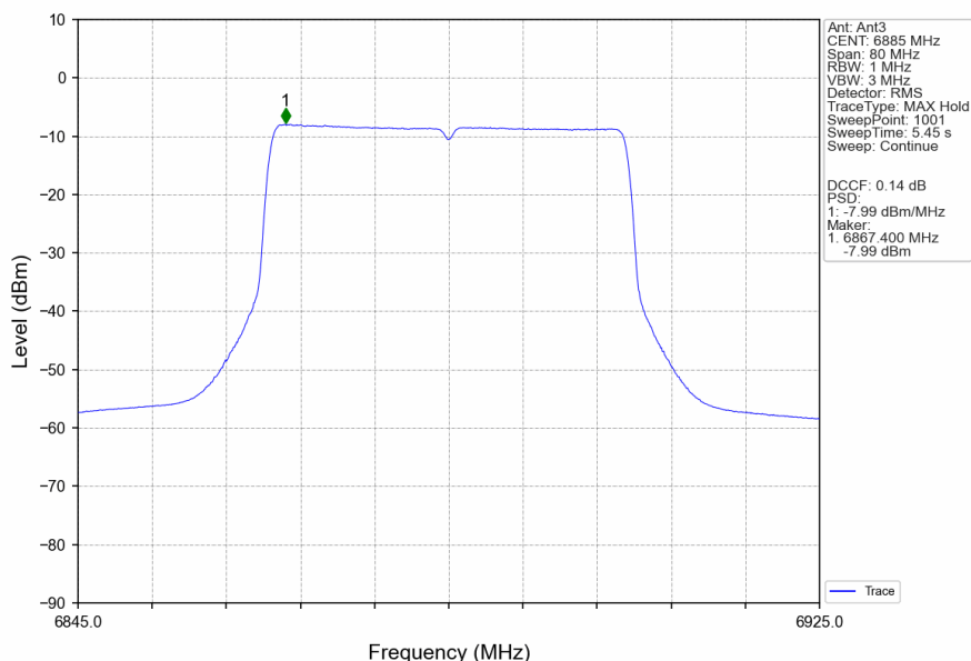
802.11ax(HEW40)_HCH_6885MHz_RU484_Left_Ant3_NTNV
