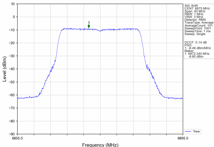
802.11ax(HEW20)_HCH_6875MHz_RU242_Left_Ant4_NTNV
