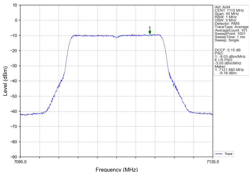
802.11ax(HEW20)_HCH_7115MHz_RU242_Left_Ant4_NTNV
