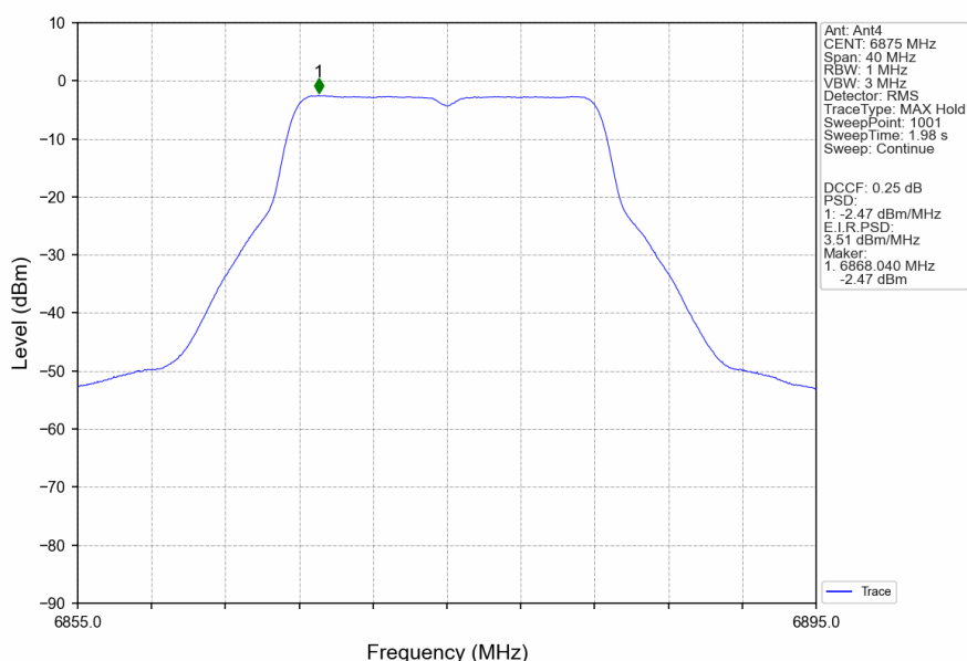
802.11a_HCH_6875MHz_Ant4_NTNV
