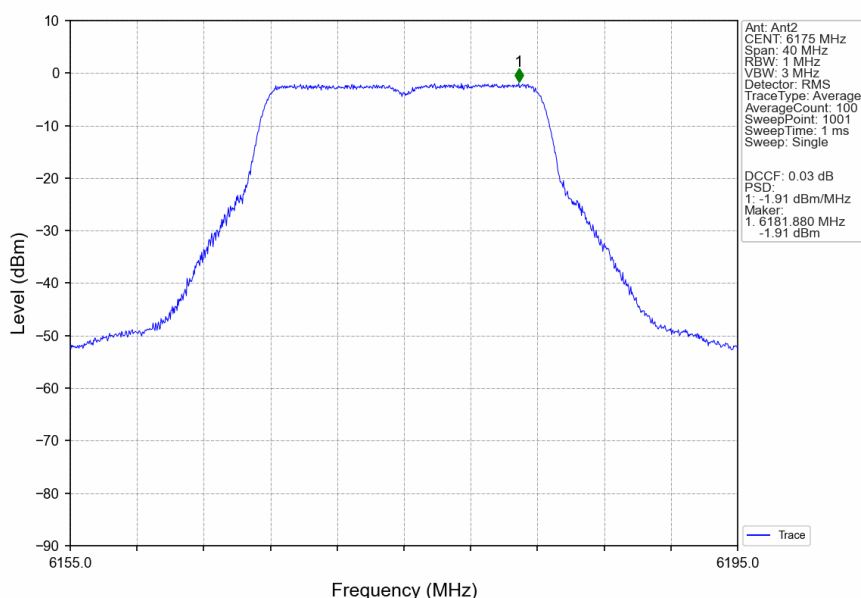
802.11a_MCH_6175MHz_Ant2_NTNV
