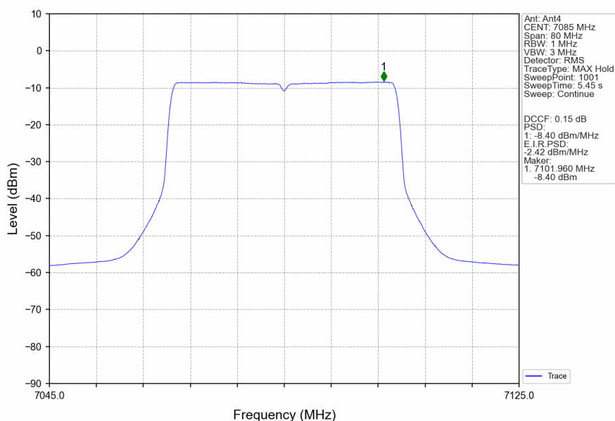
802.11ax(HEW40)_HCH_7085MHz_RU484_Left_MIMO_NTNV
