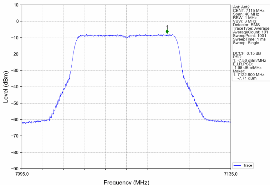
802.11ax(HEW20)_HCH_7115MHz_RU242_Left_Ant2_NTNV
