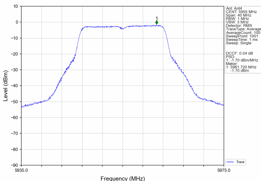
802.11a_LCH_5955MHz_Ant4_NTNV
