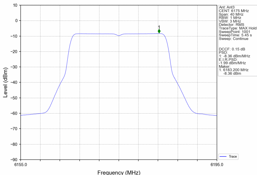
802.11ax(HEW20)_MCH_6175MHz_RU242_Left_Ant3_NTNV
