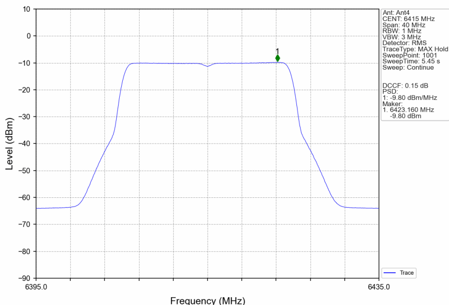
802.11ax(HEW20)_HCH_6415MHz_RU242_Left_Ant4_NTNV
