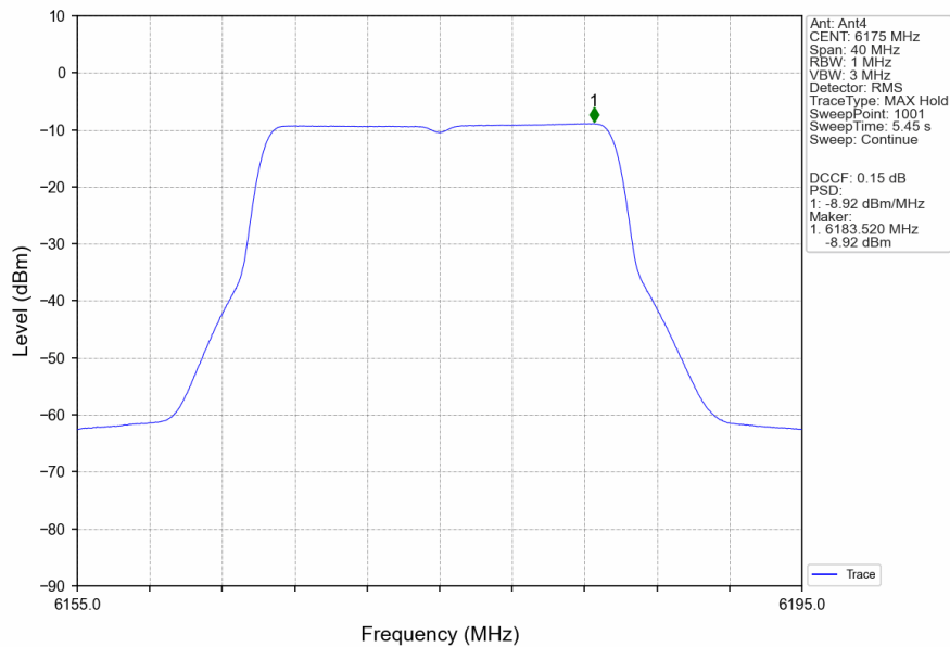
802.11ax(HEW20)_MCH_6175MHz_RU242_Left_MIMO_NTNV
