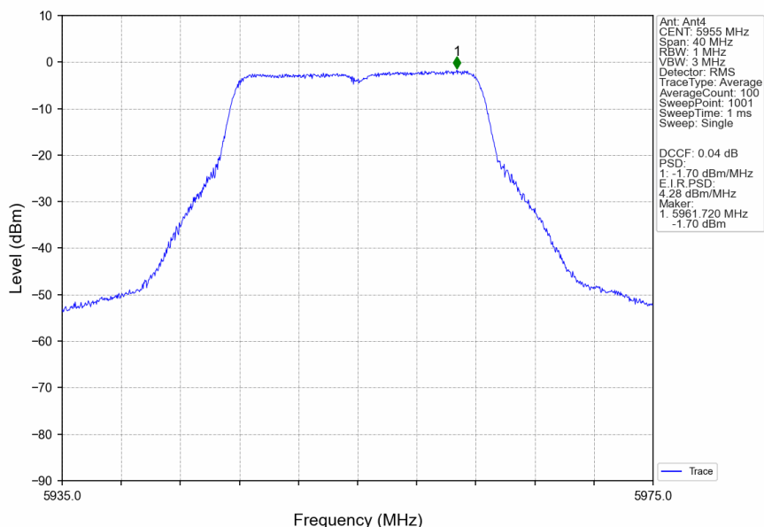
802.11a_LCH_5955MHz_Ant4_NTNV
