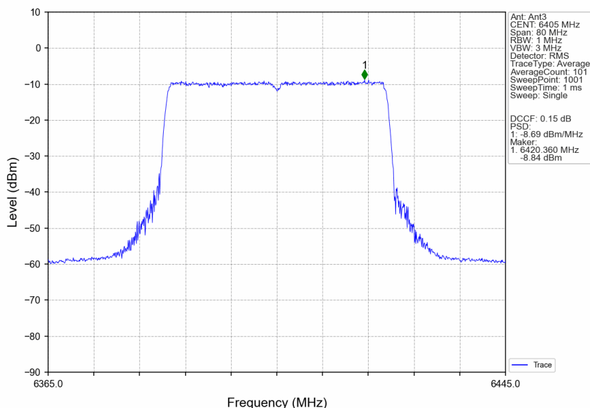
802.11ax(HEW40)_HCH_6405MHz_RU484_Left_Ant3_NTNV
