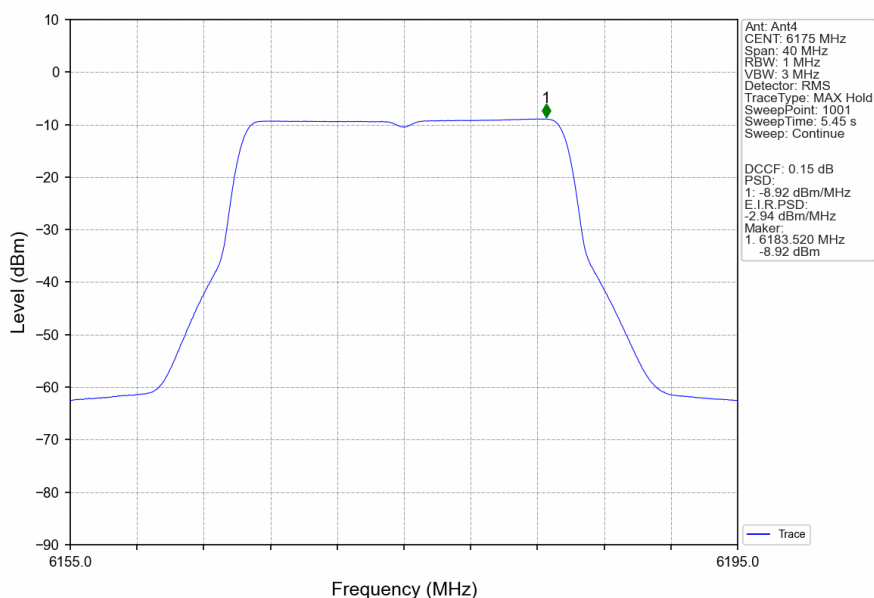
802.11ax(HEW20)_MCH_6175MHz_RU242_Left_MIMO_NTNV
