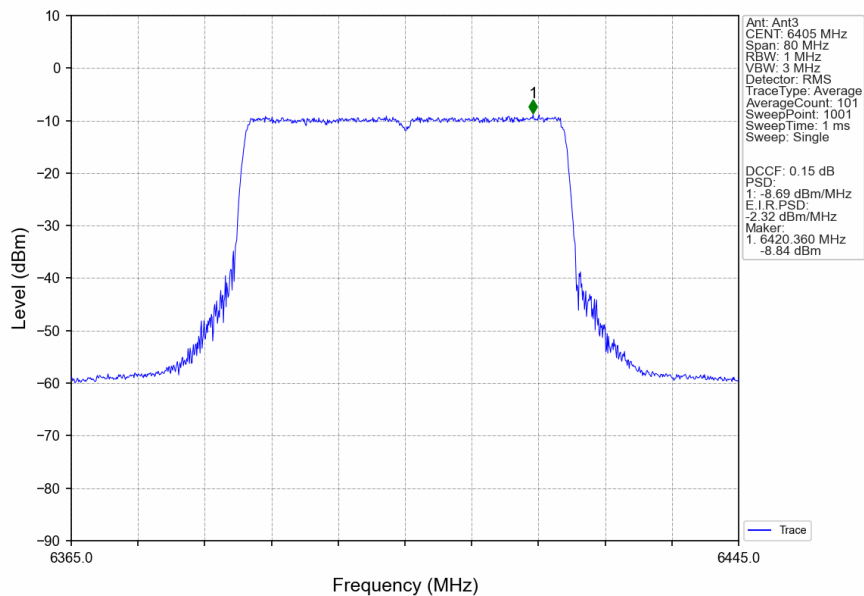
802.11ax(HEW40)_HCH_6405MHz_RU484_Left_Ant3_NTNV
