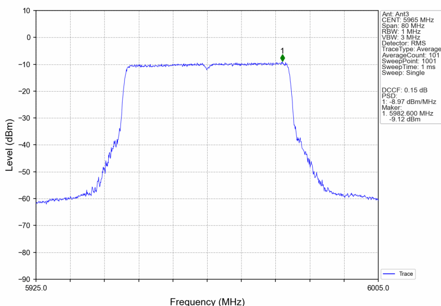
802.11ax(HEW40)_LCH_5965MHz_RU484_Left_Ant3_NTNV
