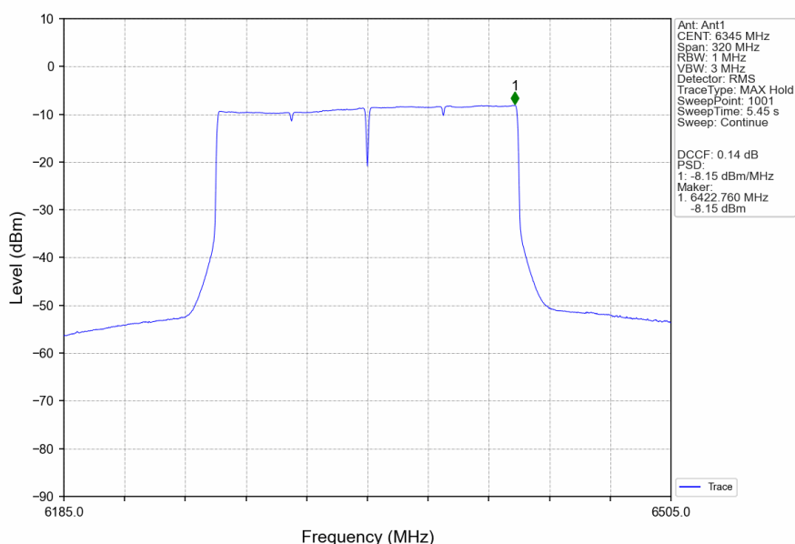
802.11ax(HEW160)_HCH_6345MHz_2xRU996_Left_Ant1_NTNV
