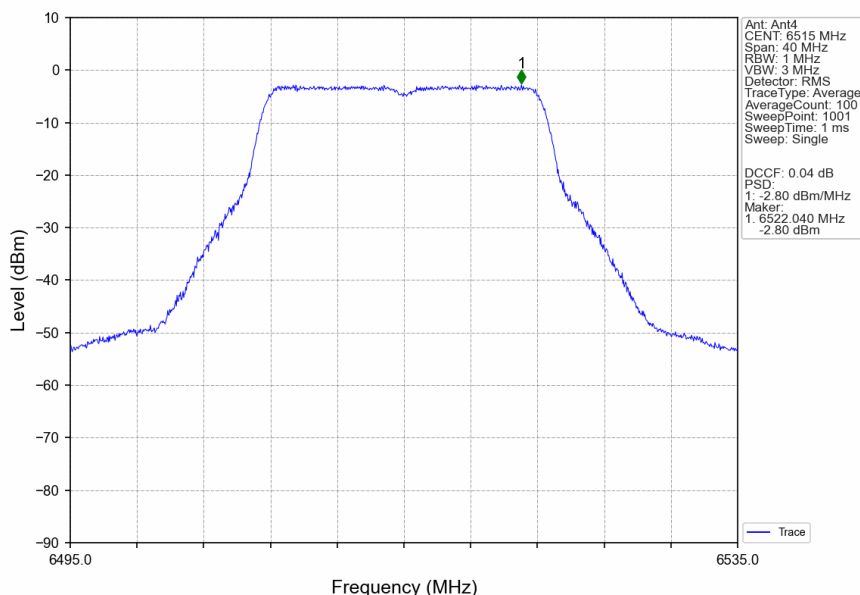
802.11a_HCH_6515MHz_Ant4_NTNV
