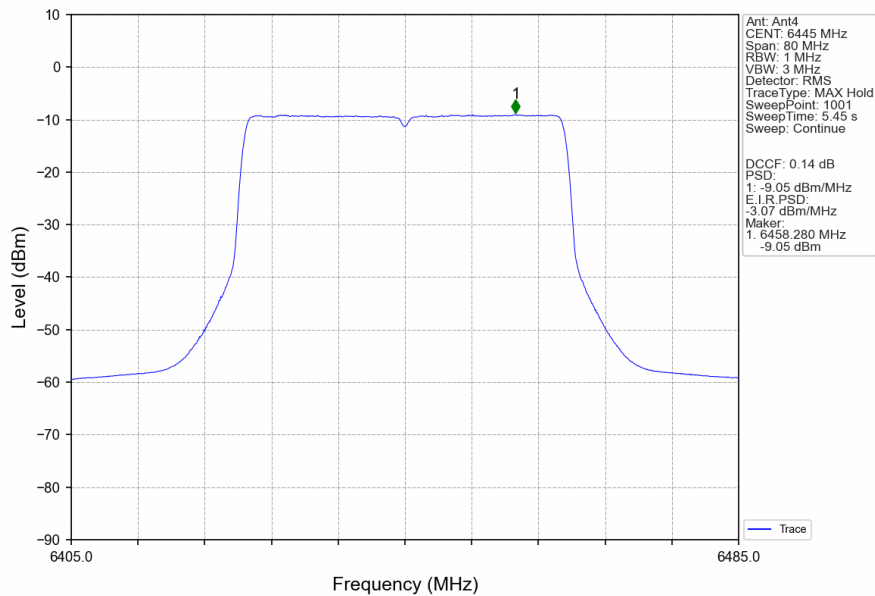
802.11ax(HEW40)_LCH_6445MHz_RU484_Left_MIMO_NTNV
