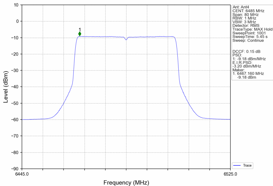
802.11ax(HEW40)_MCH_6485MHz_RU484_Left_Ant4_NTNV
