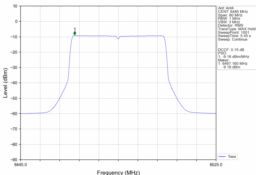
802.11ax(HEW40)_MCH_6485MHz_RU484_Left_Ant4_NTNV
