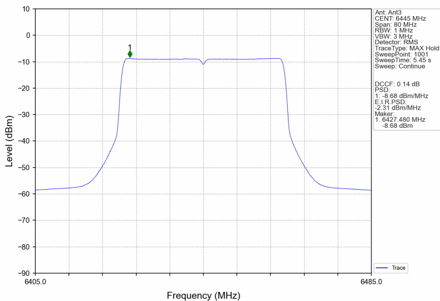
802.11ax(HEW40)_LCH_6445MHz_RU484_Left_Ant3_NTNV
