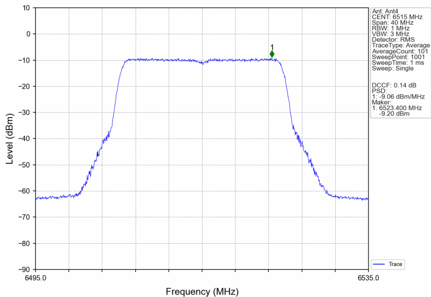
802.11ax(HEW20)_HCH_6515MHz_RU242_Left_Ant4_NTNV
