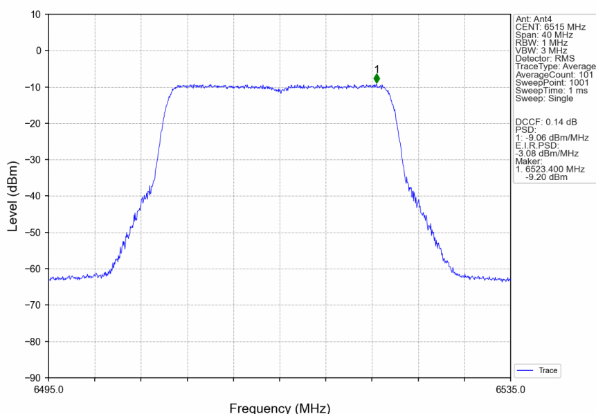
802.11ax(HEW20)_HCH_6515MHz_RU242_Left_Ant4_NTNV
