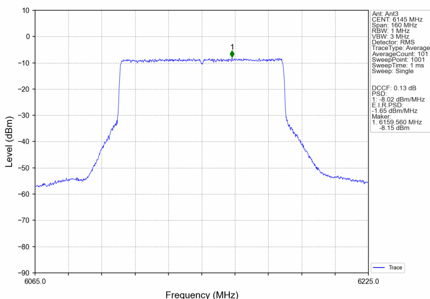
802.11ax(HEW80)_MCH_6145MHz_RU996_Left_Ant3_NTNV
