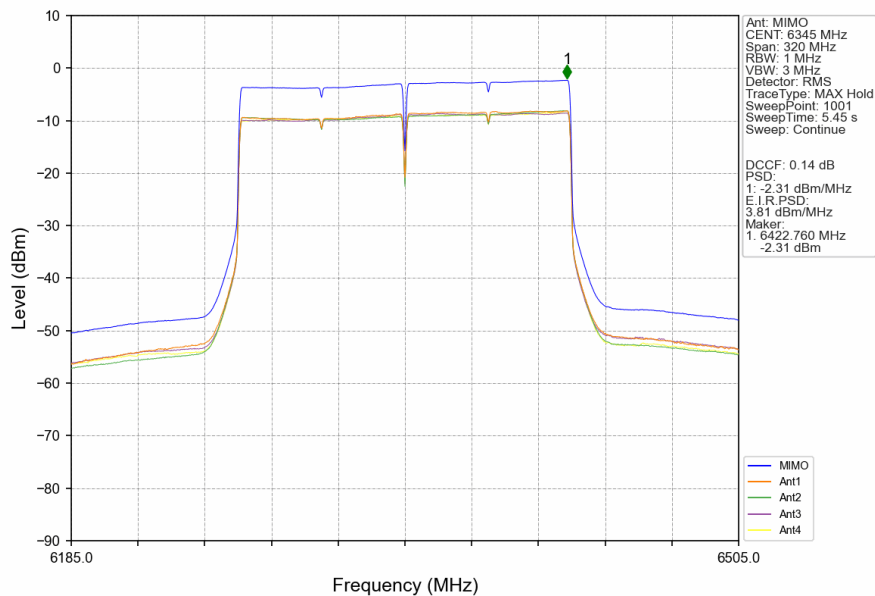
802.11ax(HEW160)_HCH_6345MHz_2xRU996_Left_MIMO_NTNV
