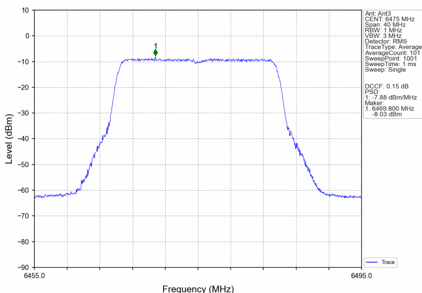
802.11ax(HEW20)_MCH_6475MHz_RU242_Left_Ant3_NTNV
