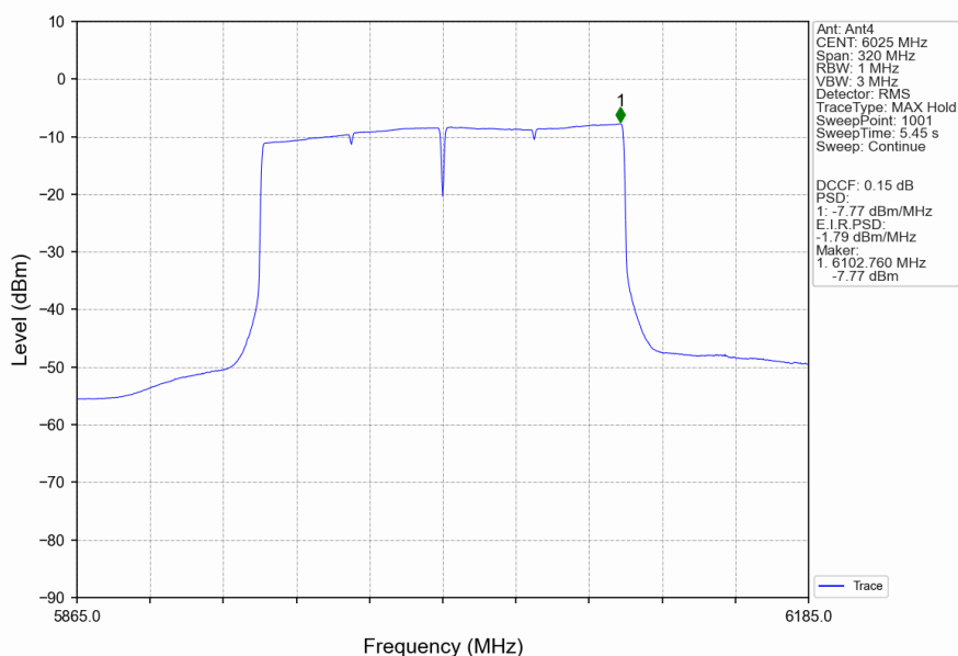
802.11ax(HEW160)_LCH_6025MHz_2xRU996_Left_MIMO_NTNV
