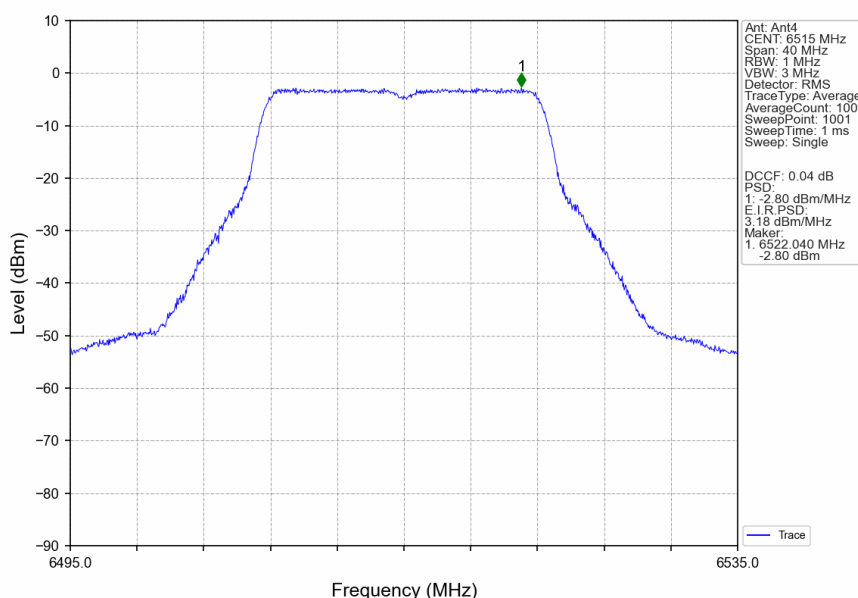
802.11a_HCH_6515MHz_Ant4_NTNV
