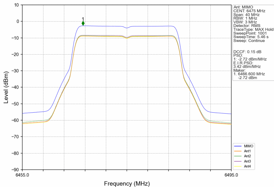
802.11be(EHT20)_MCH_6475MHz_RU242_Left_MIMO_NTNV
